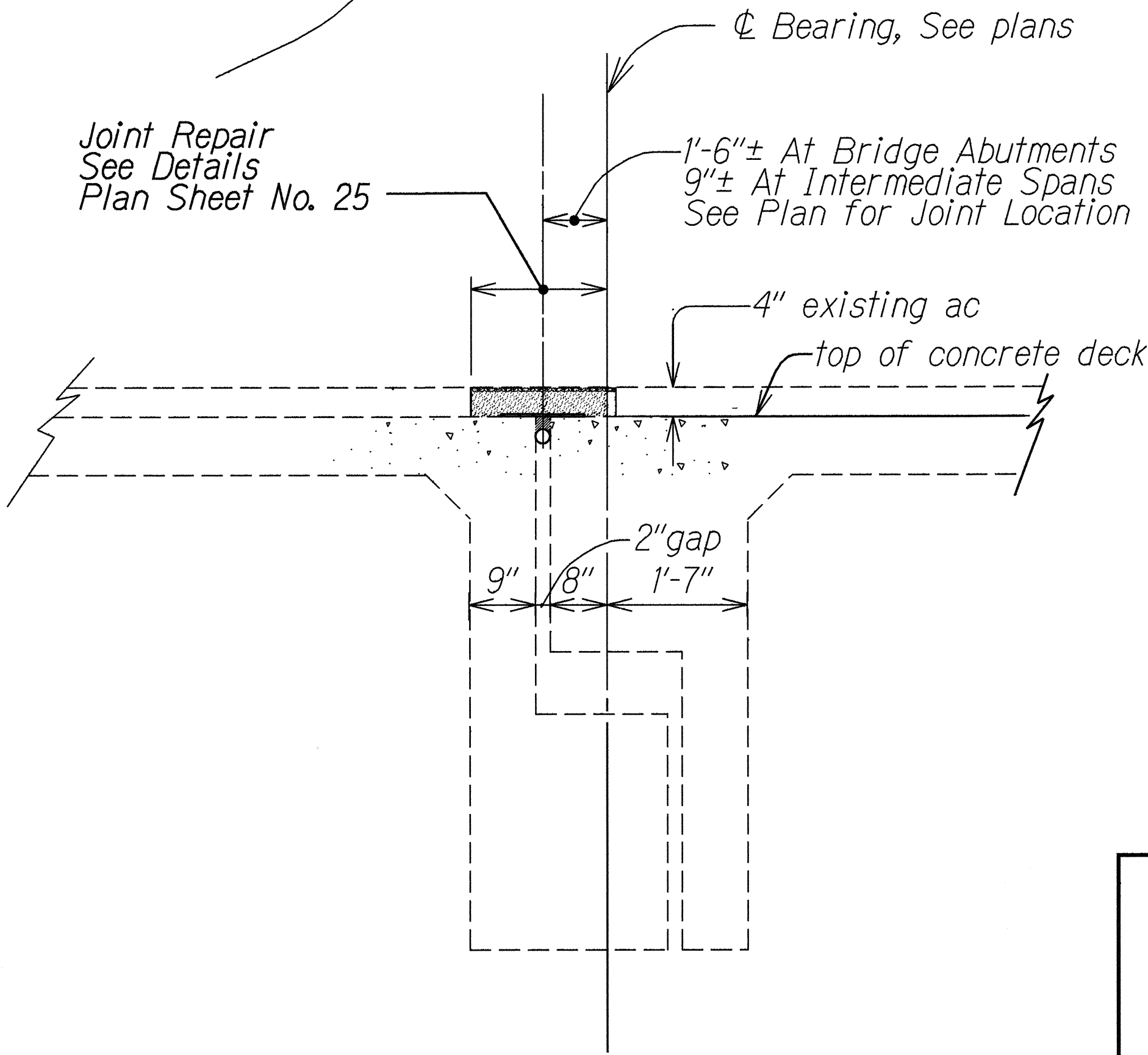
TYPICAL BRIDGE JOINT Scale: 3/4"= 1'-0"
