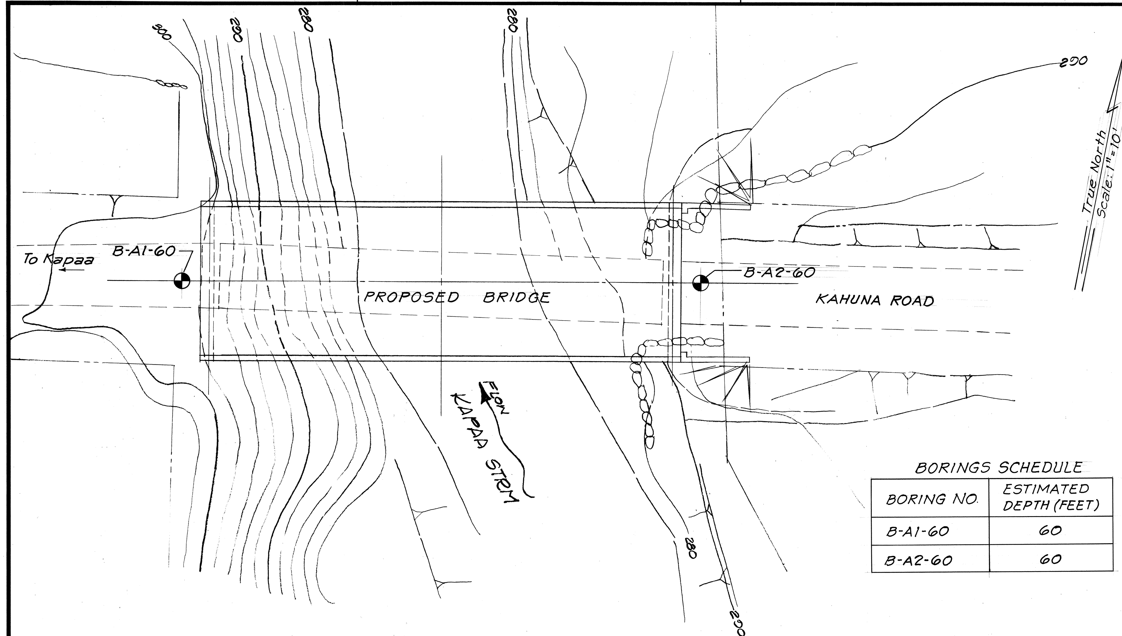
LAYOUT PLAN Scale: 1"=10'-0"
