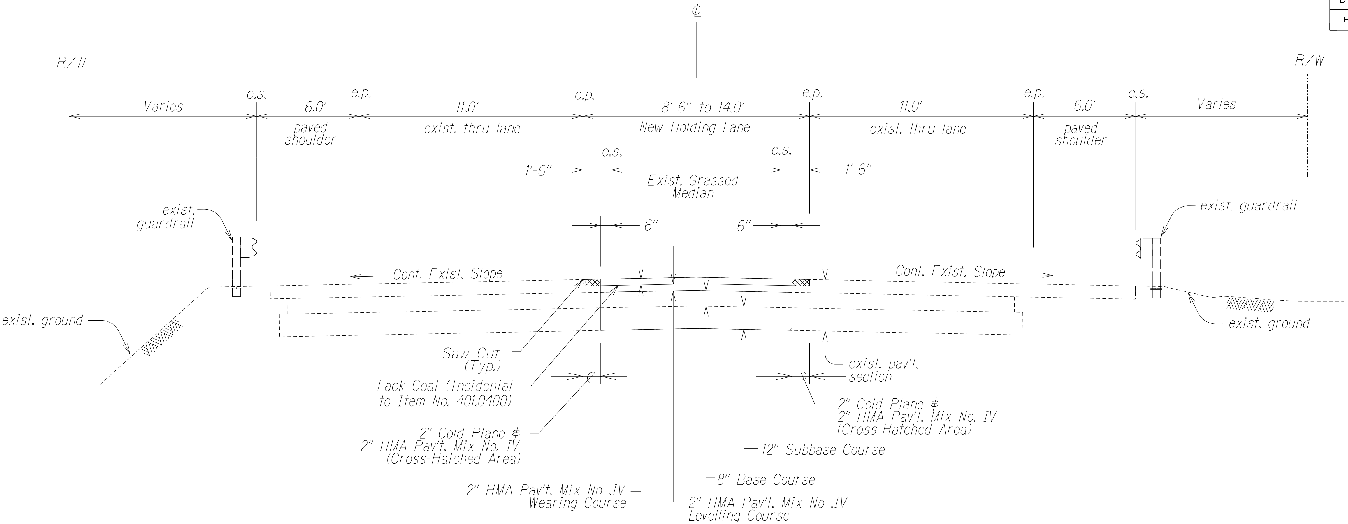
CROSS SECTION Not to Scale
