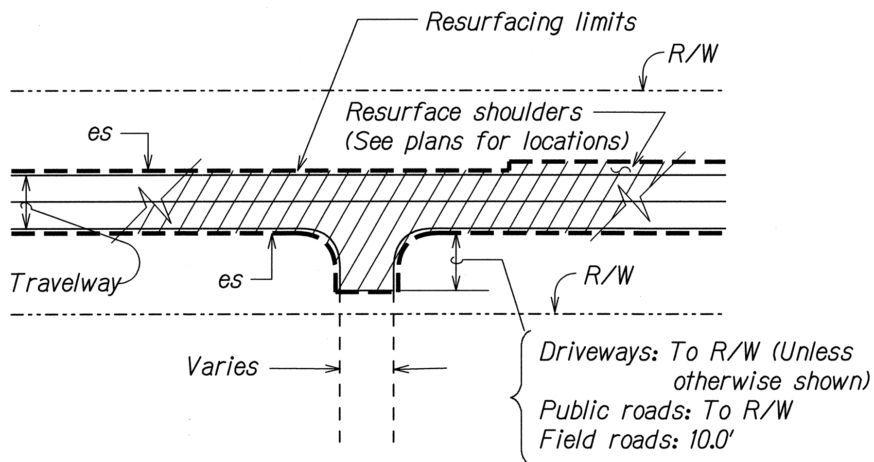
PLAN - TYPICAL RESURFACING LIMITS Not To Scale
