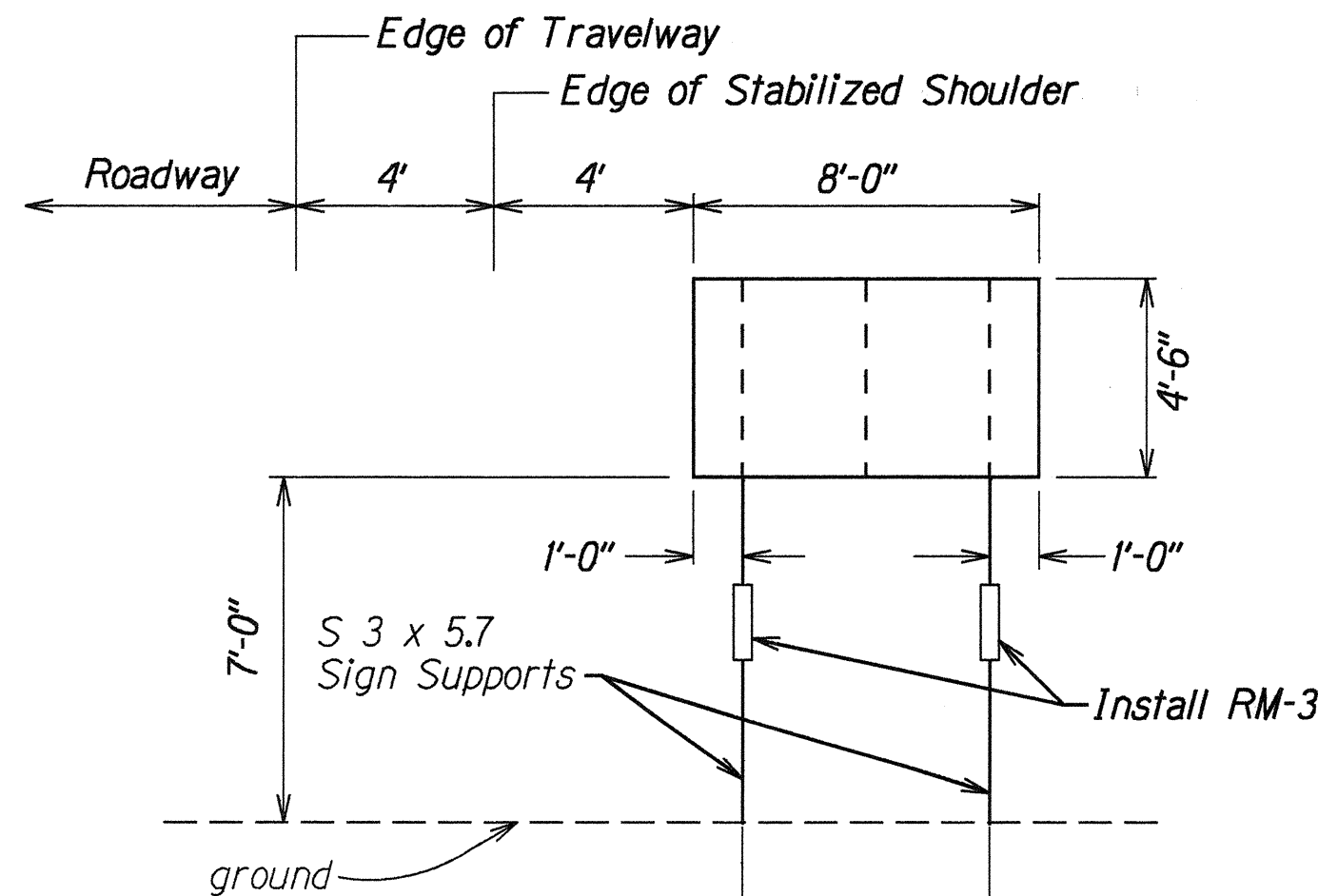
D1-2 - DETAIL FRAME LAYOUT Not To Scale
