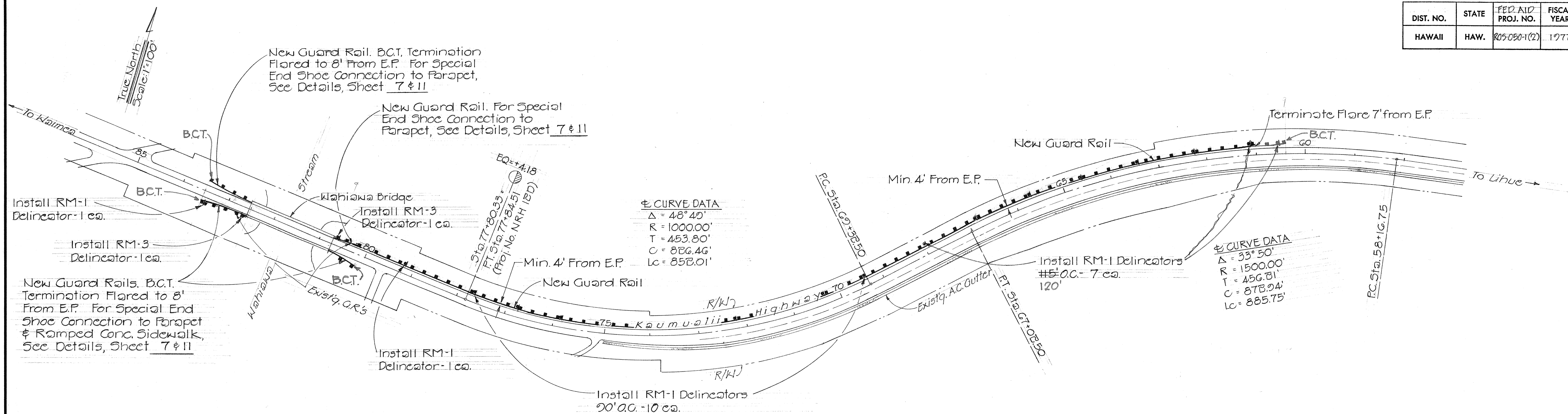
VICINITY ~ WAHIAWA BRIDGE & TRUCK CLIMBING LANES
