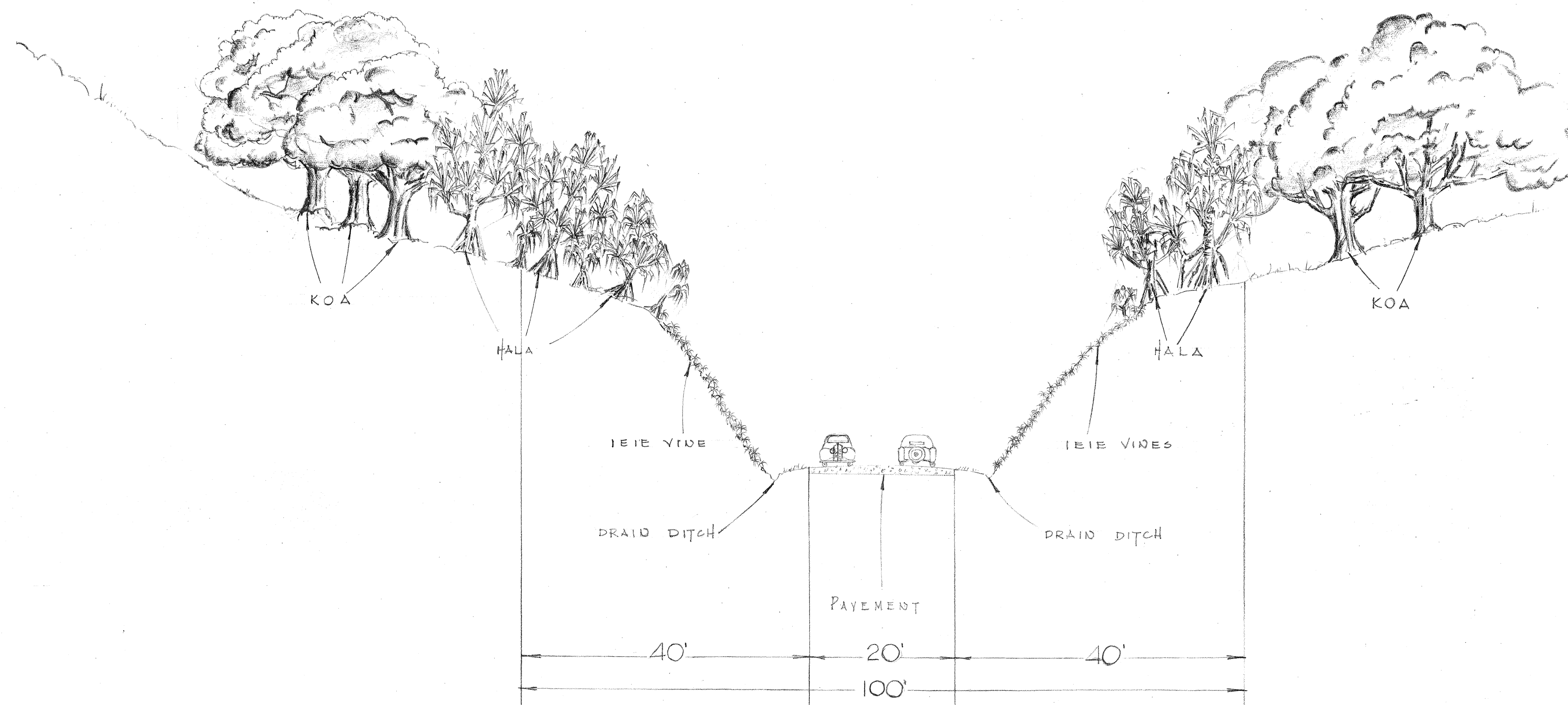
CROSS SECTION OF TYPICAL PLANTING AT STATION 303 SCALE 1"=10'
