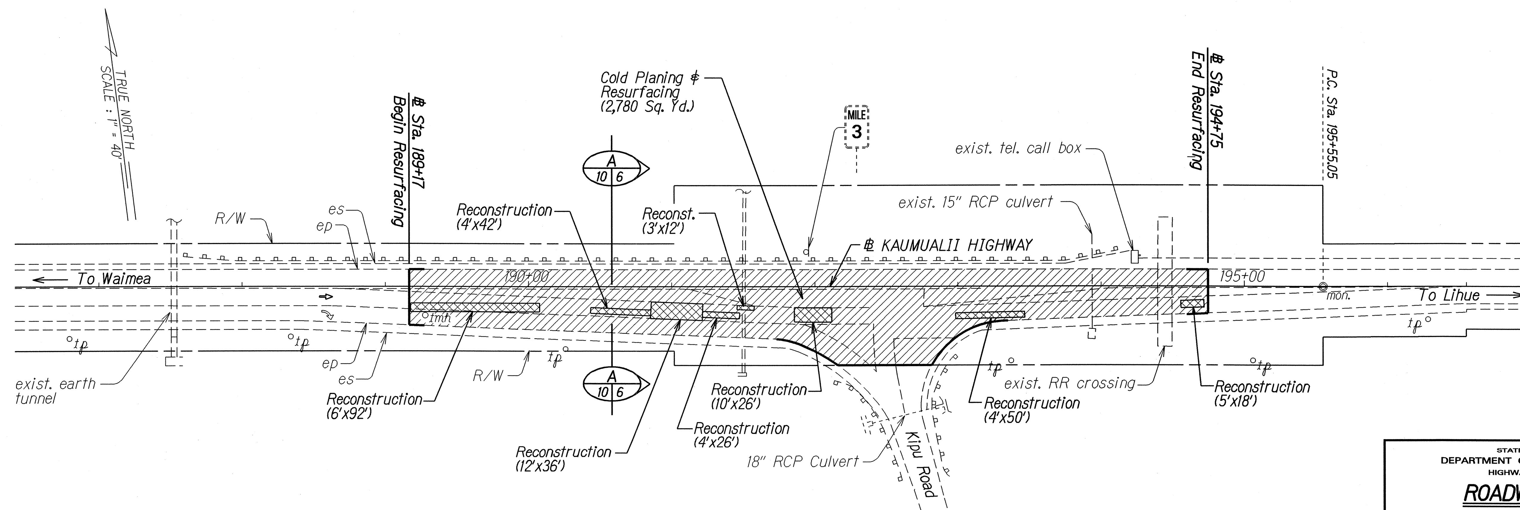
MAHINAULI BRIDGE AT M.P. 20.33
