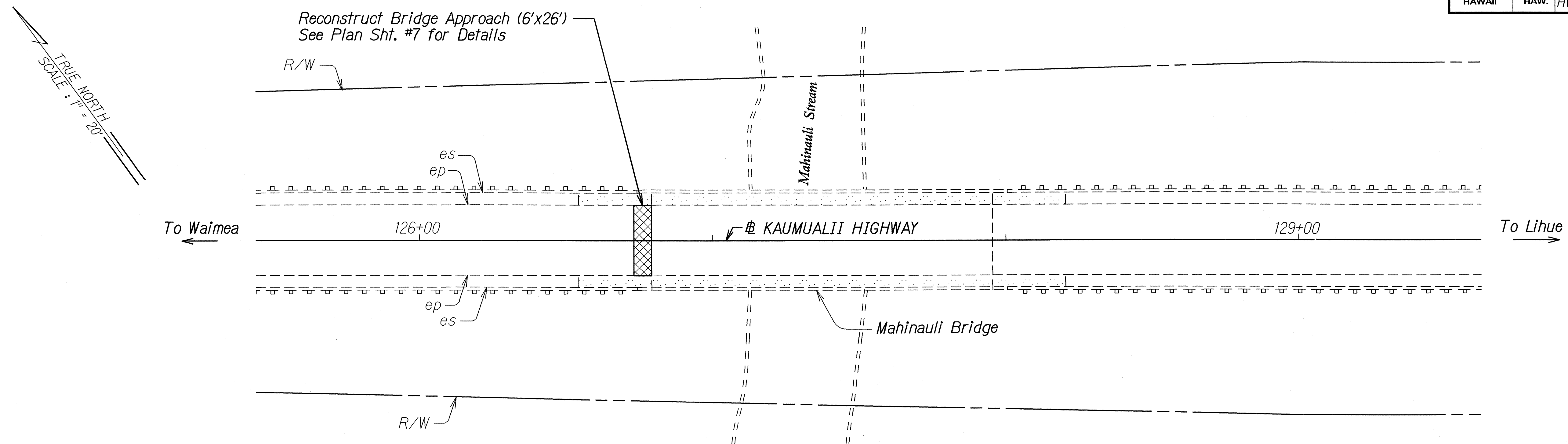
MAHINAULI BRIDGE AT M.P. 20.33
