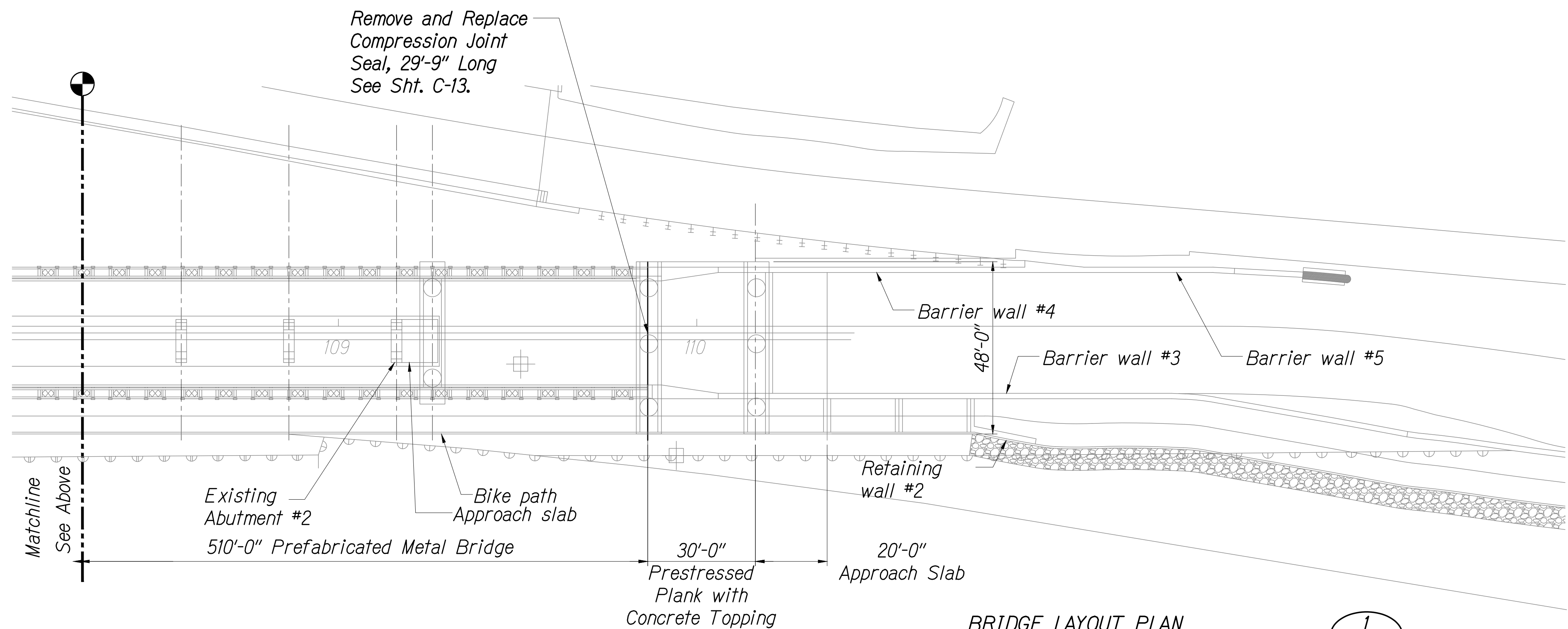
BRIDGE LAYOUT PLAN Scale: 1" = 20'-0"
