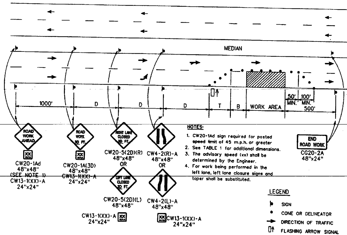
FIGURE 4 - TRAFFIC CONTROL PLAN
