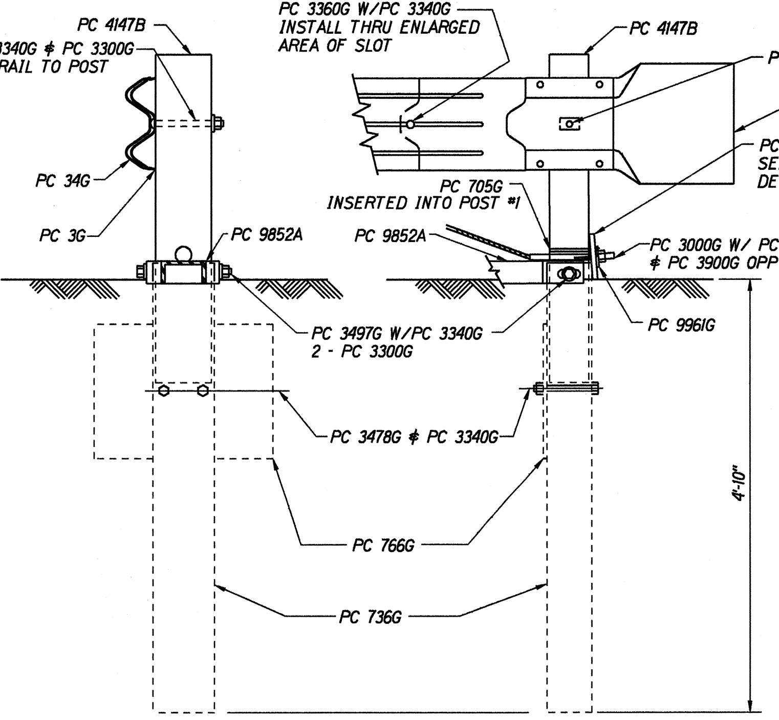
SECTION "A-A" (at POST #2) ENLARGED VIEW @ POST #1
