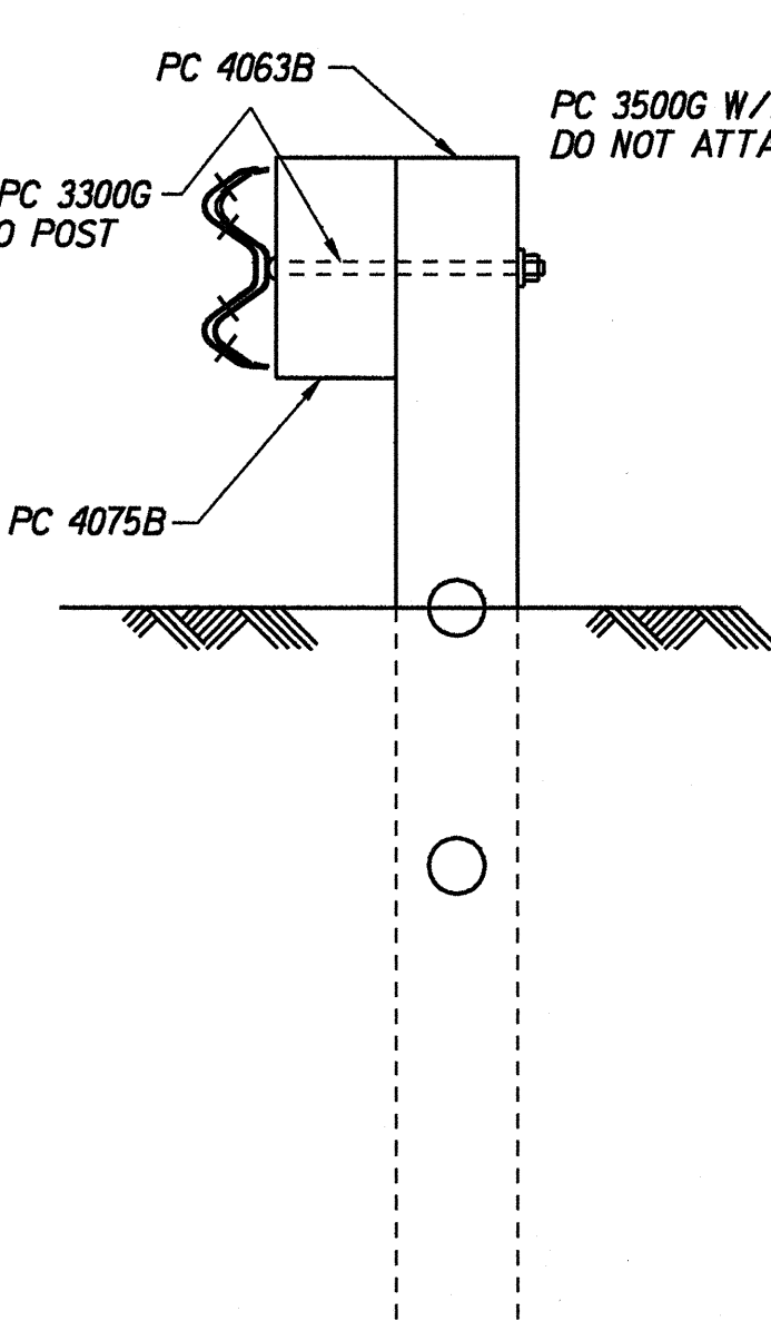
SECTION "B-B" (at POSTS #3 & #7)
