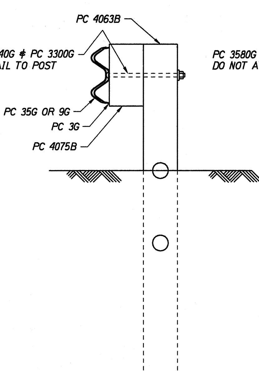
SECTION "C-C" (at POSTS #4, #6, #8, #9 & #10)
