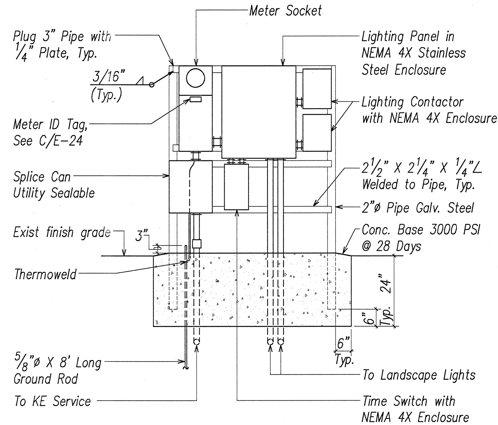
FRONT ELEVATION
