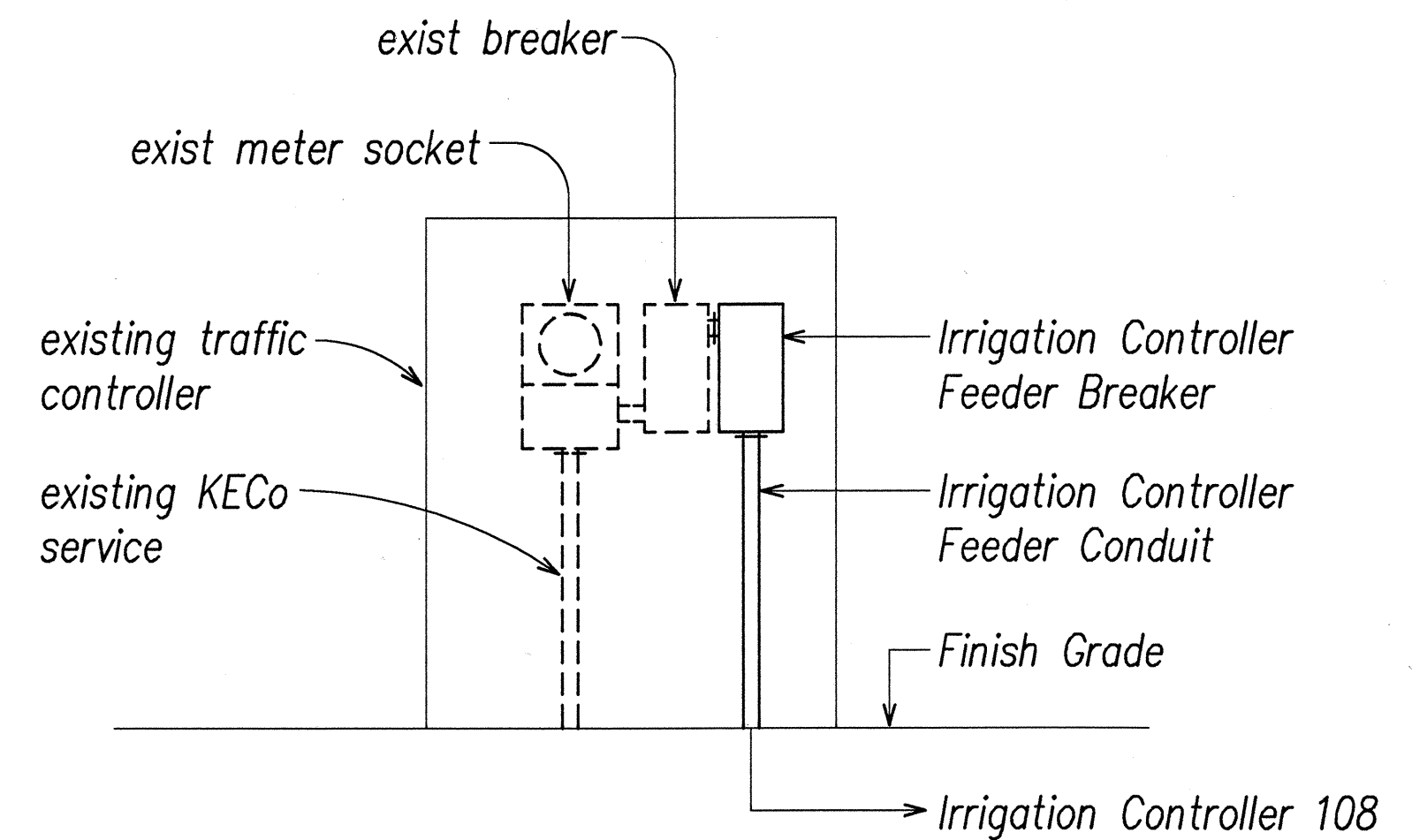
B EXIST TRAFFIC CONTROLLER ELEVATION E-24 Not to Scale
