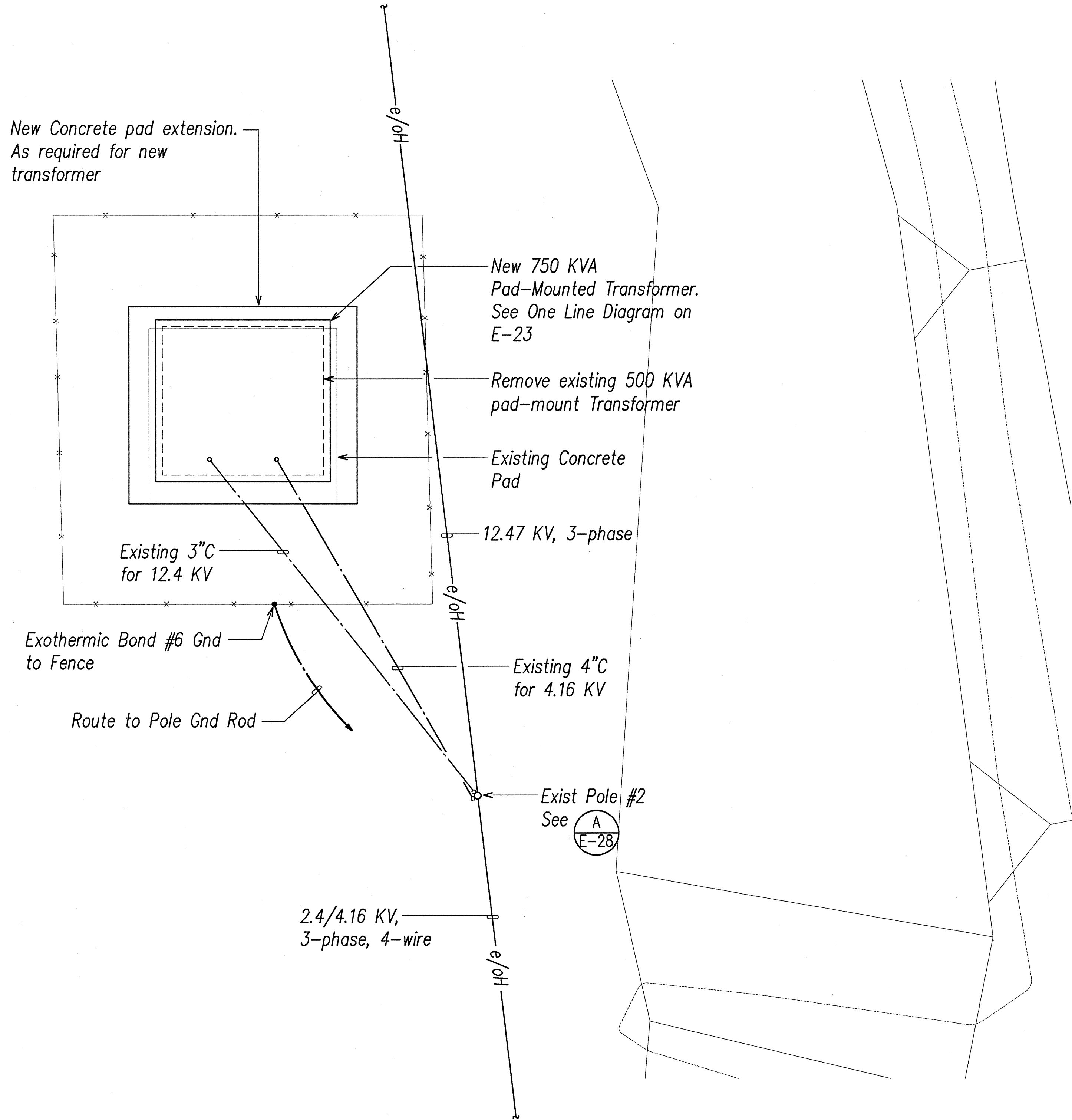
(A) TRANSFORMER FACILITY ELECTRICAL PLAN E-21 SCALE: 3/8"=1'-0"
