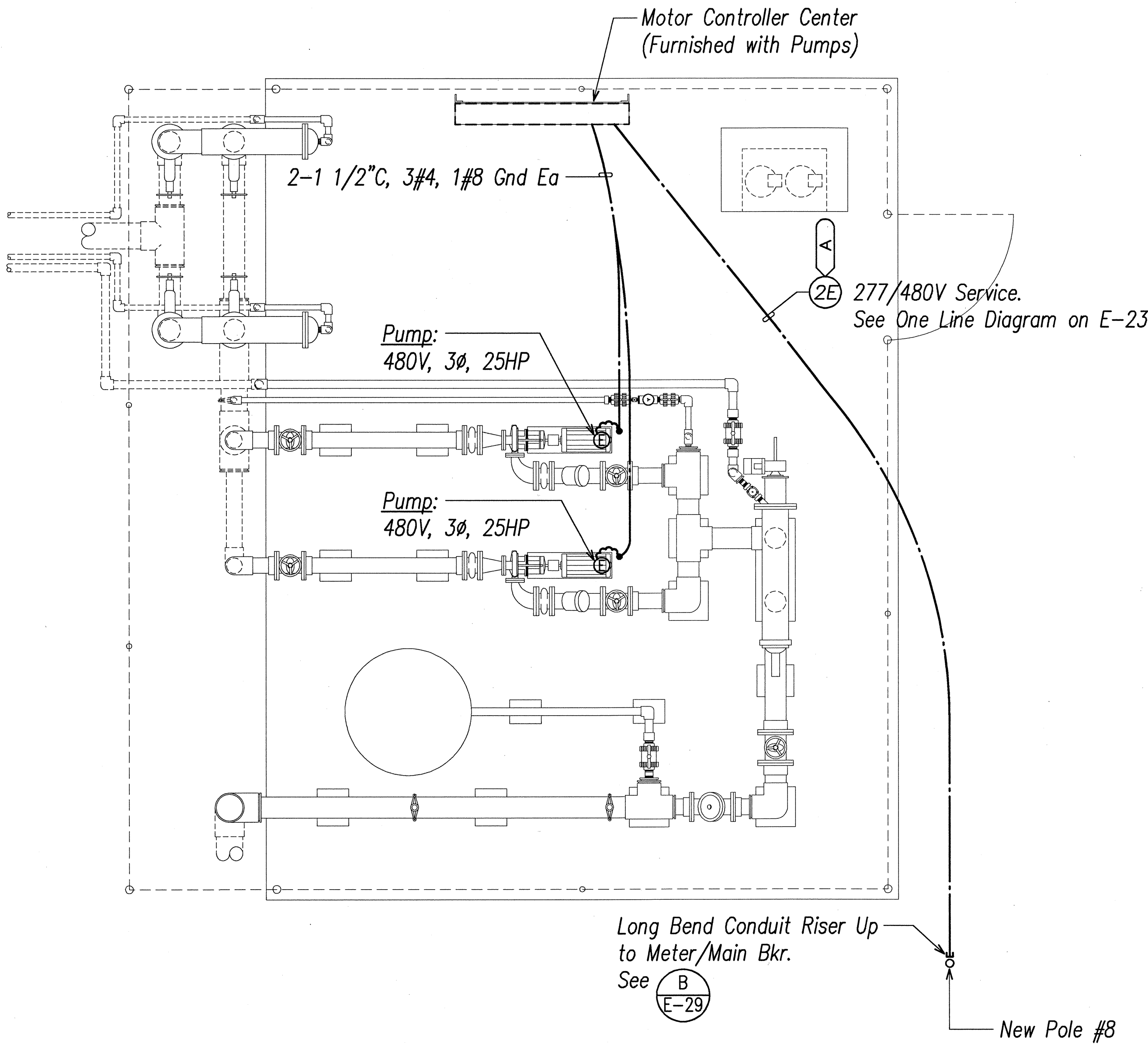
(B) PUMP FACILITY ELECTRICAL PLAN E-21 SCALE: 3/8"=1'-0"
