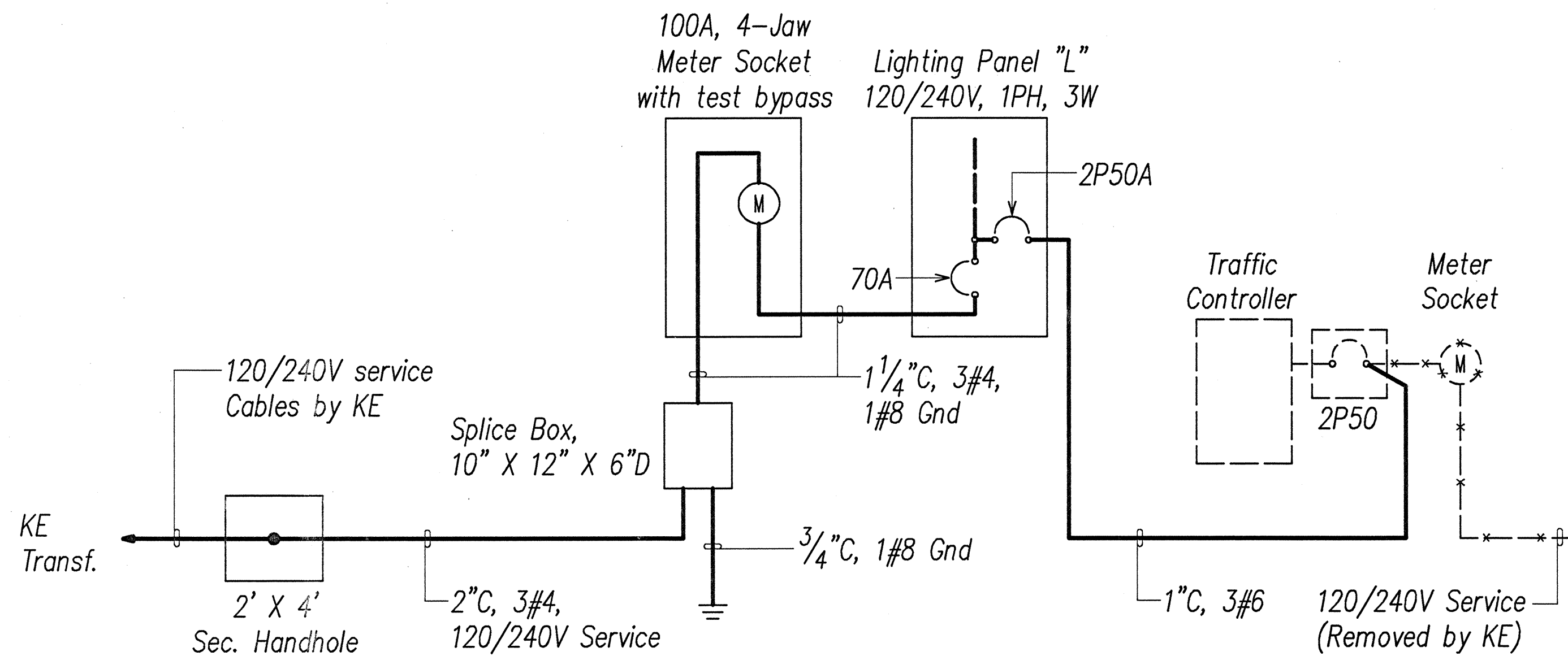
LANDSCAPE LIGHTING PANEL SERVICE DIAGRAM
