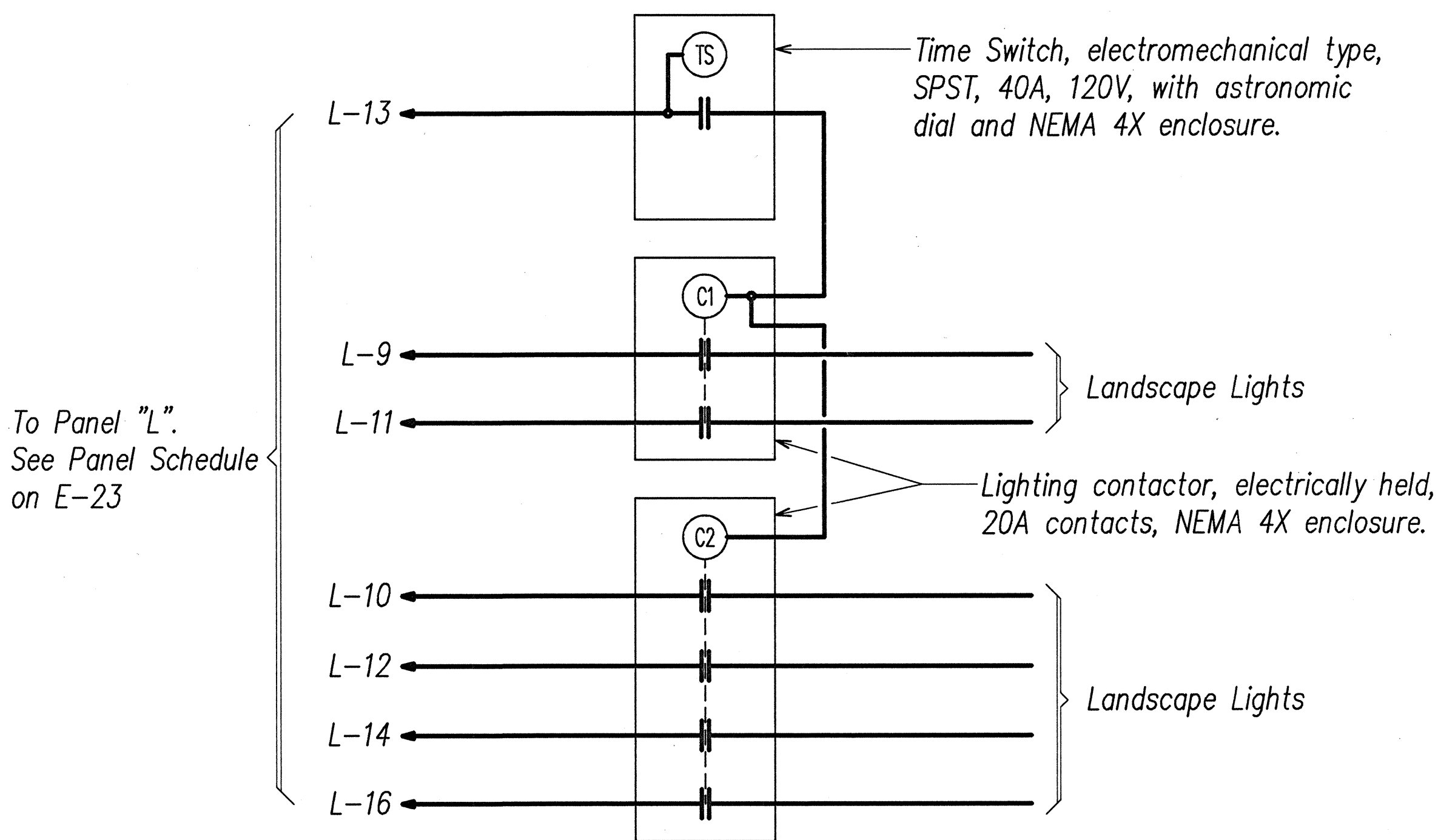
LIGHTS CONTROL DIAGRAM
