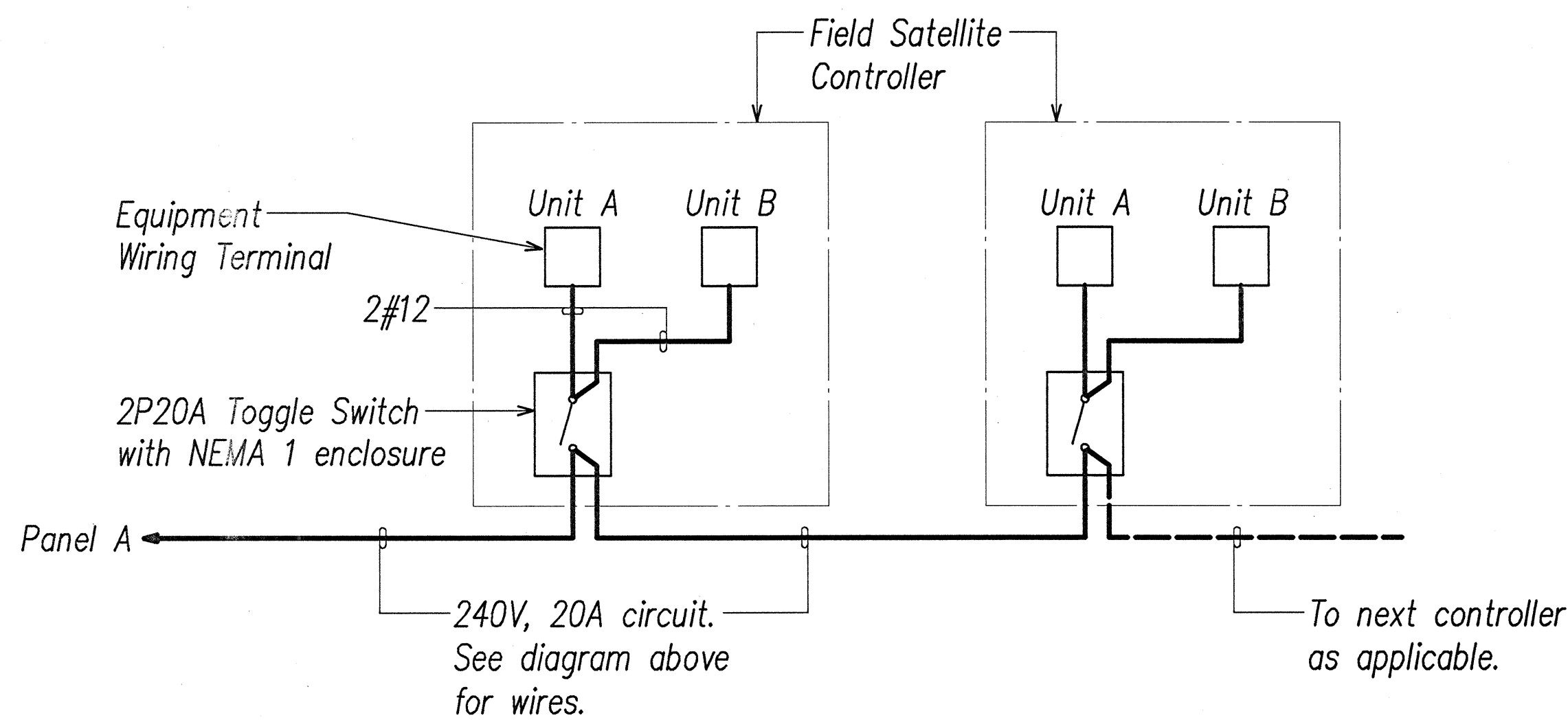
TYPICAL IRRIGATION CONTROLLER CIRCUIT DIAGRAM
