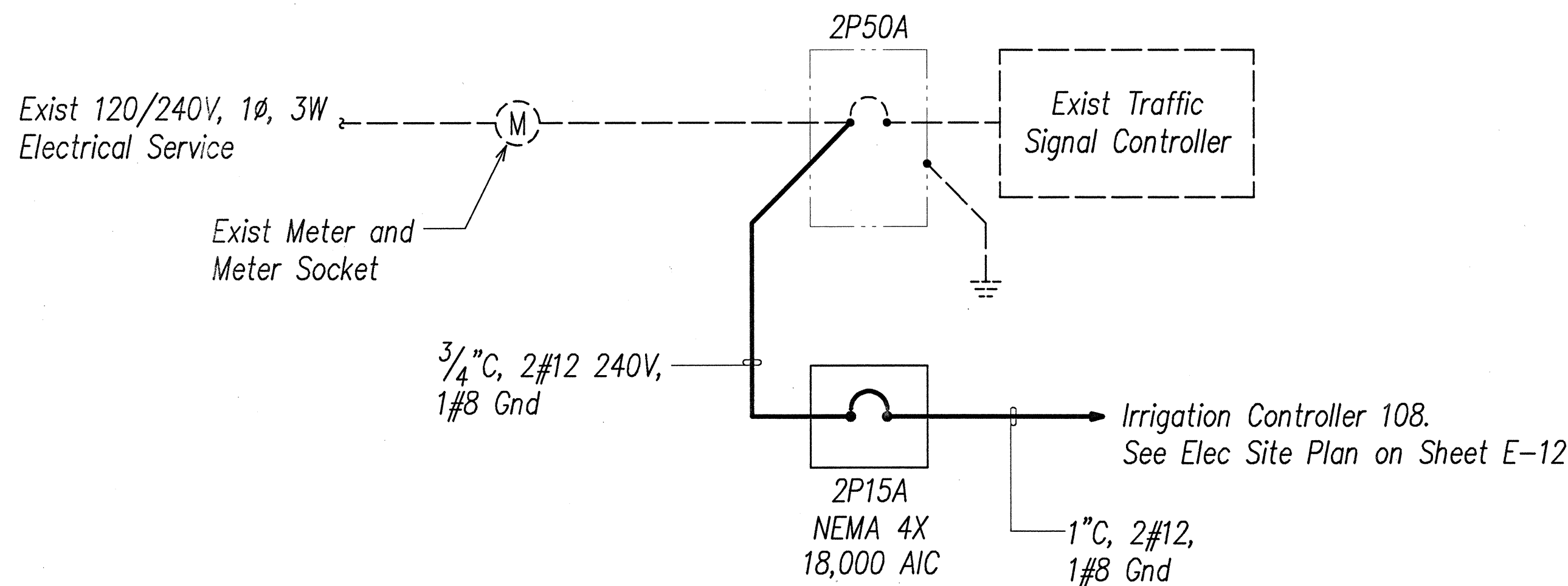
IRRIGATION CONTROLLER SERVICE DIAGRAM
