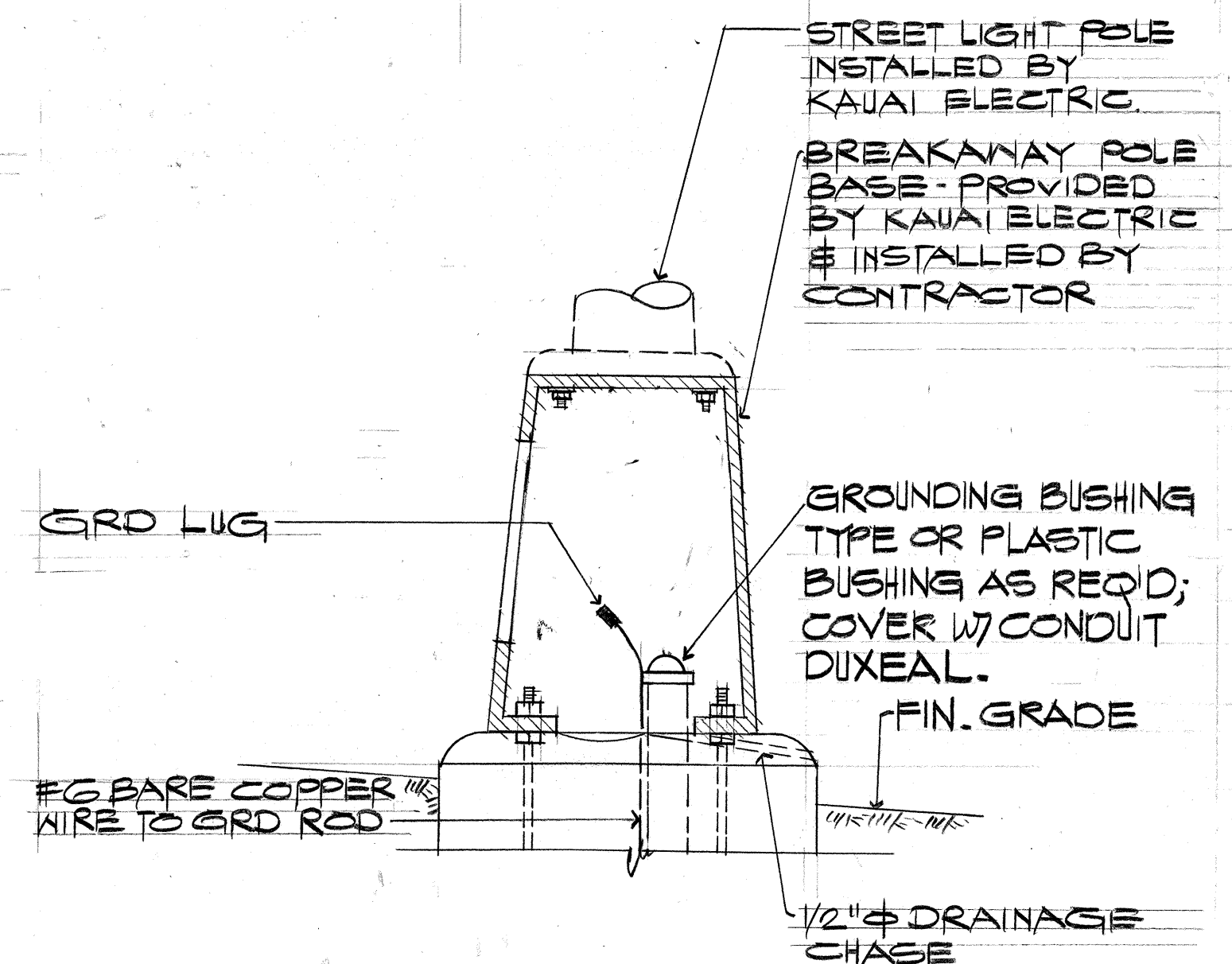
BASE DETAIL
