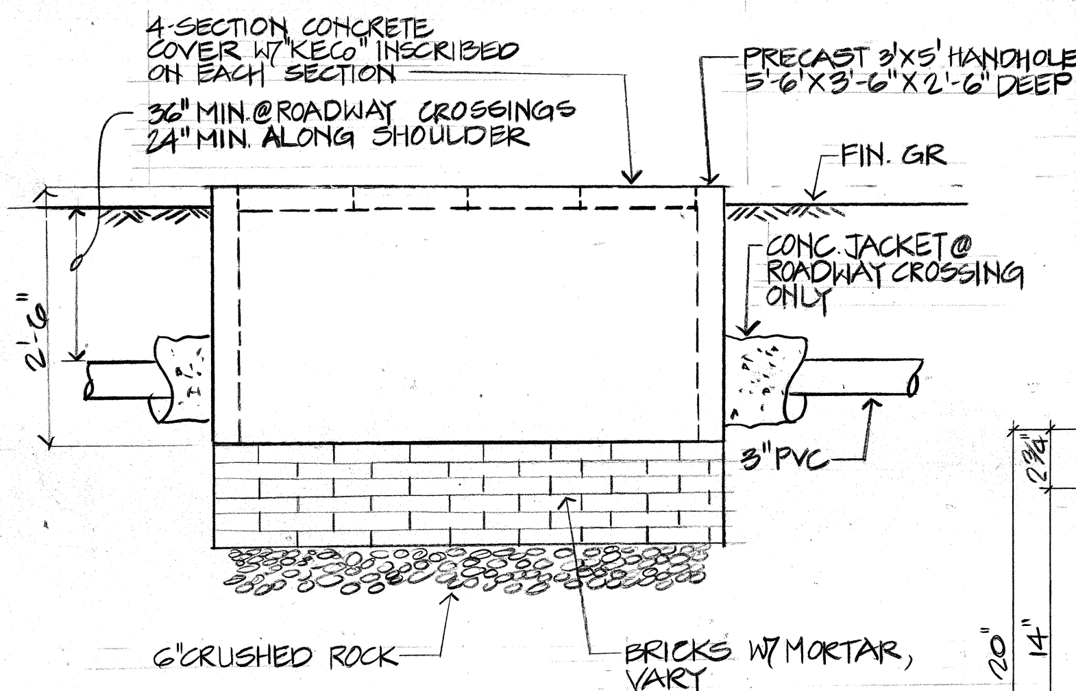
HANDHOLE DETAIL E-3
