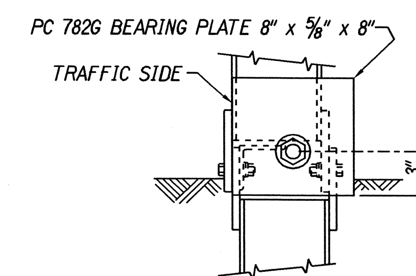
VIEW "K-K"
