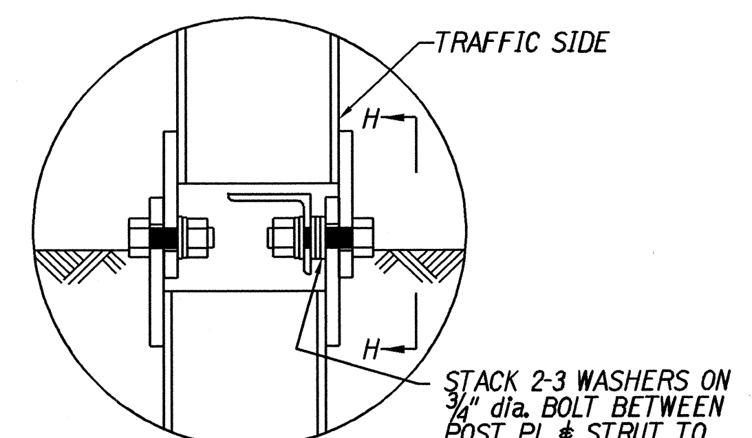
DETAIL "H" (POST #2)
