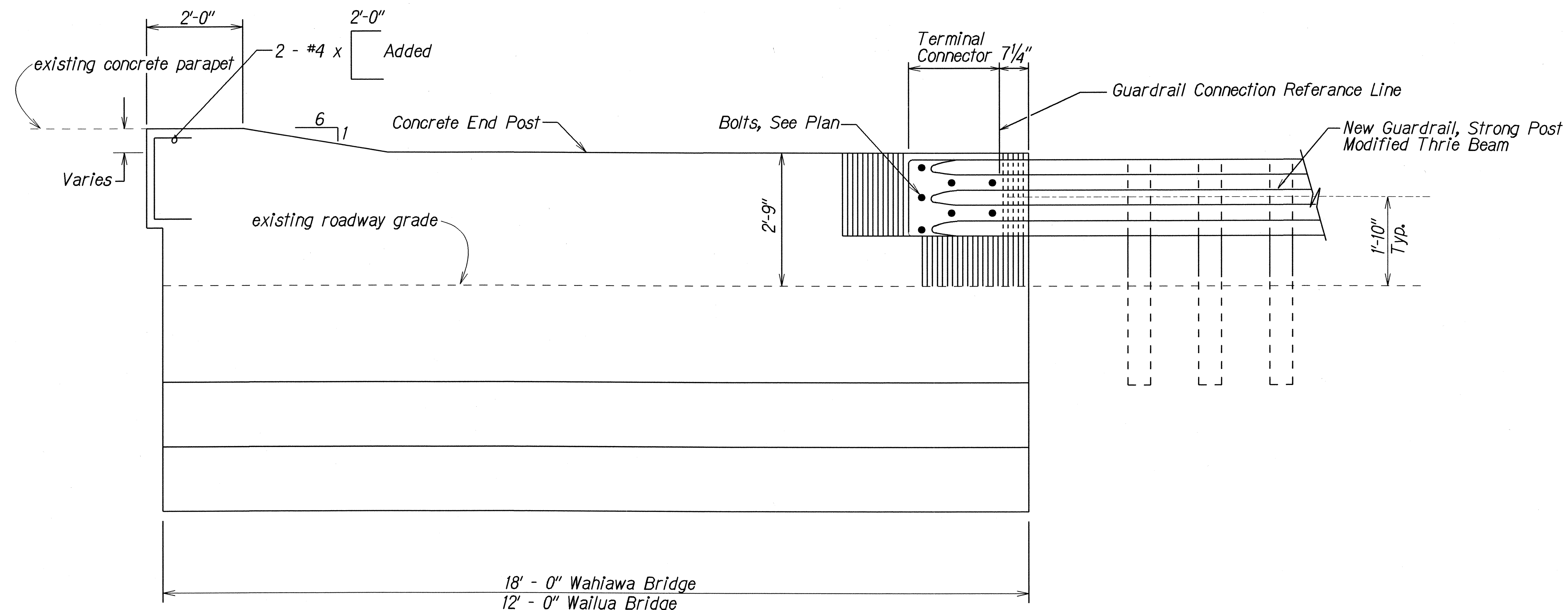
ELEVATION Scale: \frac{3}{4}" = 1'-0" CONCRETE END POST
