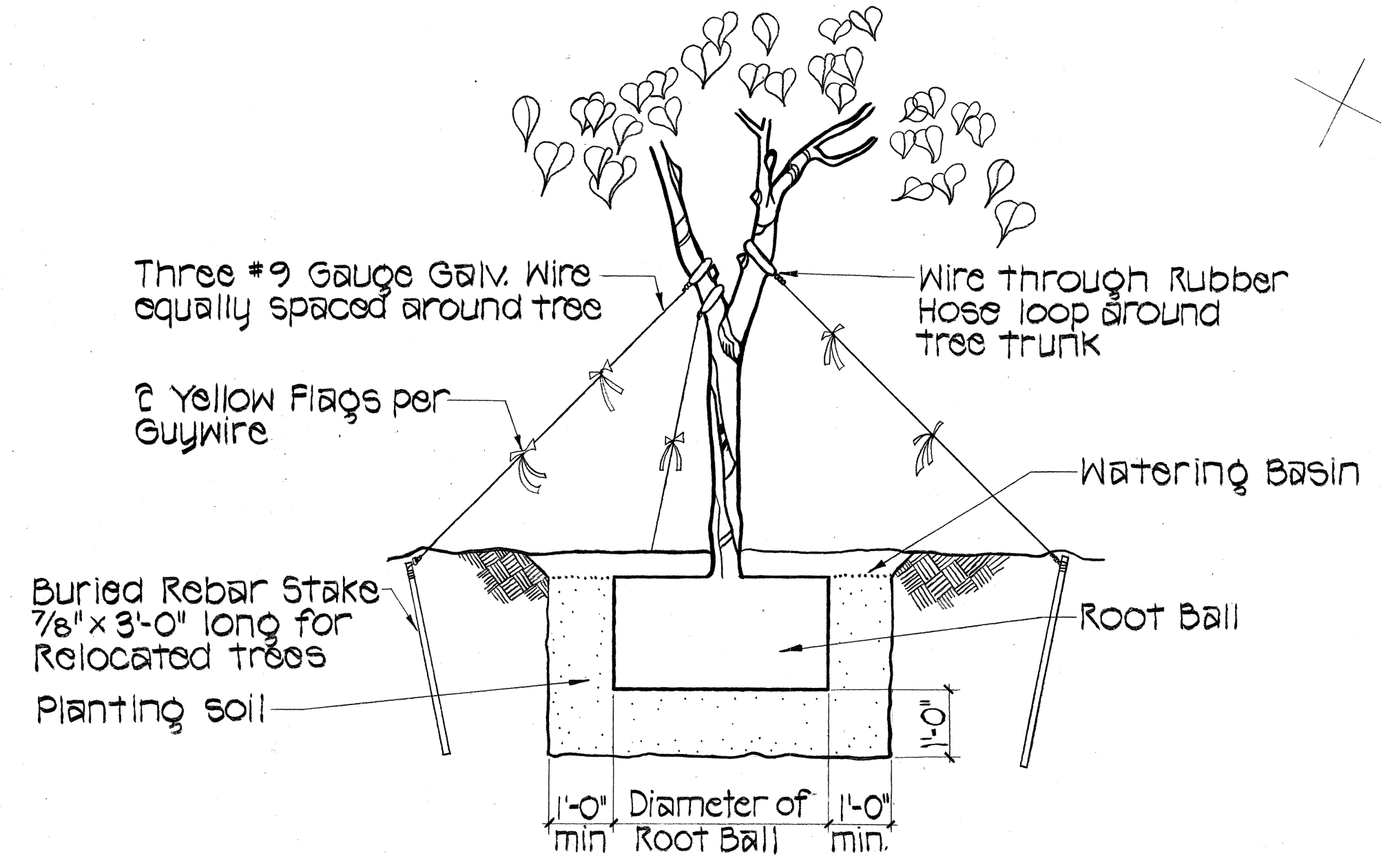
TRANSPLANTED TREE Not to Scale
