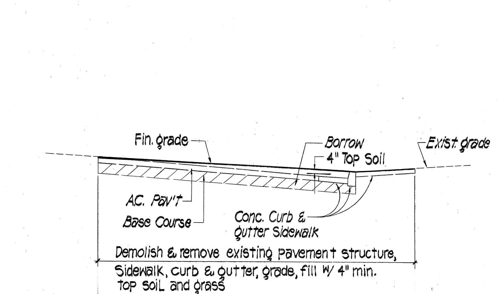
TYPICAL SECTION ~ ROADWAY DEMOLITION Not to Scale
