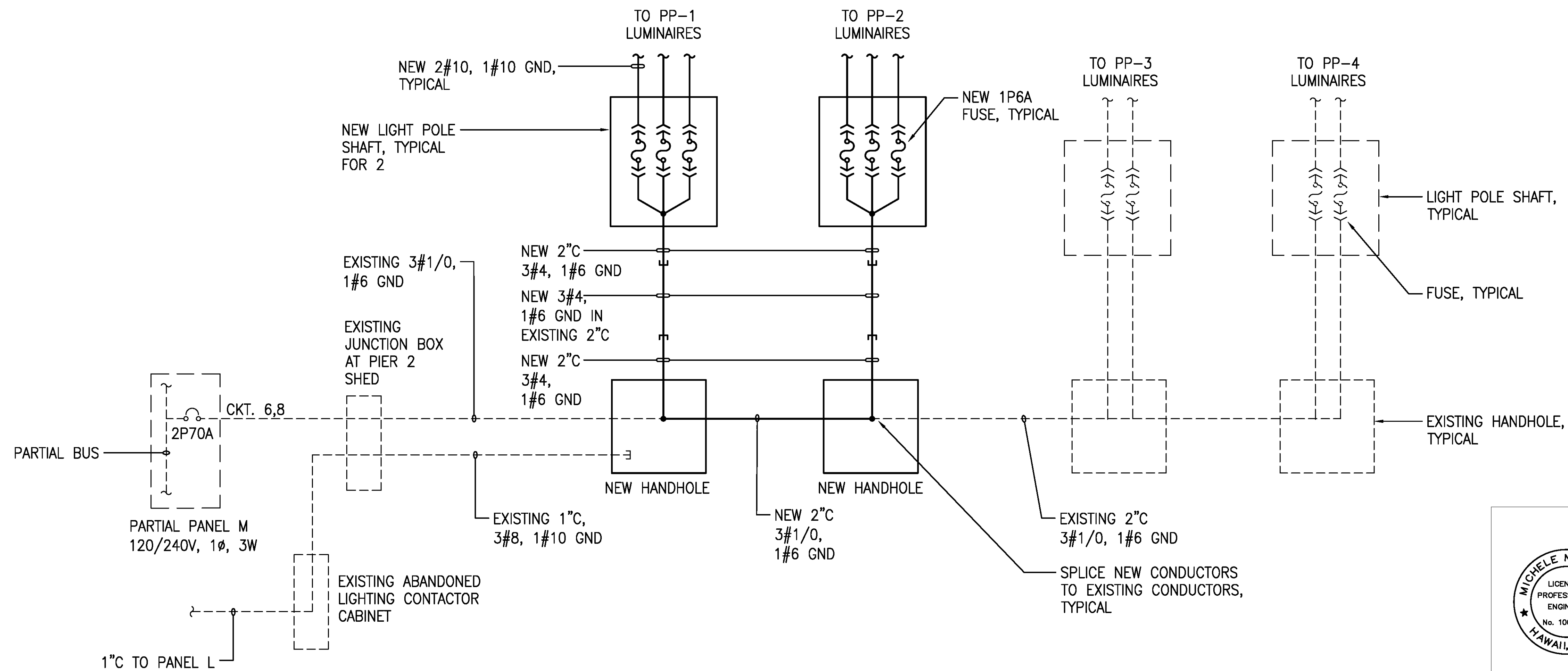
PARTIAL PIER 2 LIGHT POLE WIRING DIAGRAM - NEW WORK NO SCALE
