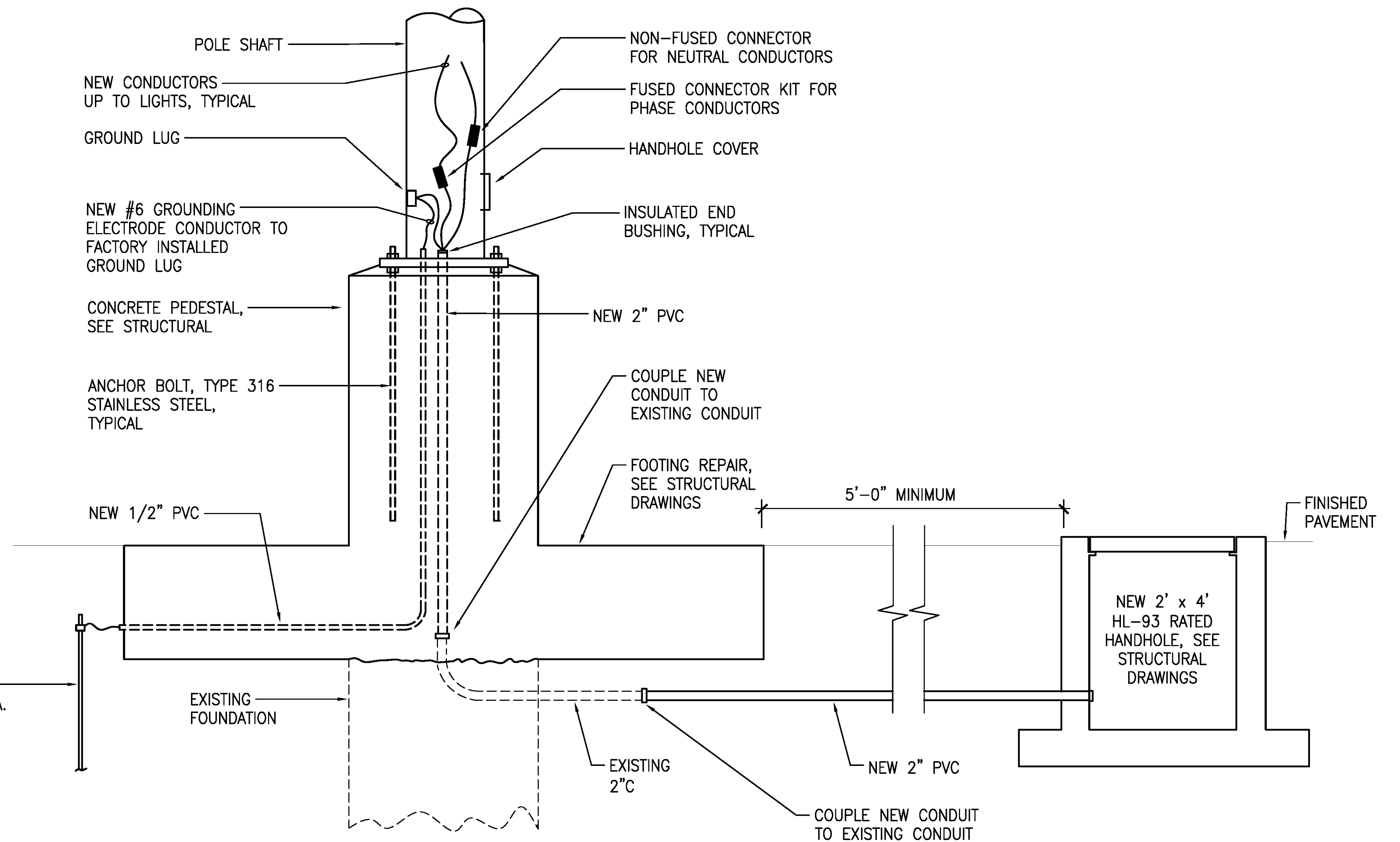
3 PEDESTAL - NEW WORK (PP-1, PP-2) E-7 NOT TO SCALE
