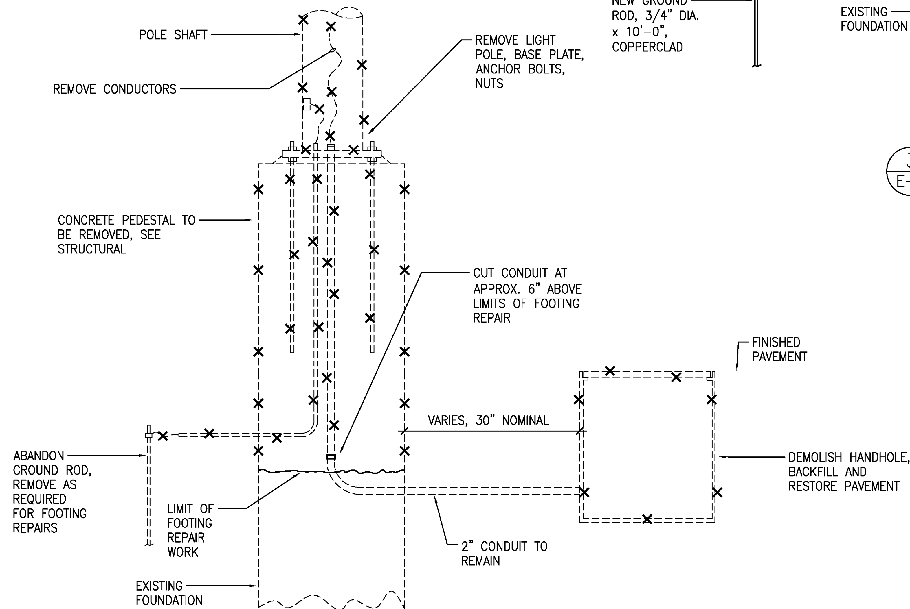
2 PEDESTAL - DEMOLITION WORK (PP-1, PP-2) E-7 NOT TO SCALE
