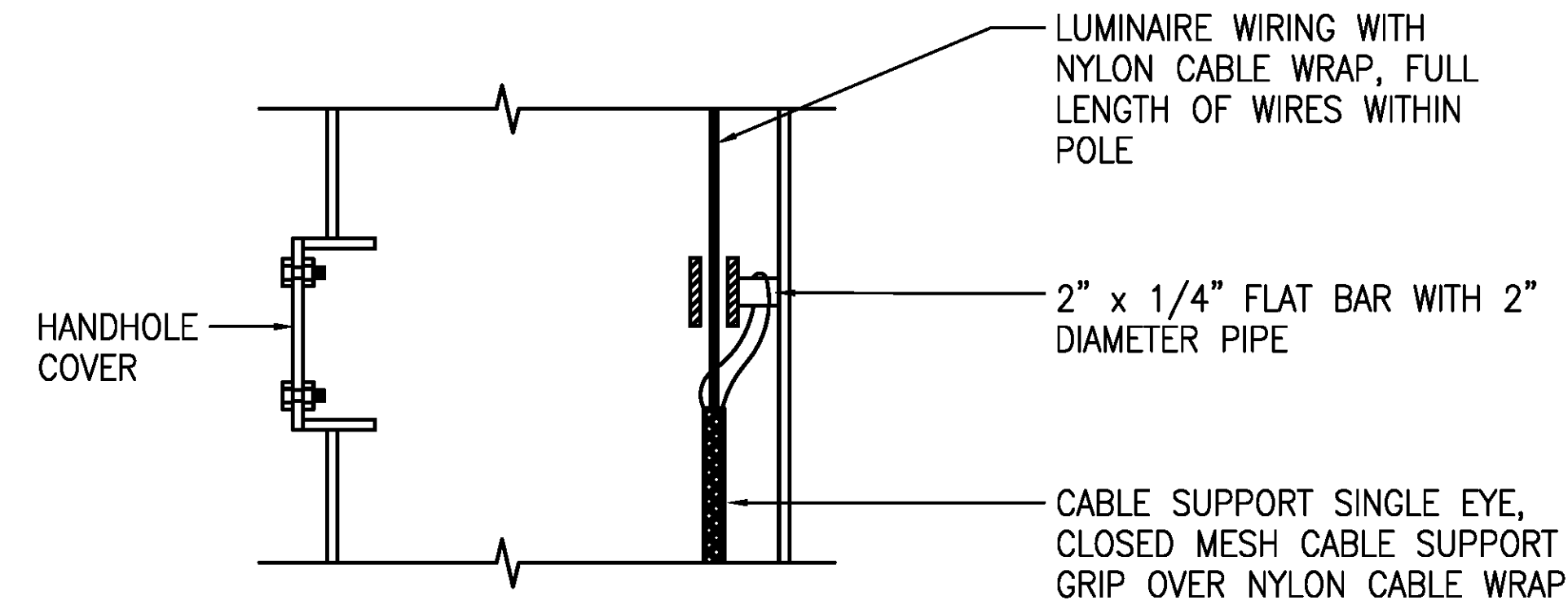
1 CABLE GUIDE DETAIL E-7 NOT TO SCALE
