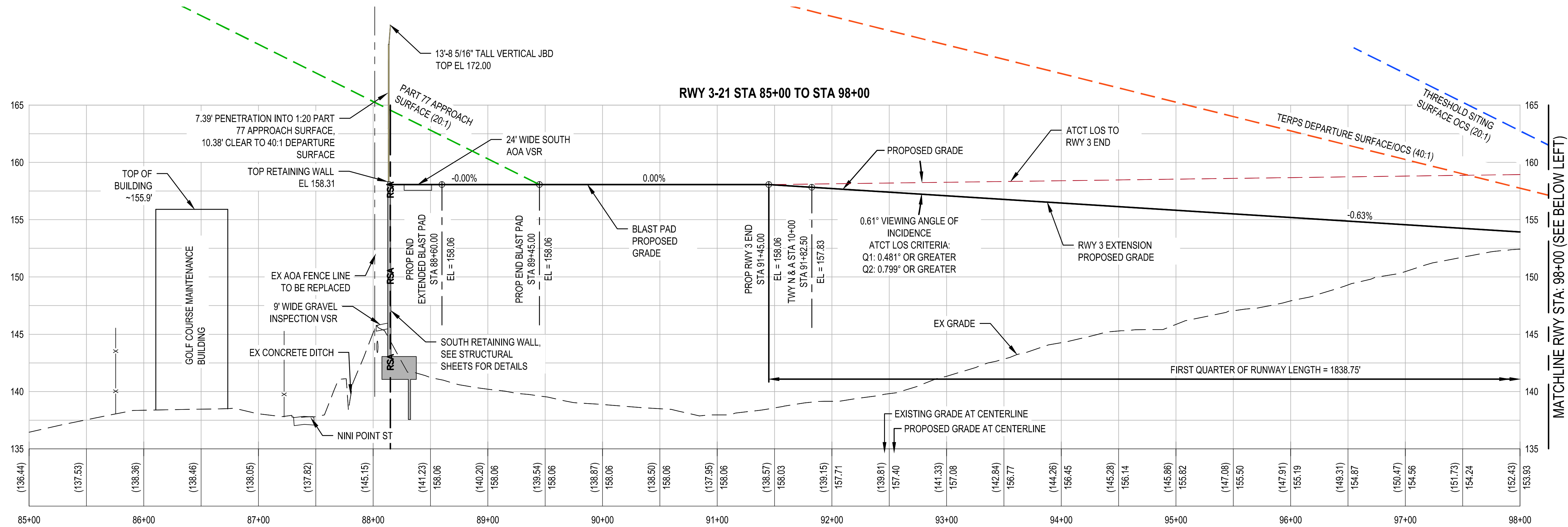
RUNWAY 3 - PROFILE STA 85+00 TO STA 98+00
