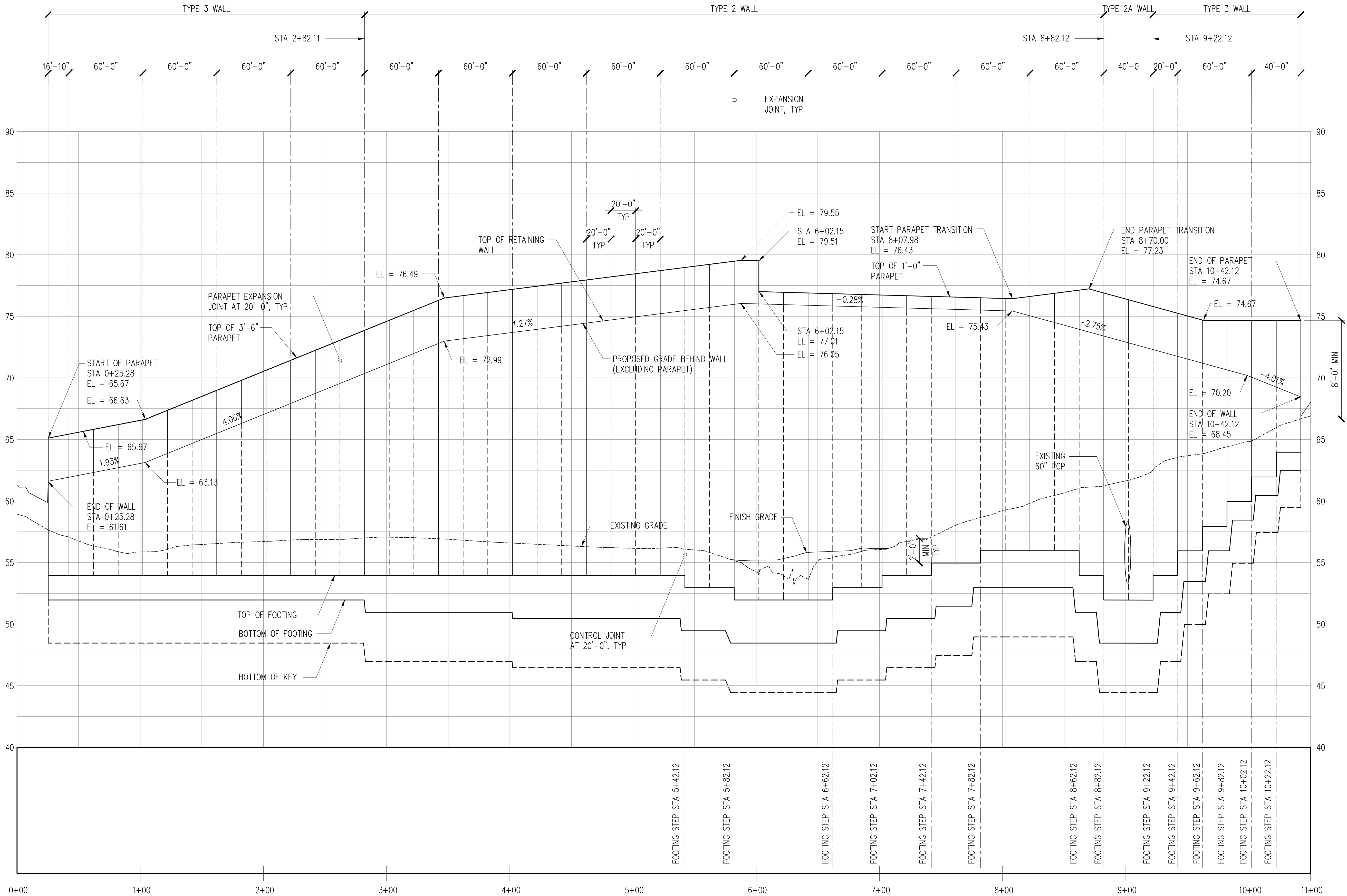
1 NORTH RETAINING WALL PROFILE S1.2 VERTICAL SCALE: 1" = 4'-0" HORIZONTAL SCALE: 1" = 40'-0"
