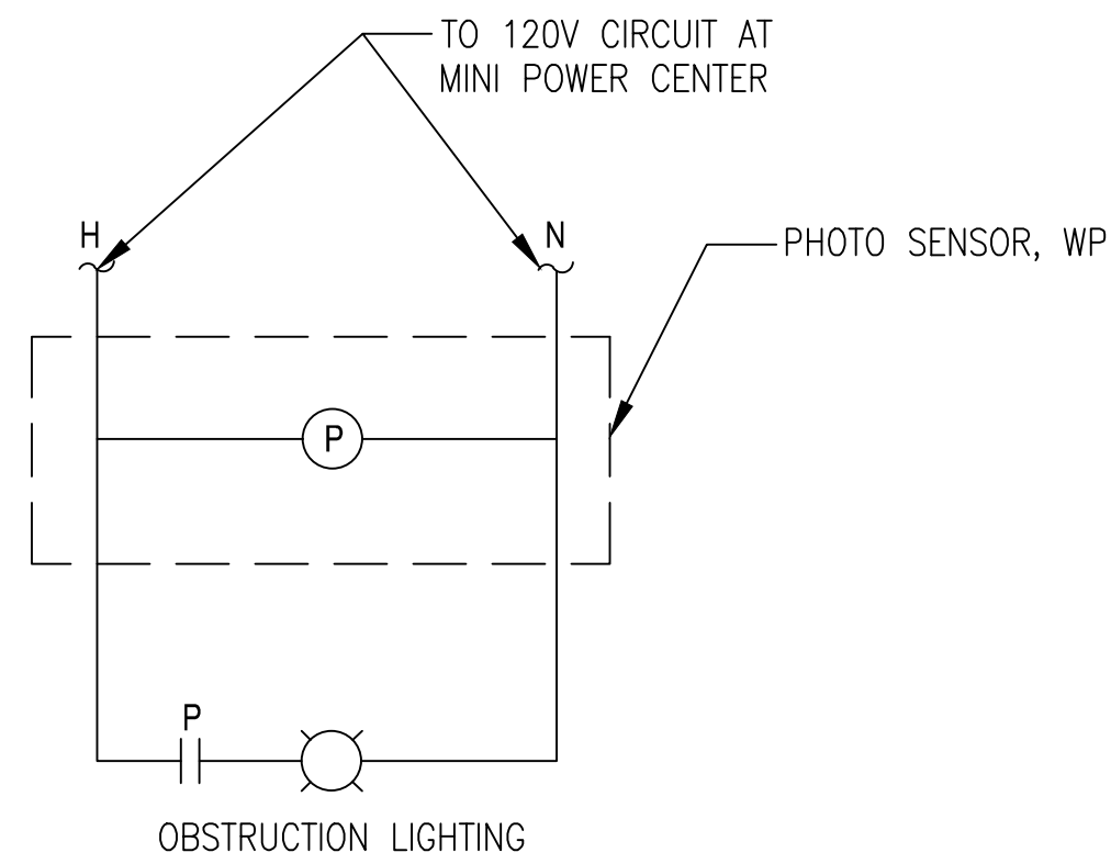
JET BLAST DEFLECTOR OBSTRUCTION LIGHTING CONTROL WIRING DIAGRAM SCALE: N.T.S.
