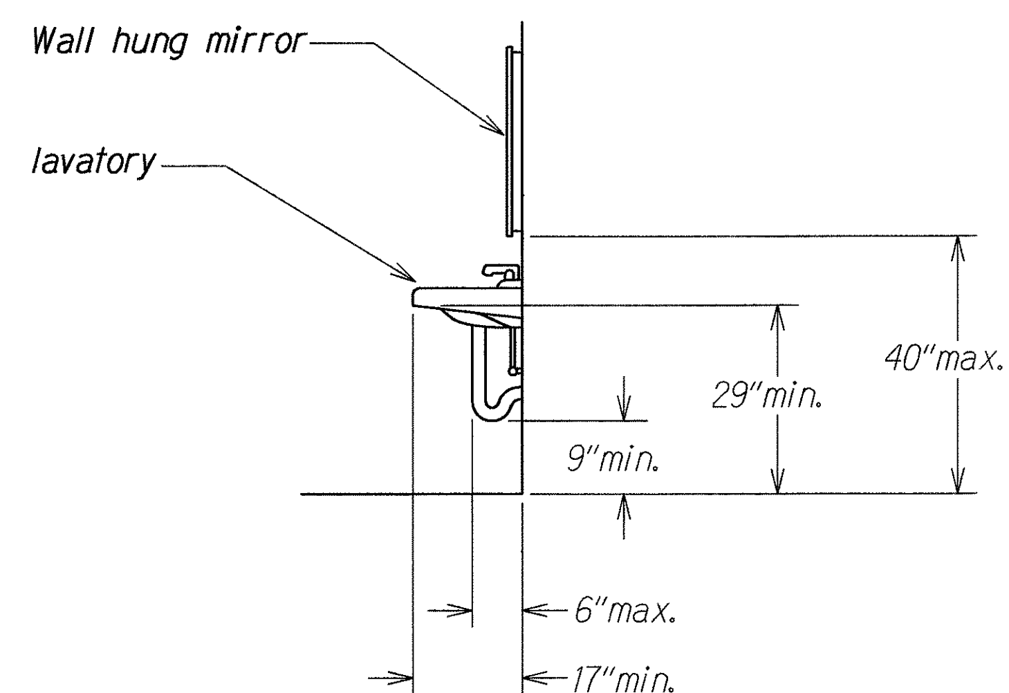
LAVATORY CLEARANCES Not to Scale
