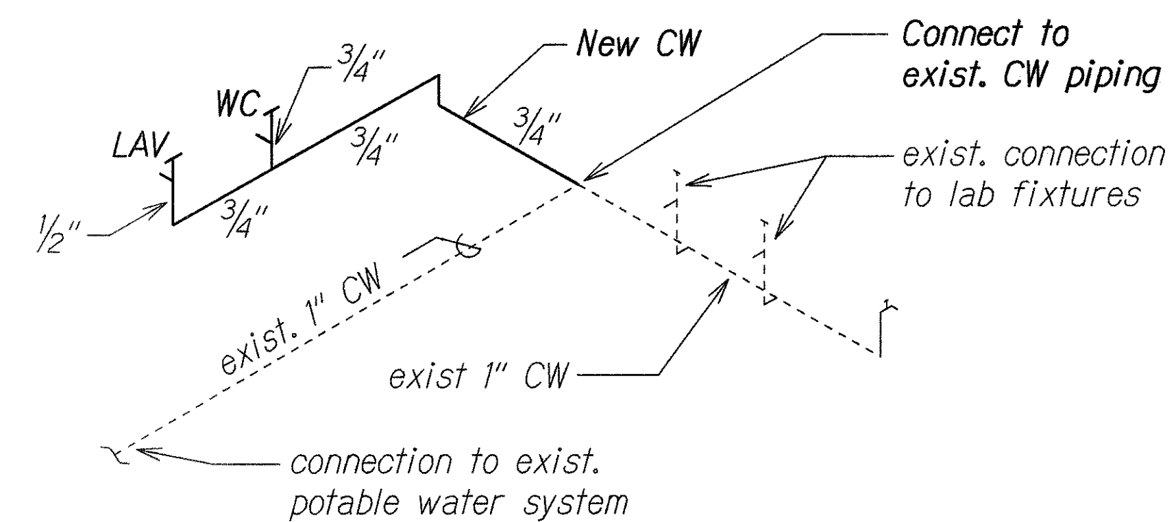
COLD WATER PIPING DIAGRAM FOR NEW BATHROOM (BUILDING C) Not to Scale
