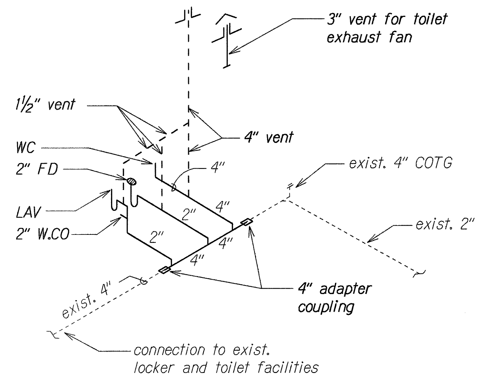
SANITARY SEWER DIAGRAM FOR NEW BATHROOM (BUILDING C) Not to Scale
