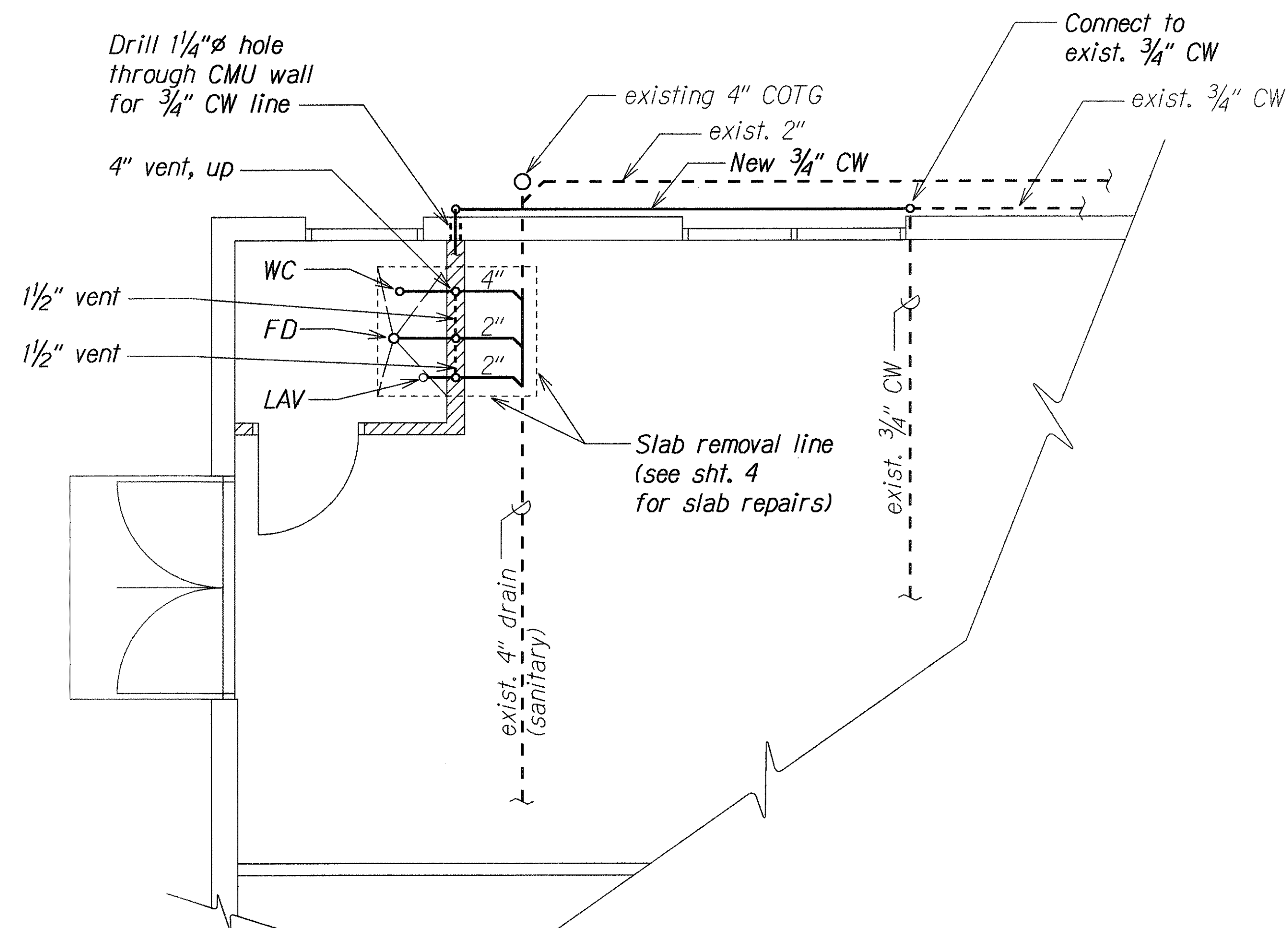
PLUMBING PLAN Scale: \frac{3}{8}"=1'
