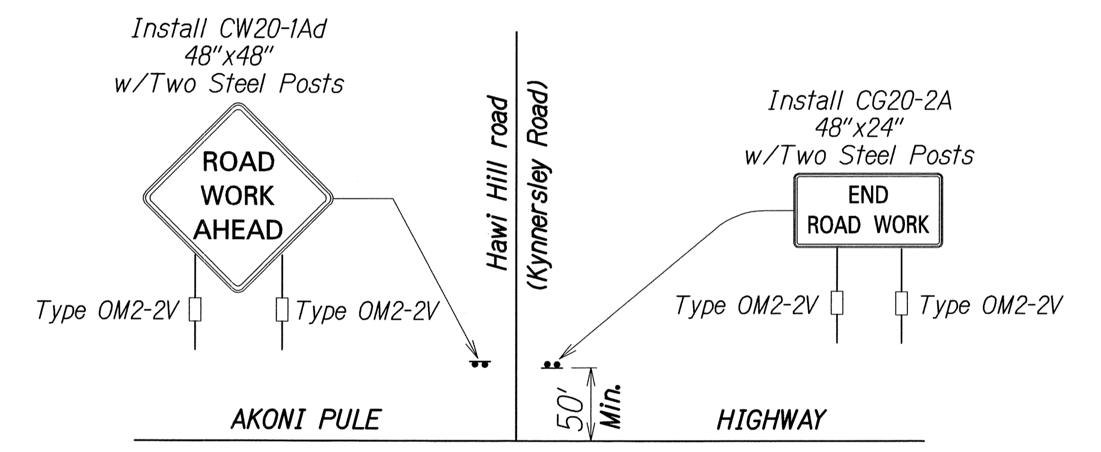
TYPICAL DETAIL FOR CONSTRUCTION SIGNS ERECTED ON SIDEROADS
