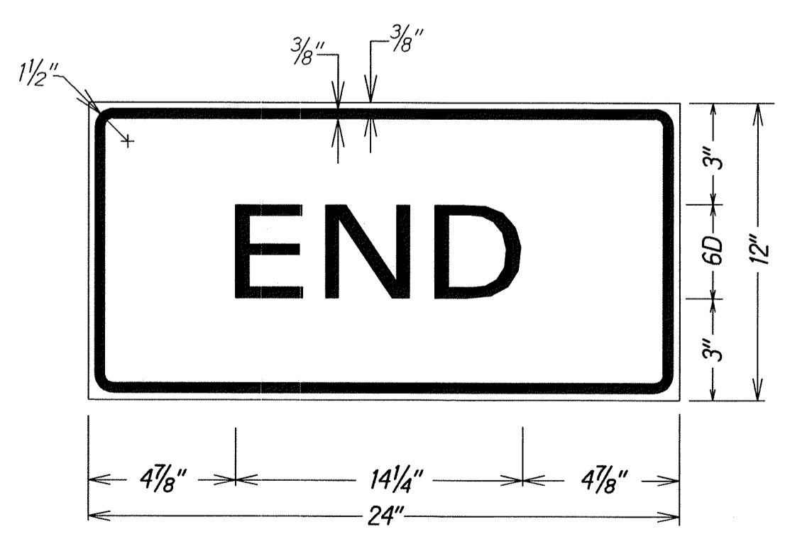
TYPICAL DETAIL FOR CONSTRUCTION SIGNS ERECTED ON SIDEROADS
