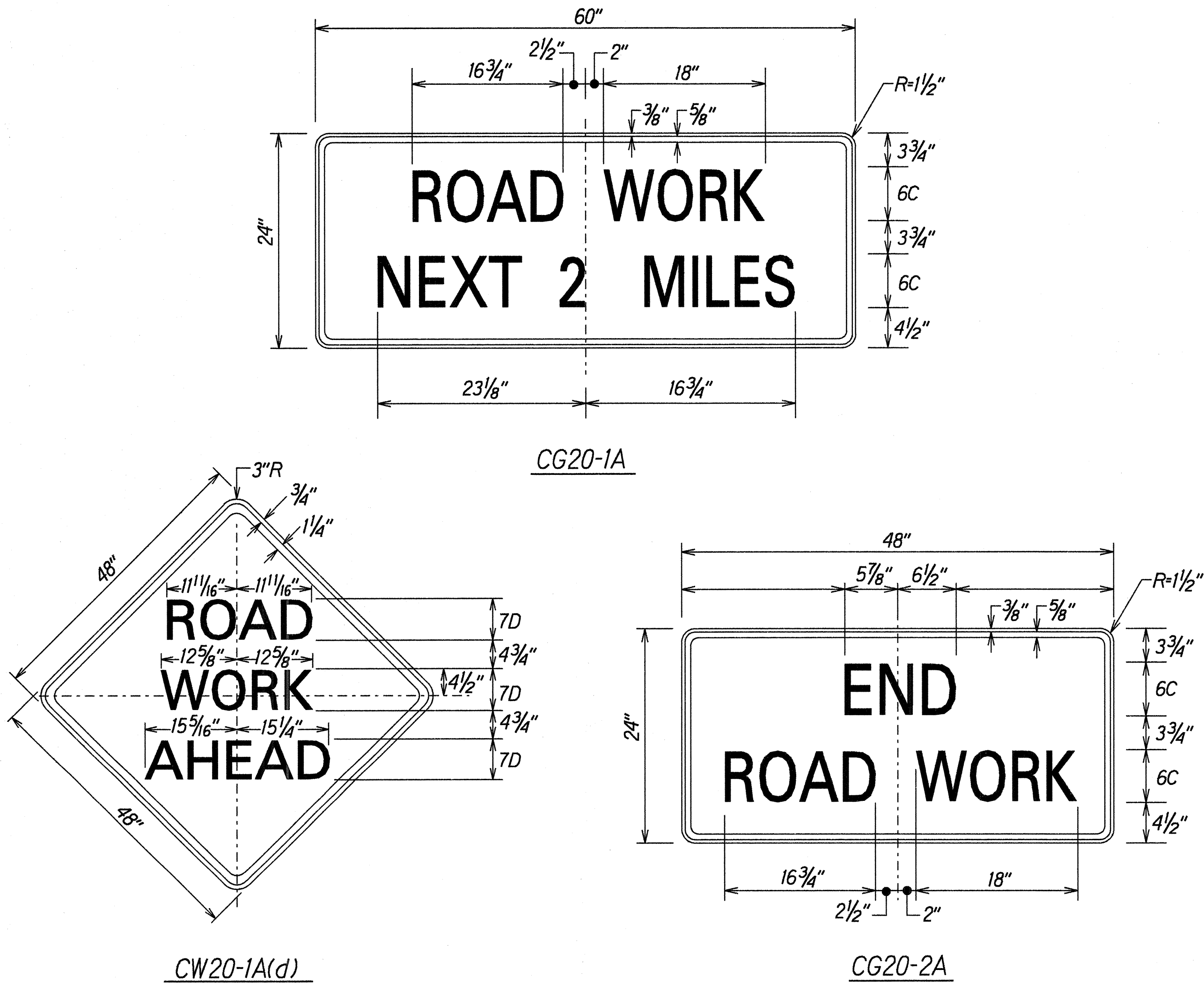
SIGN DETAILS Not To Scale
