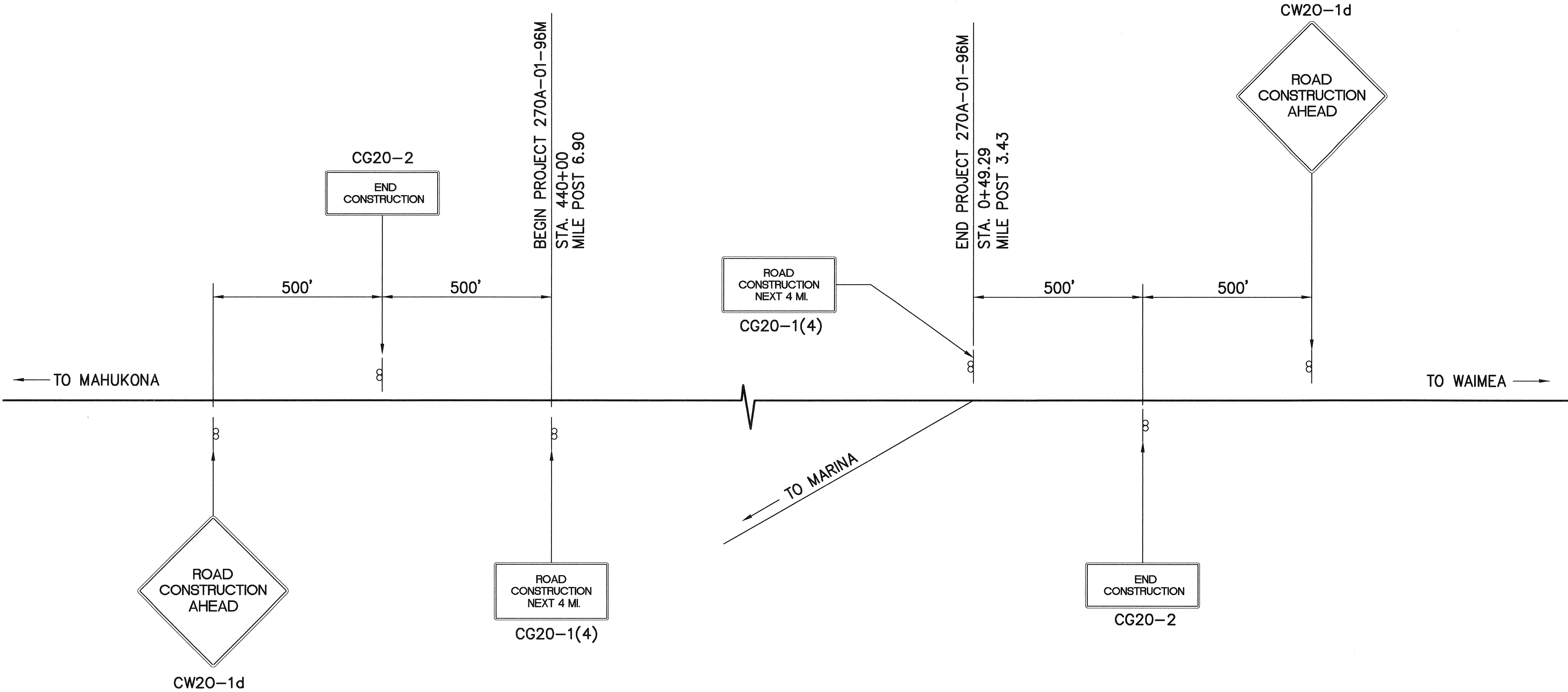
CONSTRUCTION SIGN PLAN NOT TO SCALE
