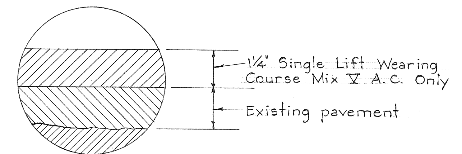
PAVEMENT DETAIL STA. 579+00 to STA. 605+08 Not To Scale
