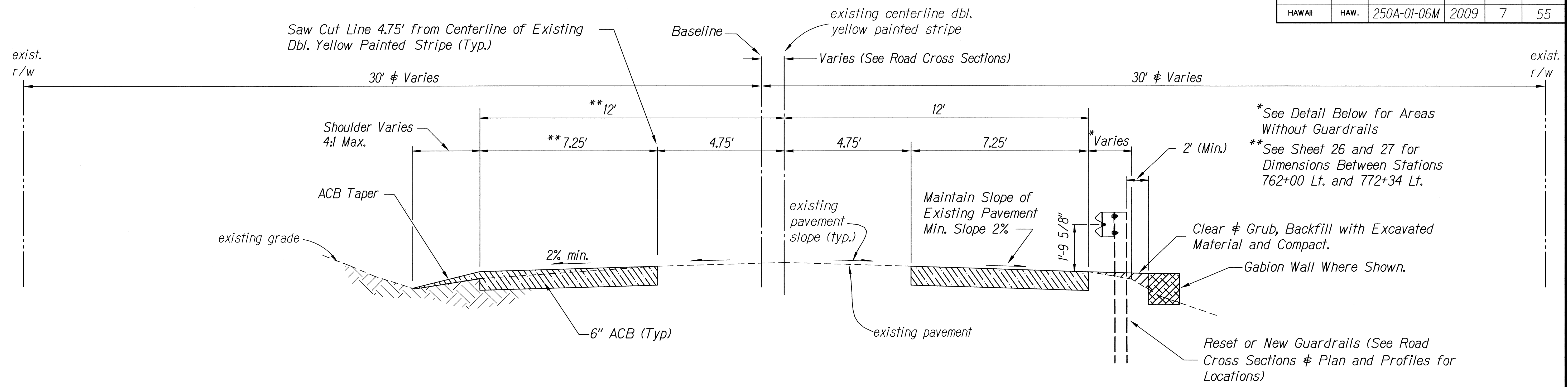
TYPICAL SECTION - KOHALA MOUNTAIN ROAD - NORMAL CROWN Scale: Not to Scale
