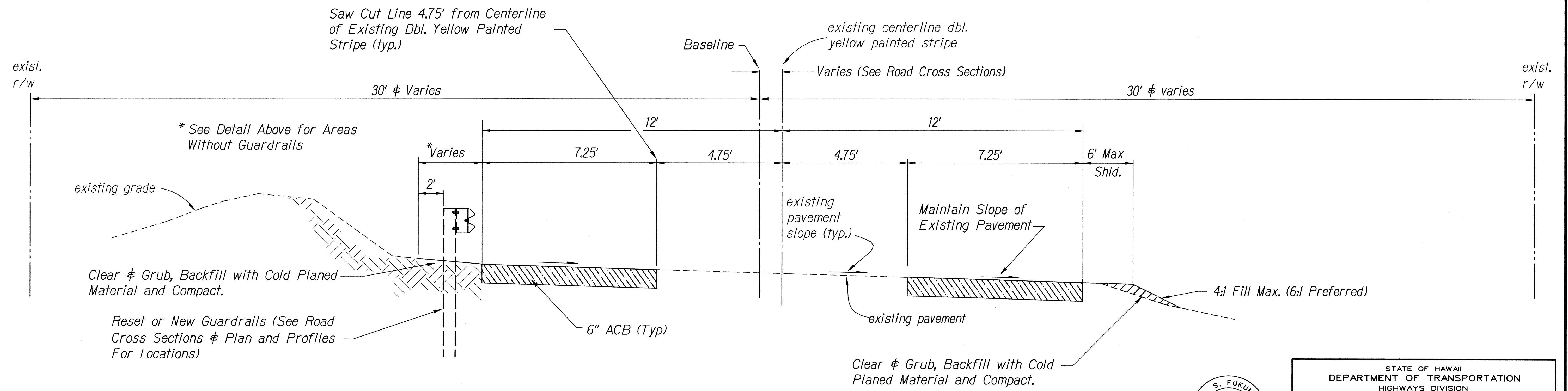
TYPICAL SECTION - KOHALA MOUNTAIN ROAD - SUPERELEVATED SECTION Scale: Not to Scale
