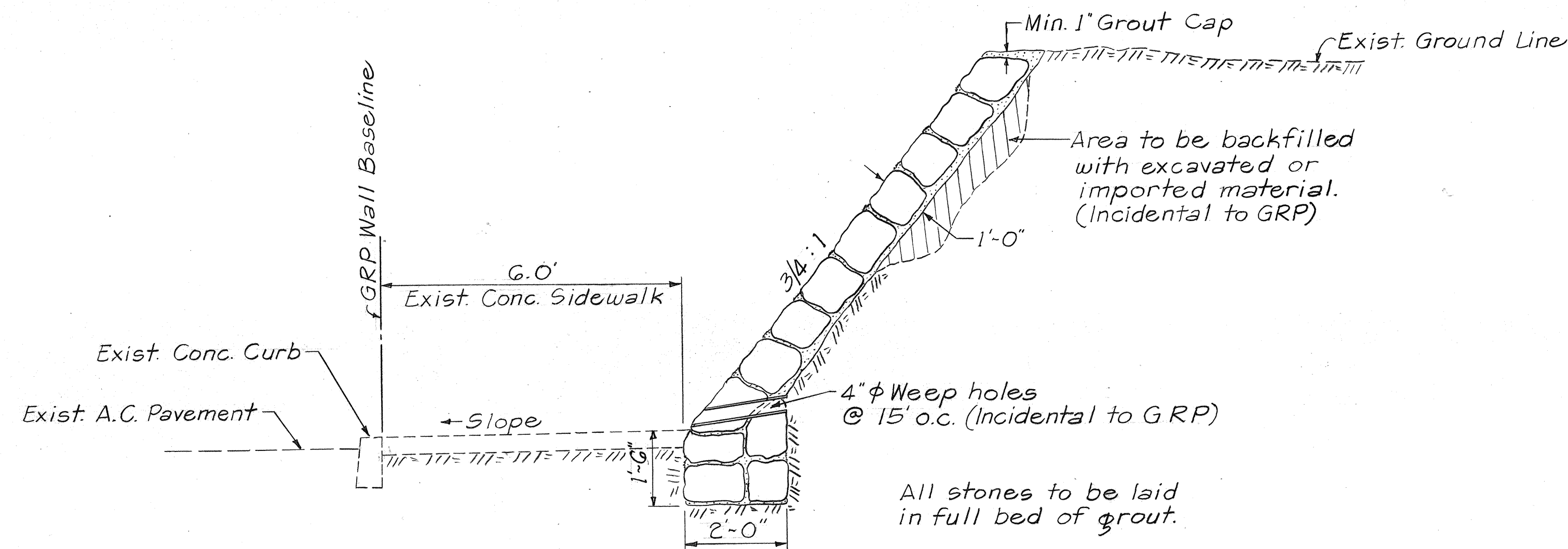
GRP WALL DETAIL Scale: 1/2"=1'-0"
