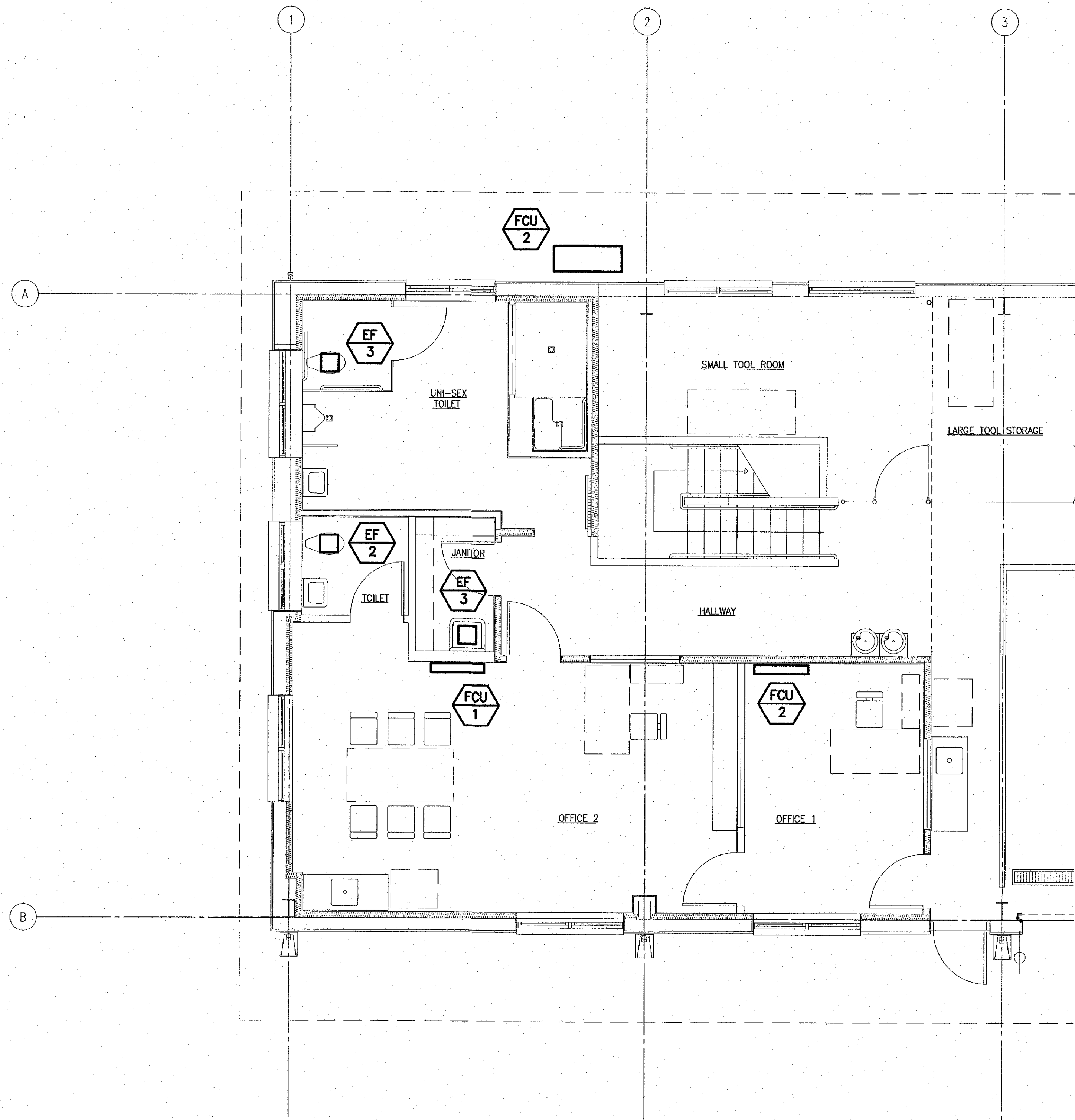
SHOP BUILDING PARTIAL ACV PLAN SCALE: 1/4" = 1'-0"
