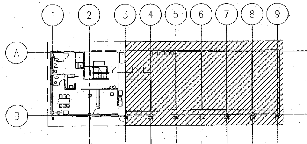
SHOP BUILDING
