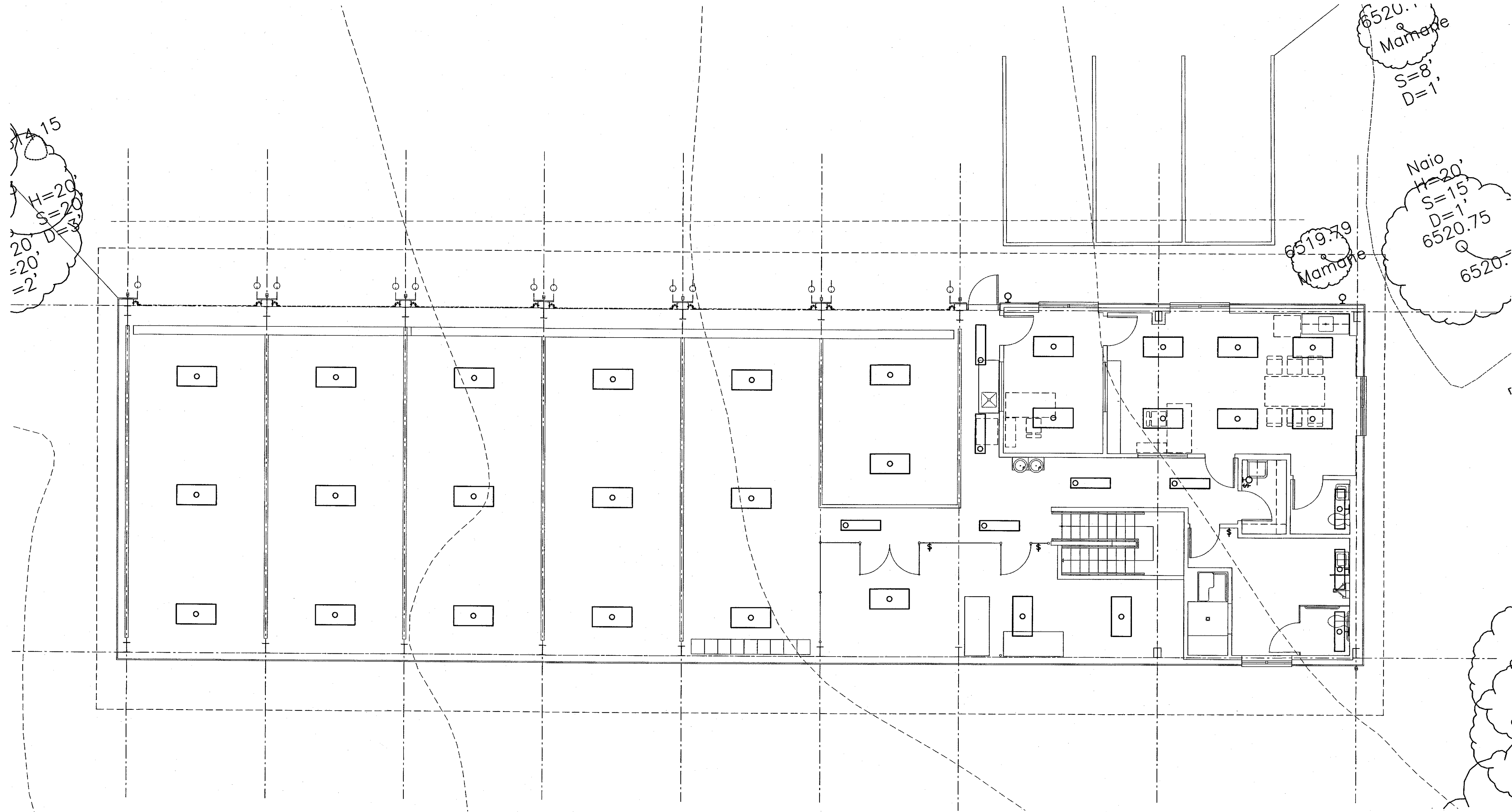
SHOP BUILDING LIGHTING PLAN SCALE: 3/16"=1'-0"
