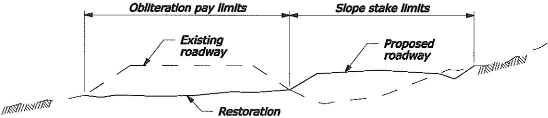
ROADWAY OBLITERATION, METHOD 1 TYPICAL SECTION
