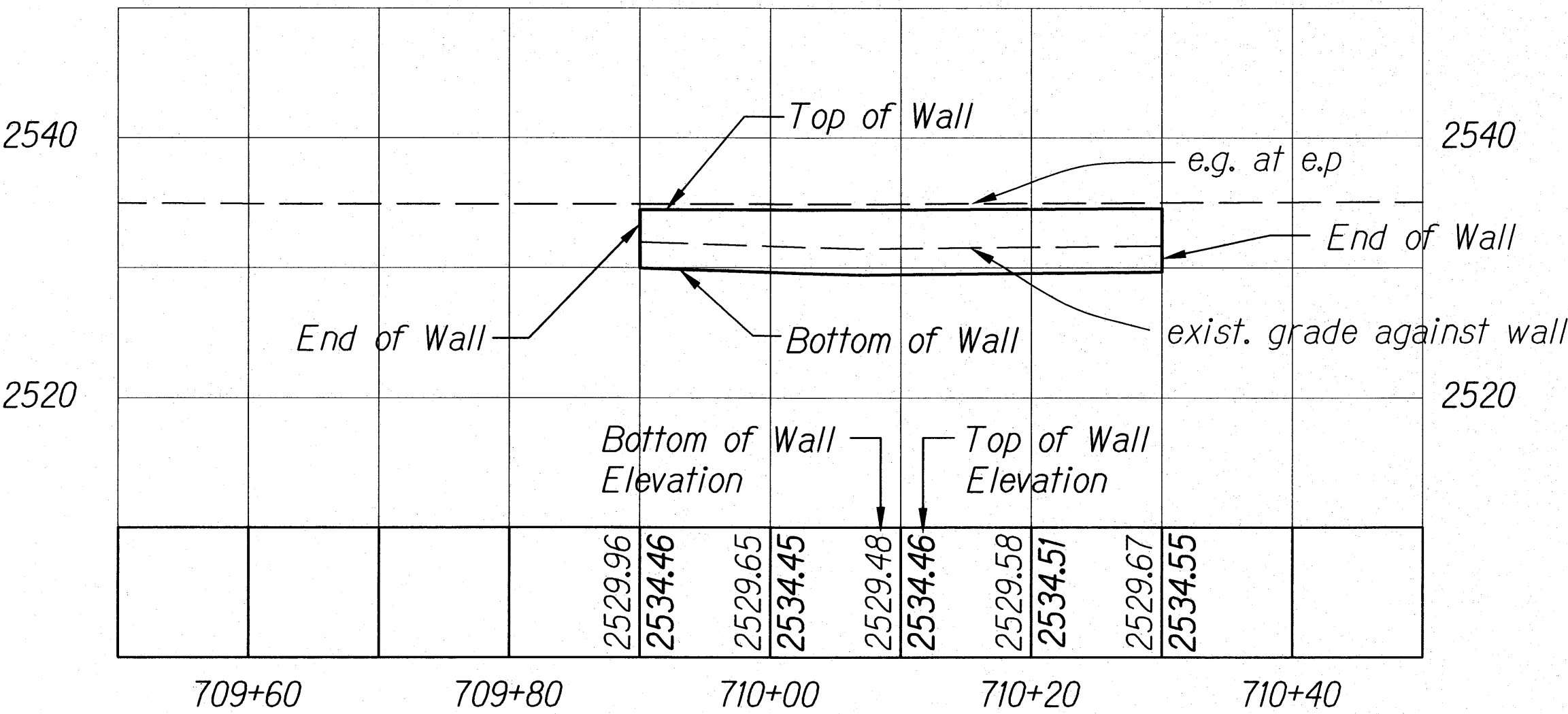
CRM WALL PROFILE - MP 15.3 MAKAI STA. 709+90 TO 710+30 Scale: 1"=10'
