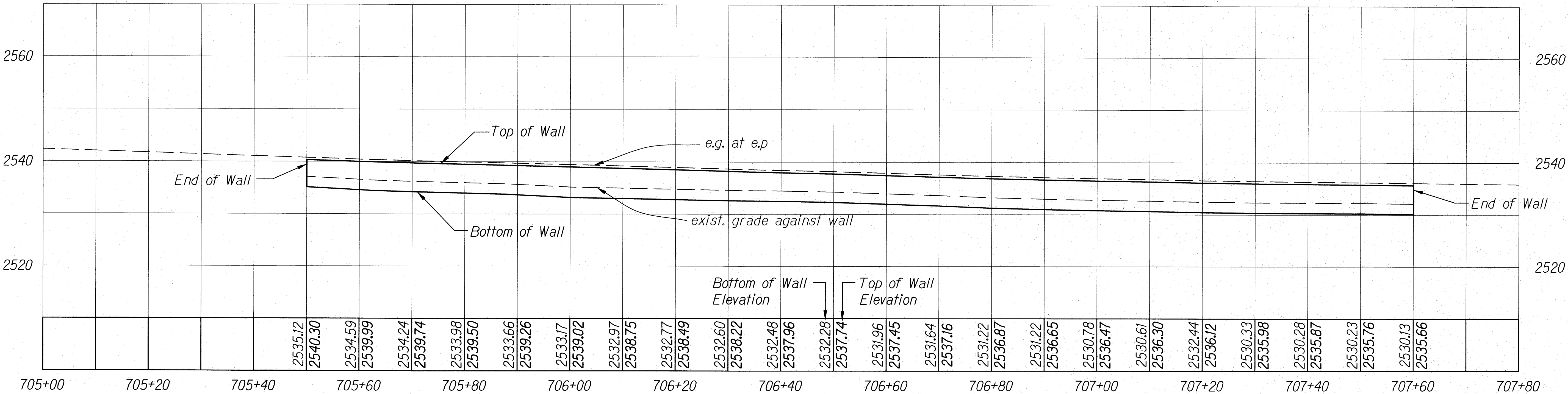
CRM WALL PROFILE - MP 15.3 MAKAI STA. 705+50 TO 707+60 Scale: 1"=10'
