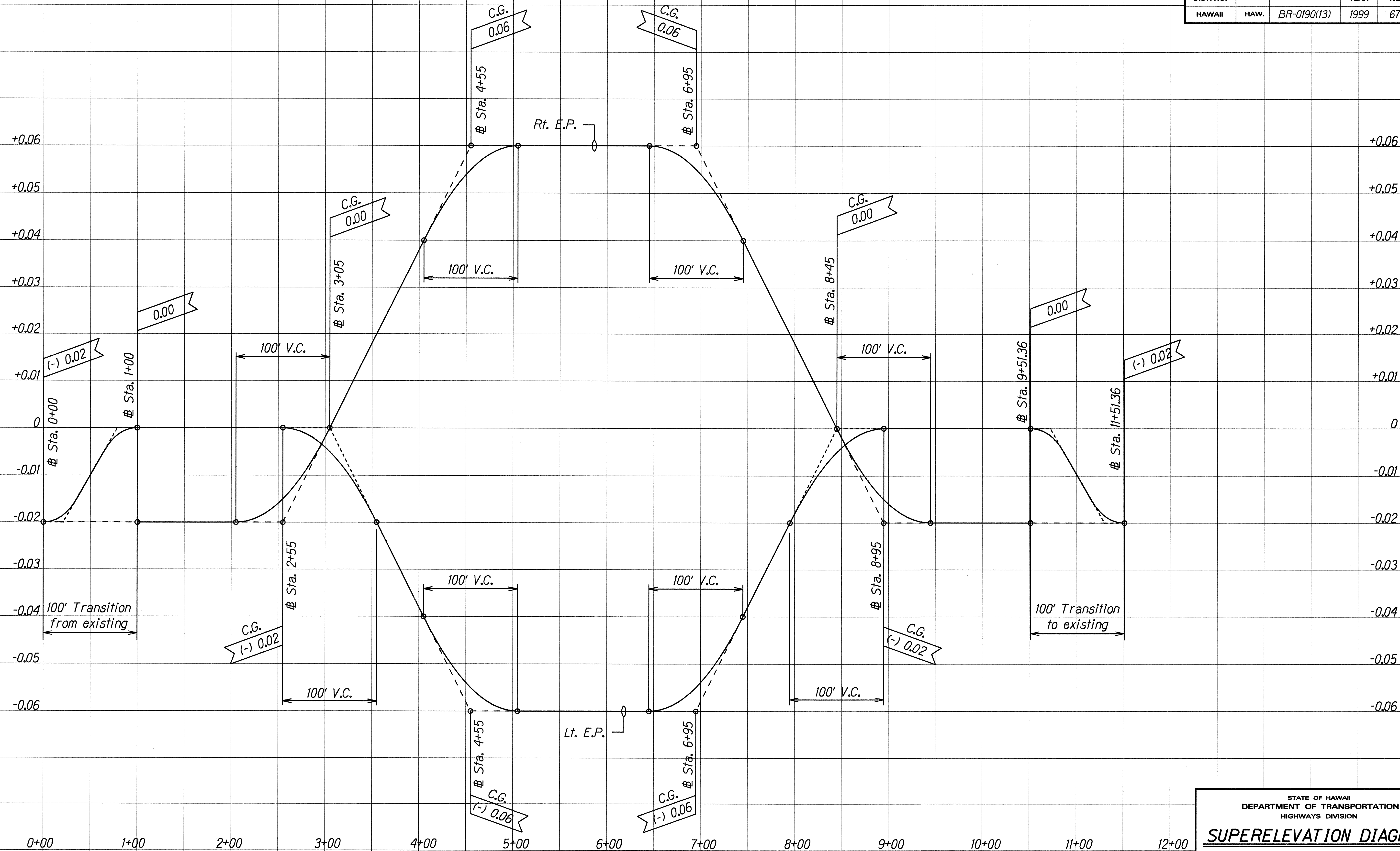
SUPERELEVATION DIAGRAM - POPOO BRIDGE DETOUR ROAD
