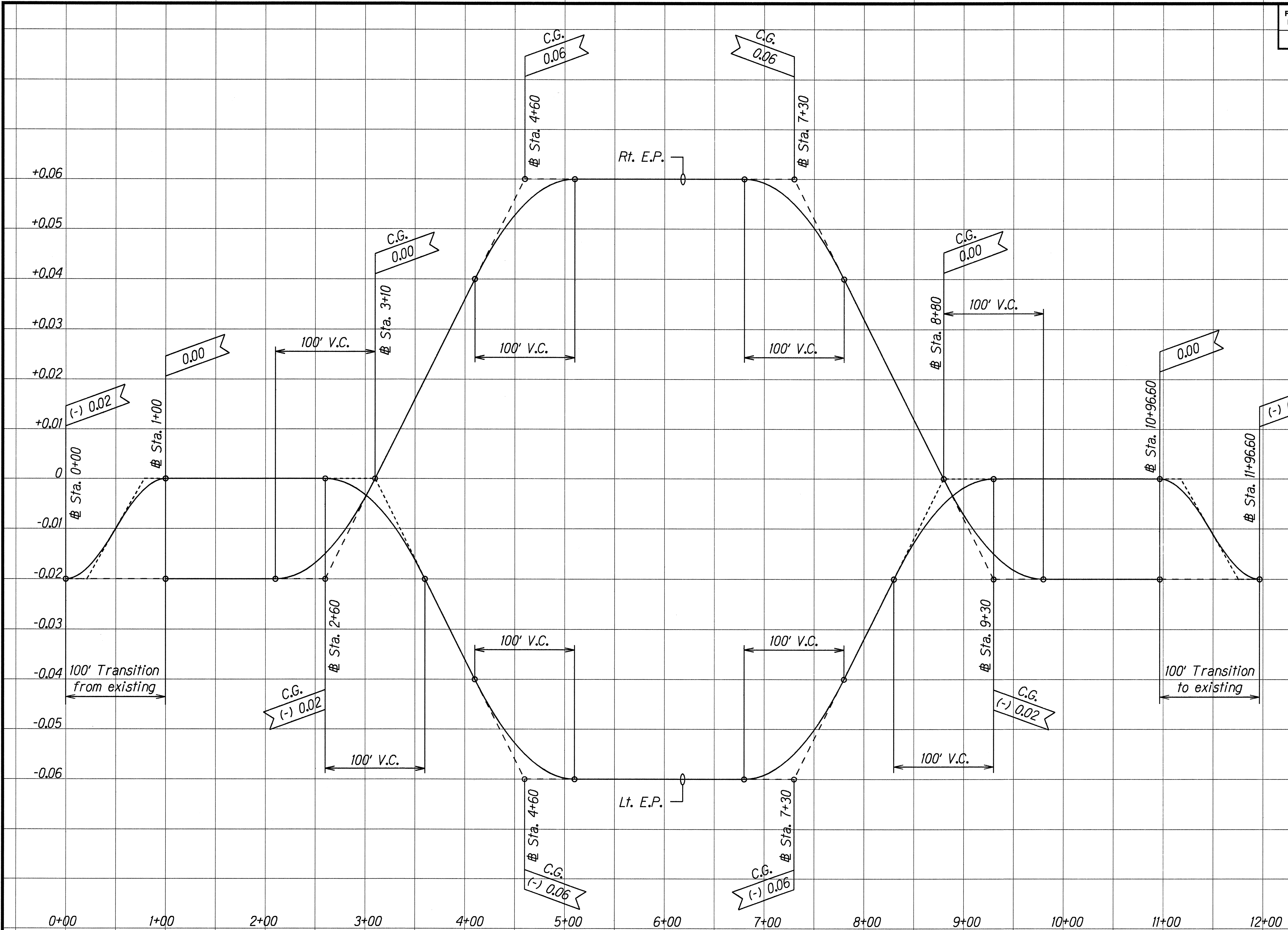
SUPERELEVATION DIAGRAM - AUWAIKEAKUA BRIDGE DETOUR ROAD
