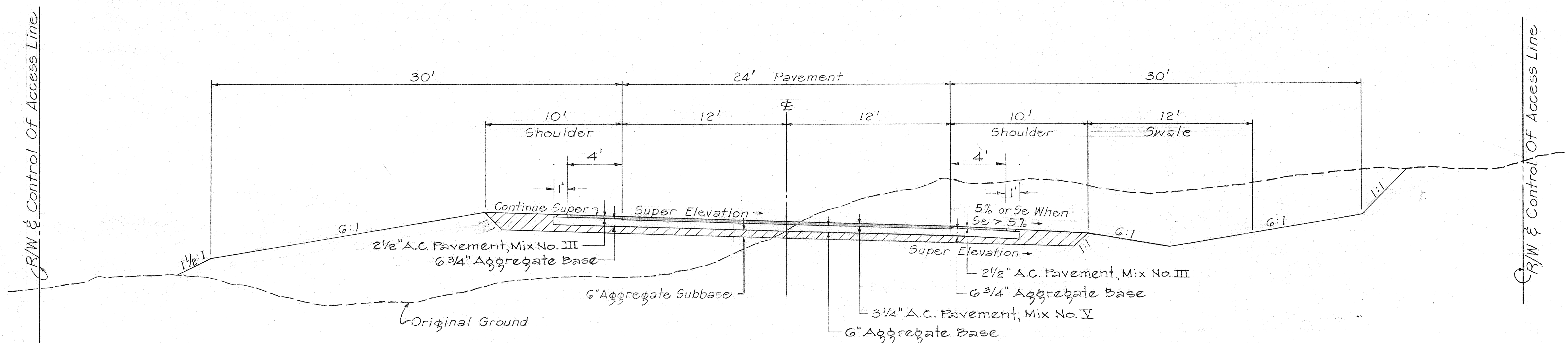
TYPICAL SECTION ON CURVE
