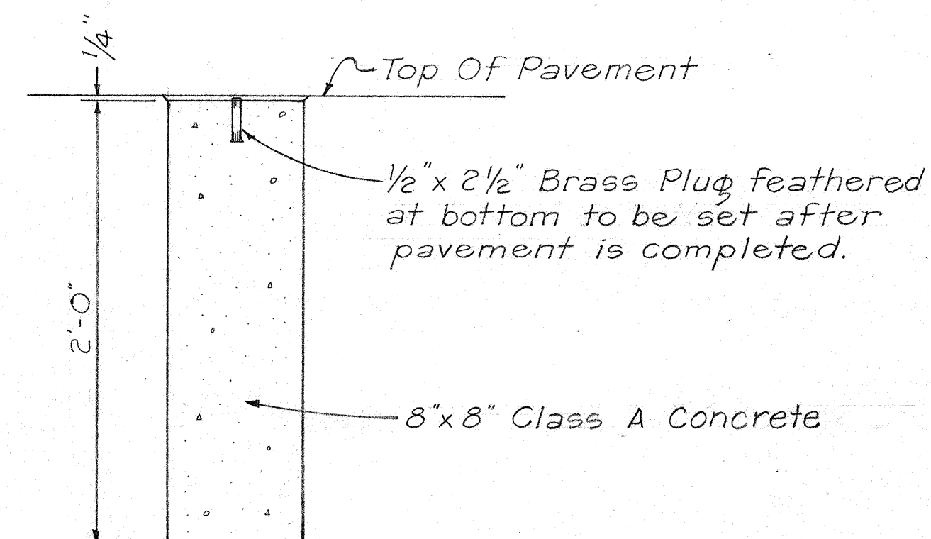
CENTERLINE MONUMENT DETAIL
