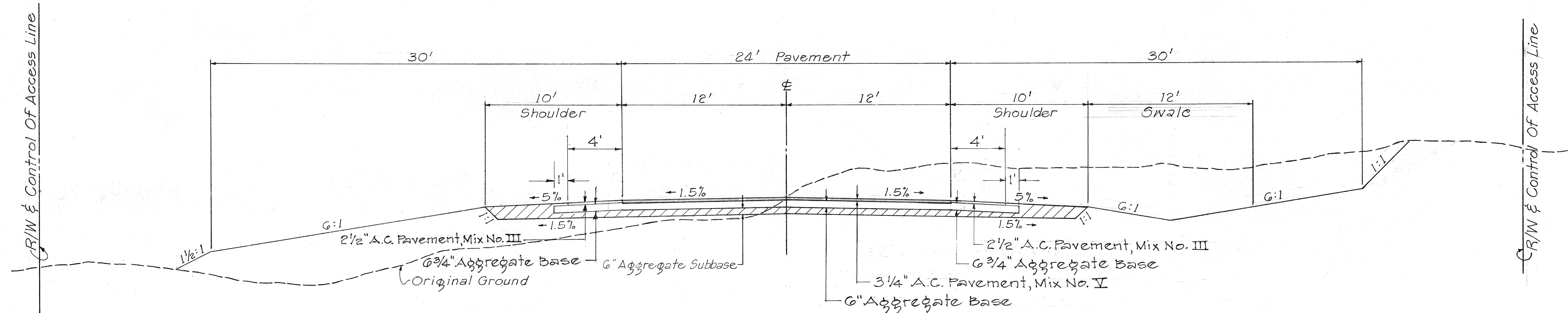
TYPICAL SECTION ON TANGENT
