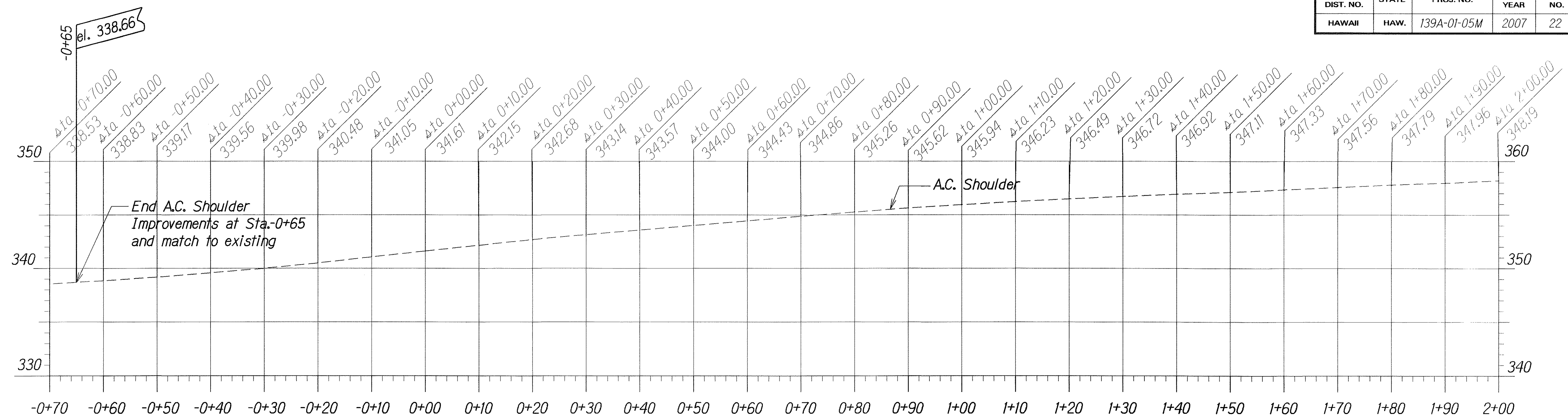
PROFILE ROUTE NO. 1 \phi OF SIDEWALK \phi A.C. SHOULDER (STATION (-)0+65 TO STATION 2+00)
