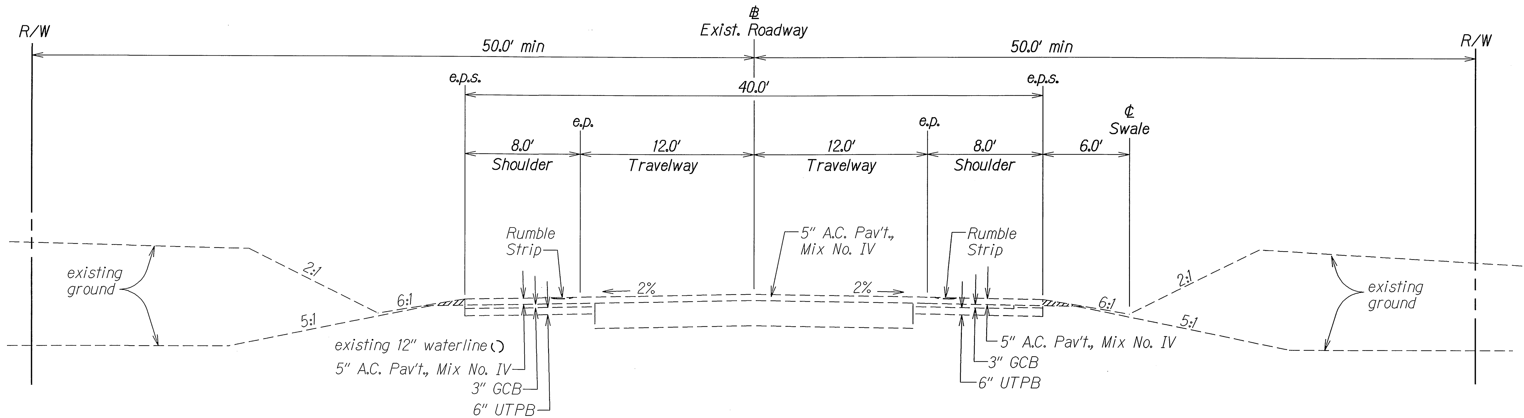
TYPICAL EXISTING TANGENT SECTION & WATERLINE Scale: 1/4" = 1'-0"
