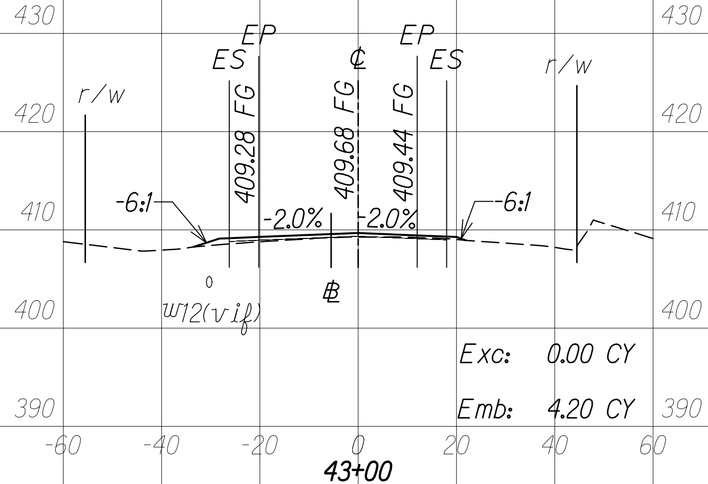
ROADWAY CROSS SECTIONS (KEAAU-PAHOA RD.) Scale: Horiz. 1" = 20' Vert. 1" = 10'
