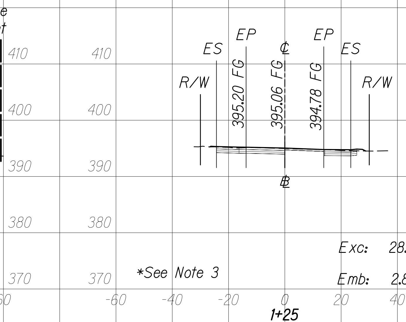
ROADWAY CROSS SECTIONS (ORCHIDLAND DR.) Scale: Horiz. 1" = 20' Vert. 1" = 10'
