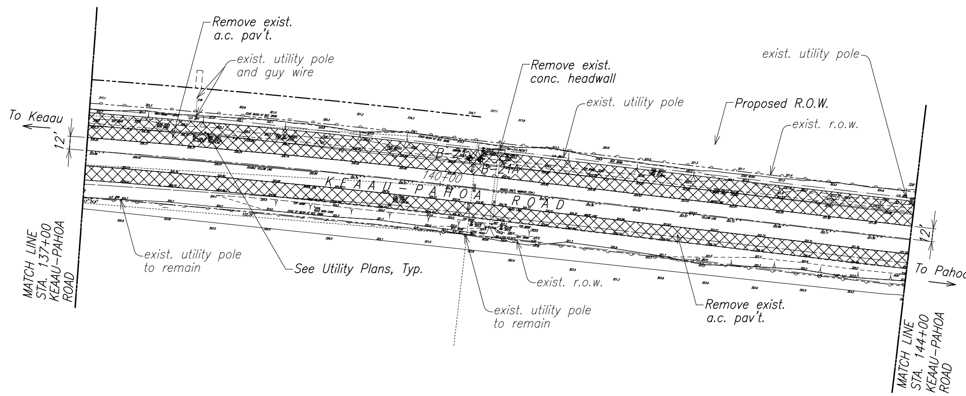
DEMOLITION PLAN - 4 Scale: 1" = 40'
