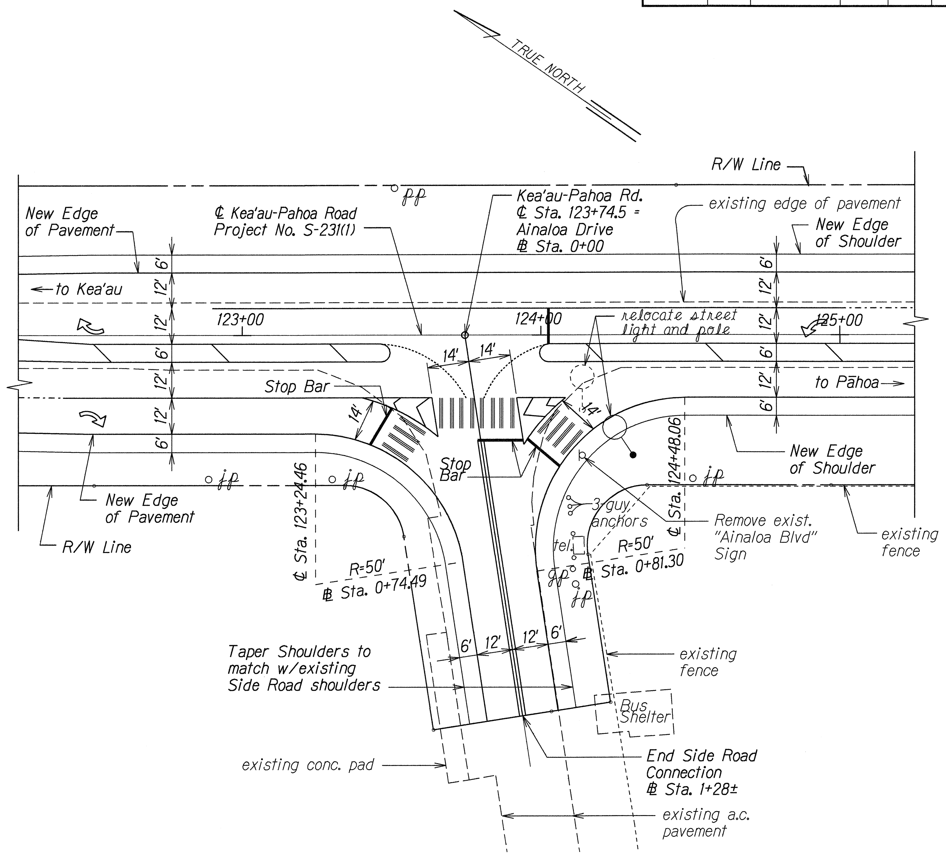
SIDE ROAD PLAN - AINALOA BLVD Scale 1" = 20'
