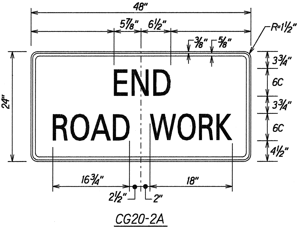
SIGN DETAILS Not To Scale
