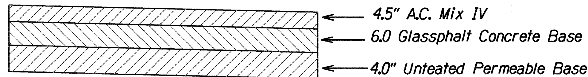
TYPICAL SECTION FOR ROAD "E" & DECELERATION LANE
