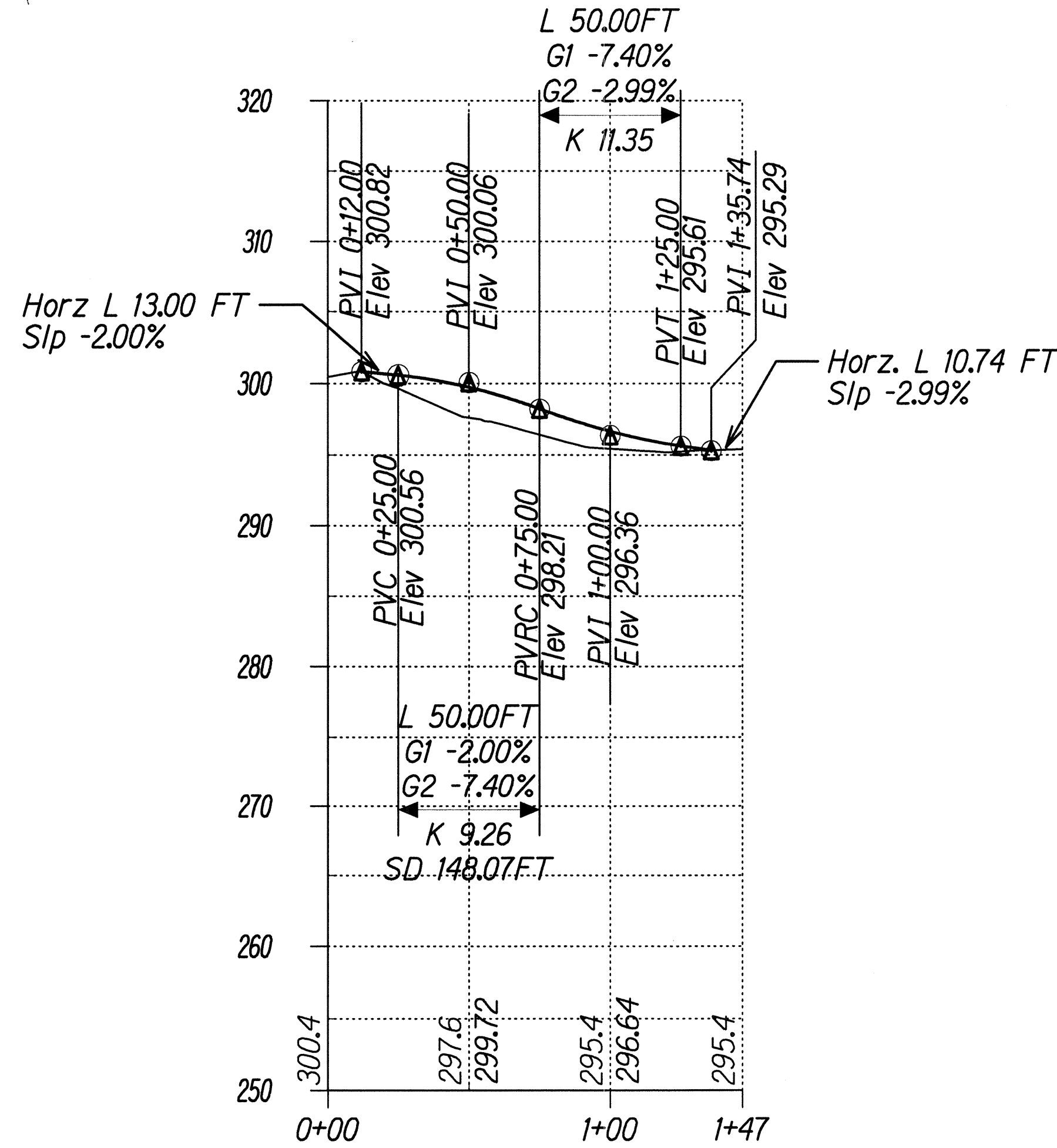
PROFILE ROAD "E"
