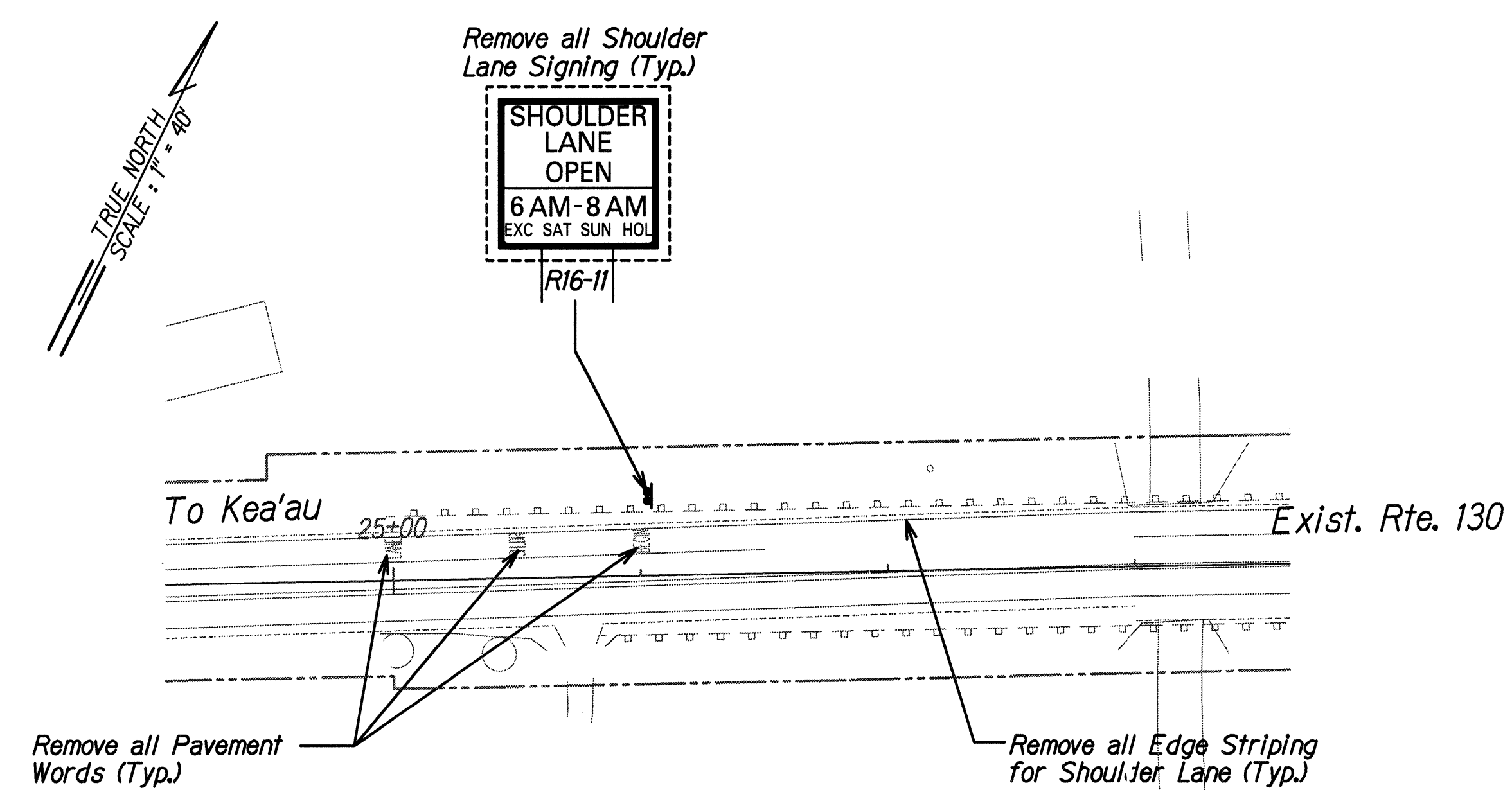
TYPICAL SHLDR. LANE REMOVAL DETAIL SCALE: 1"=40'
