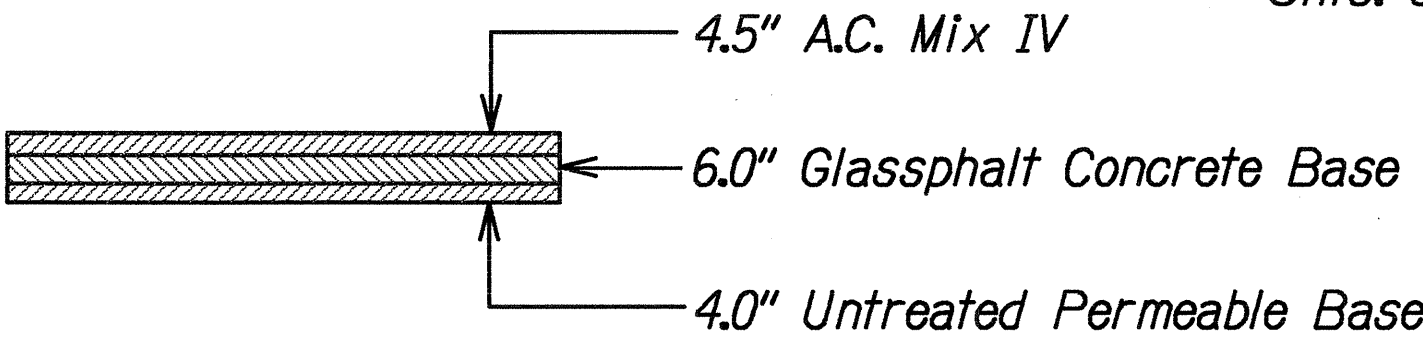
Typical Section for All Median Sections Scale: N.T.S.
