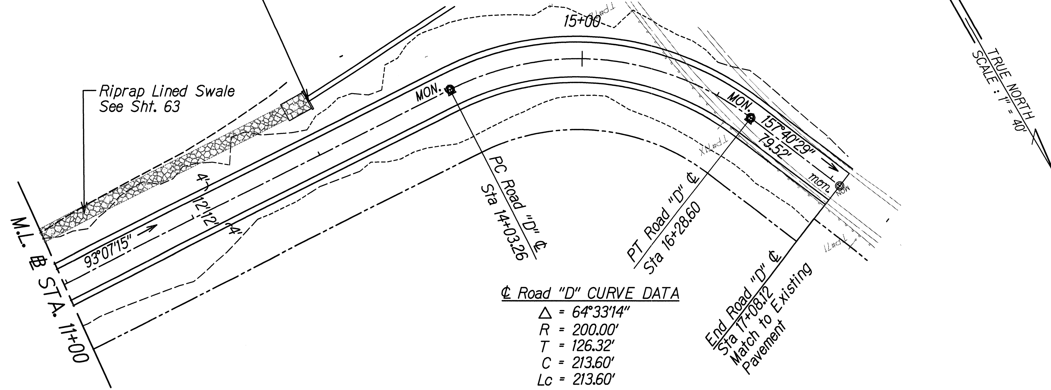
ROAD "D" PLAN
