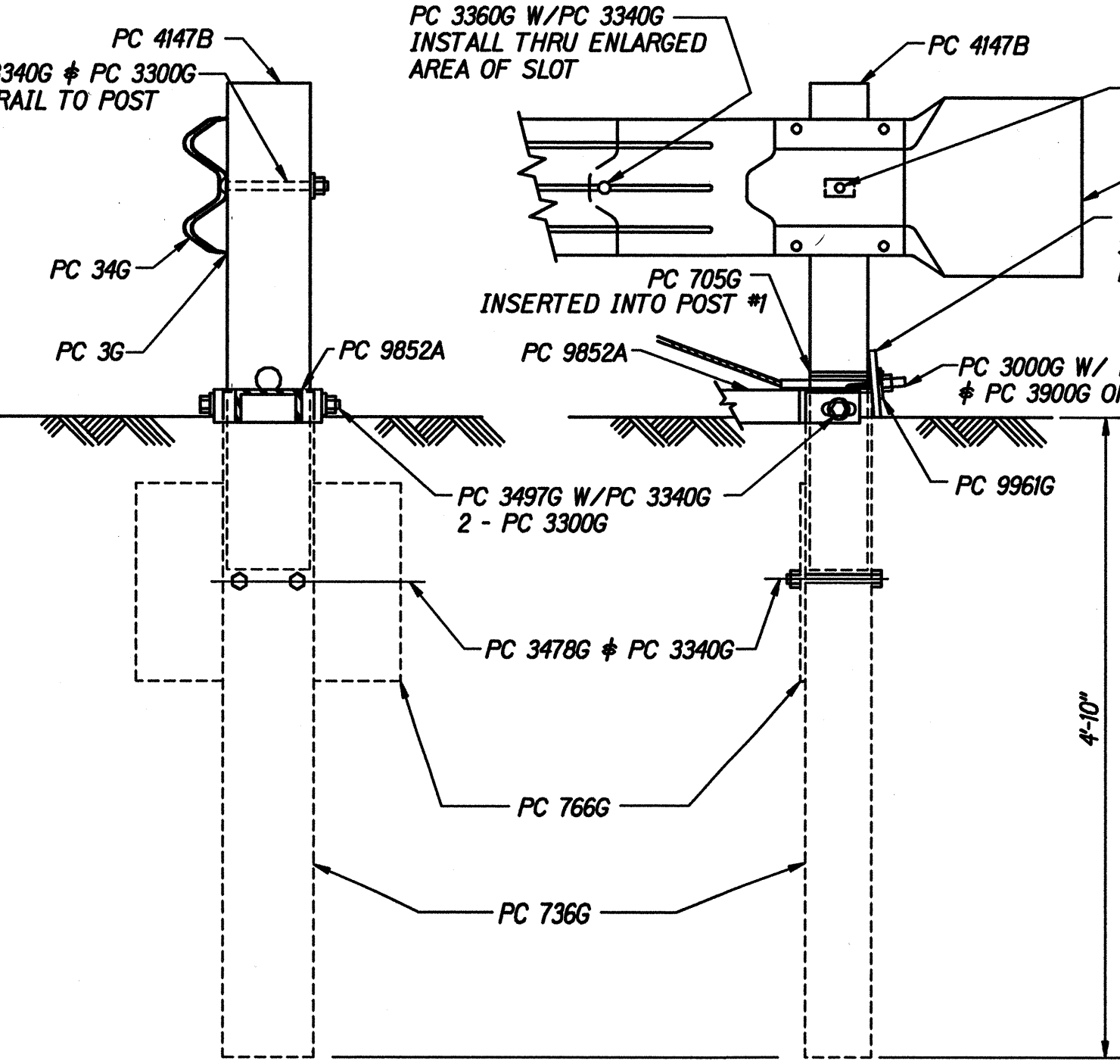
SECTION "A-A" (@ POST #2)
