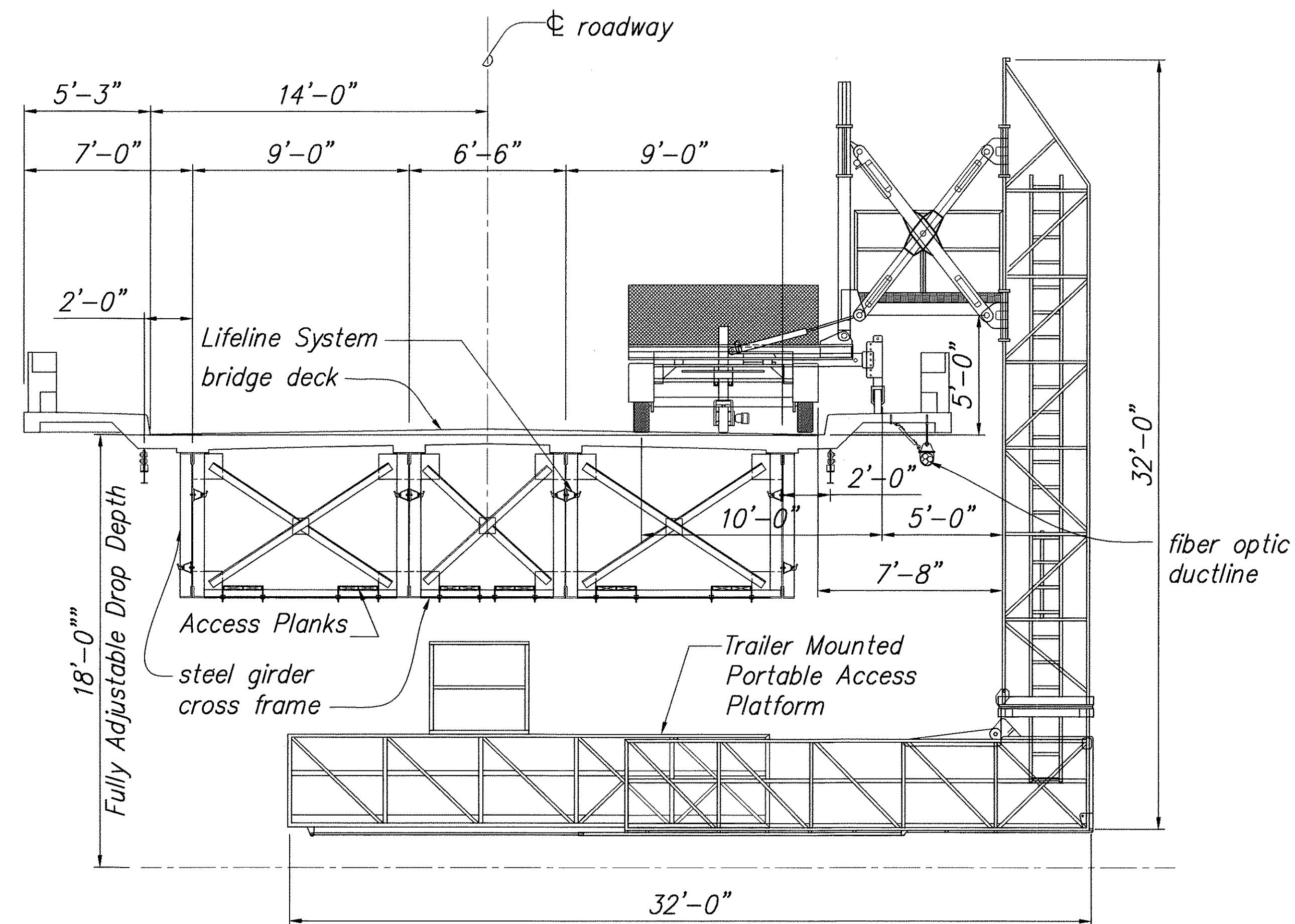
SECTION WITH PORTABLE ACCESS PLATFORM A 13 15 Scale: 1/4" = 1'-0"
