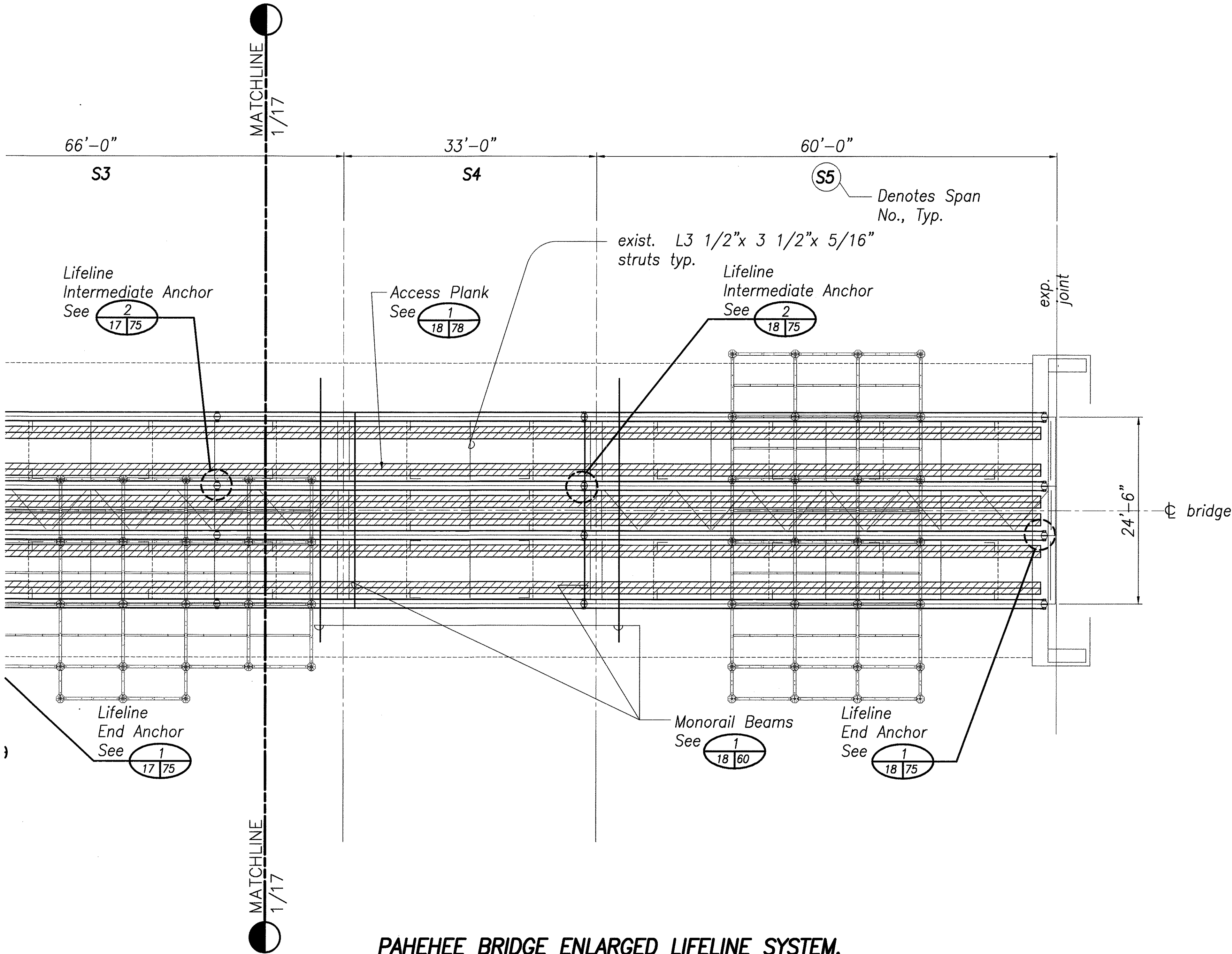
PAHEHEE BRIDGE ENLARGED LIFELINE SYSTEM, PLANKING & ACCESS PLATFORM PLAN
