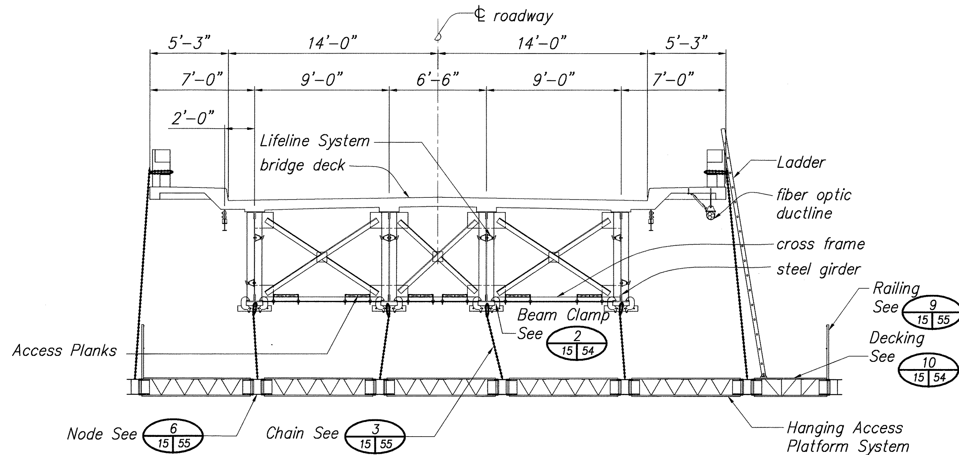
SECTION WITH HANGING ACCESS PLATFORM CONFIGURATION No. 2 C 13 19 15 Scale: 1/4" = 1'-0"
