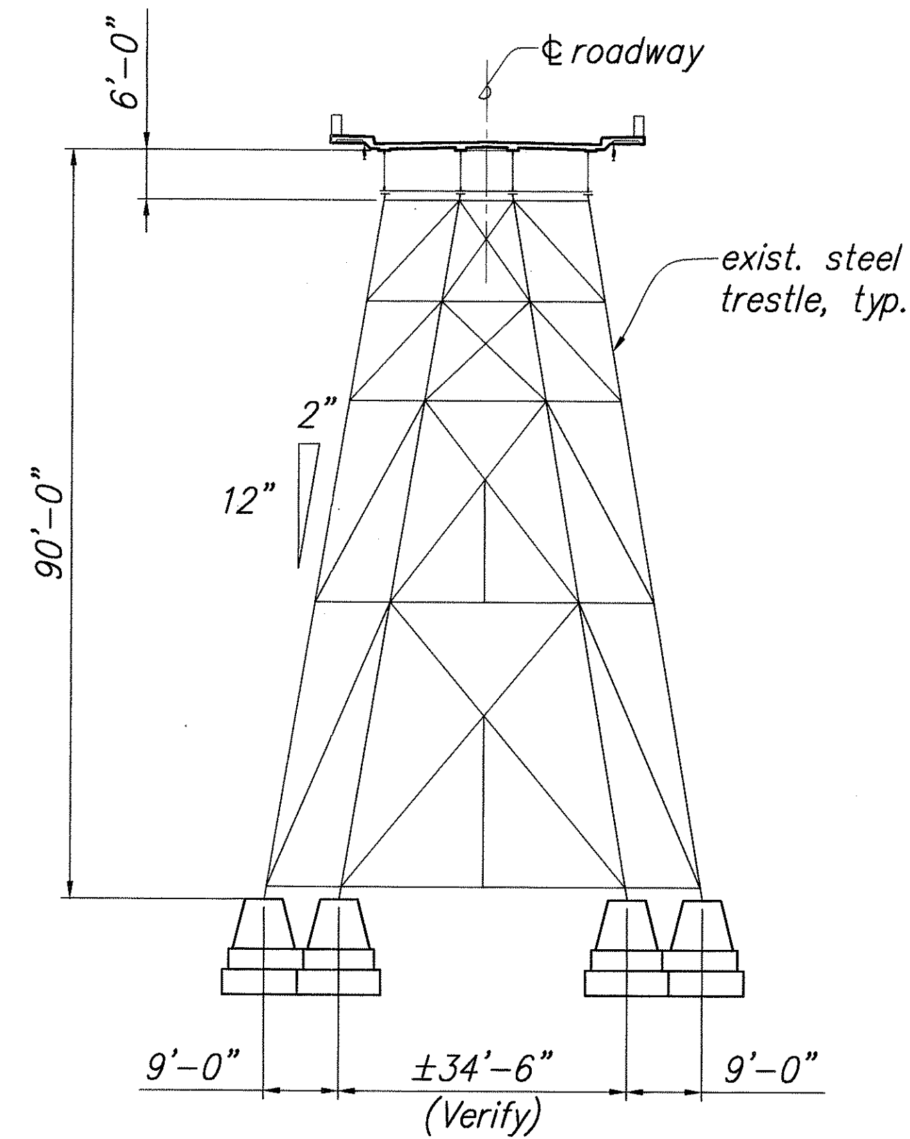
SECTION AT BENT No. 2 B 13 14 Scale: 1/16" = 1'-0"
