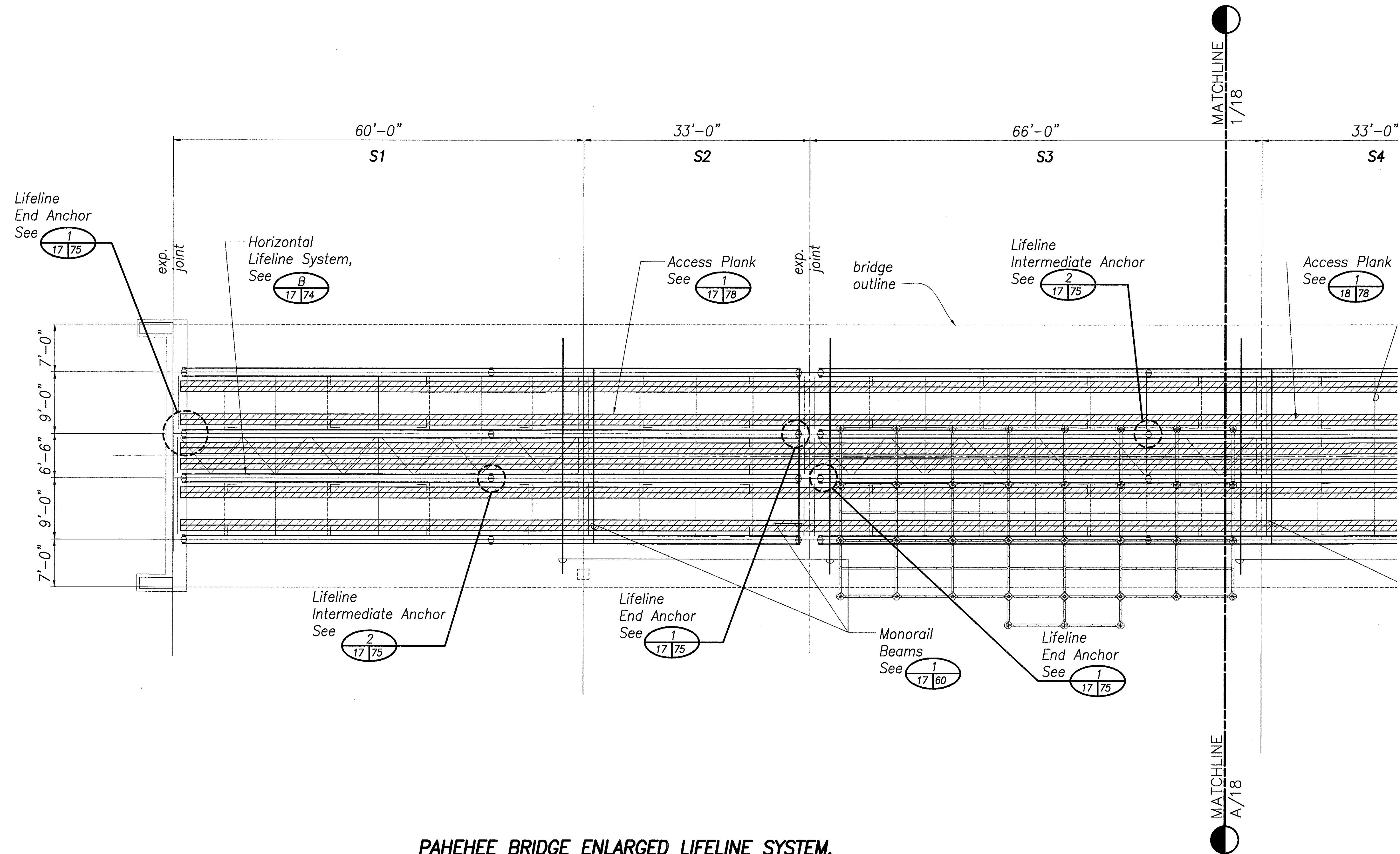
PAHEHEE BRIDGE ENLARGED LIFELINE SYSTEM, PLANKING & ACCESS PLATFORM PLAN
