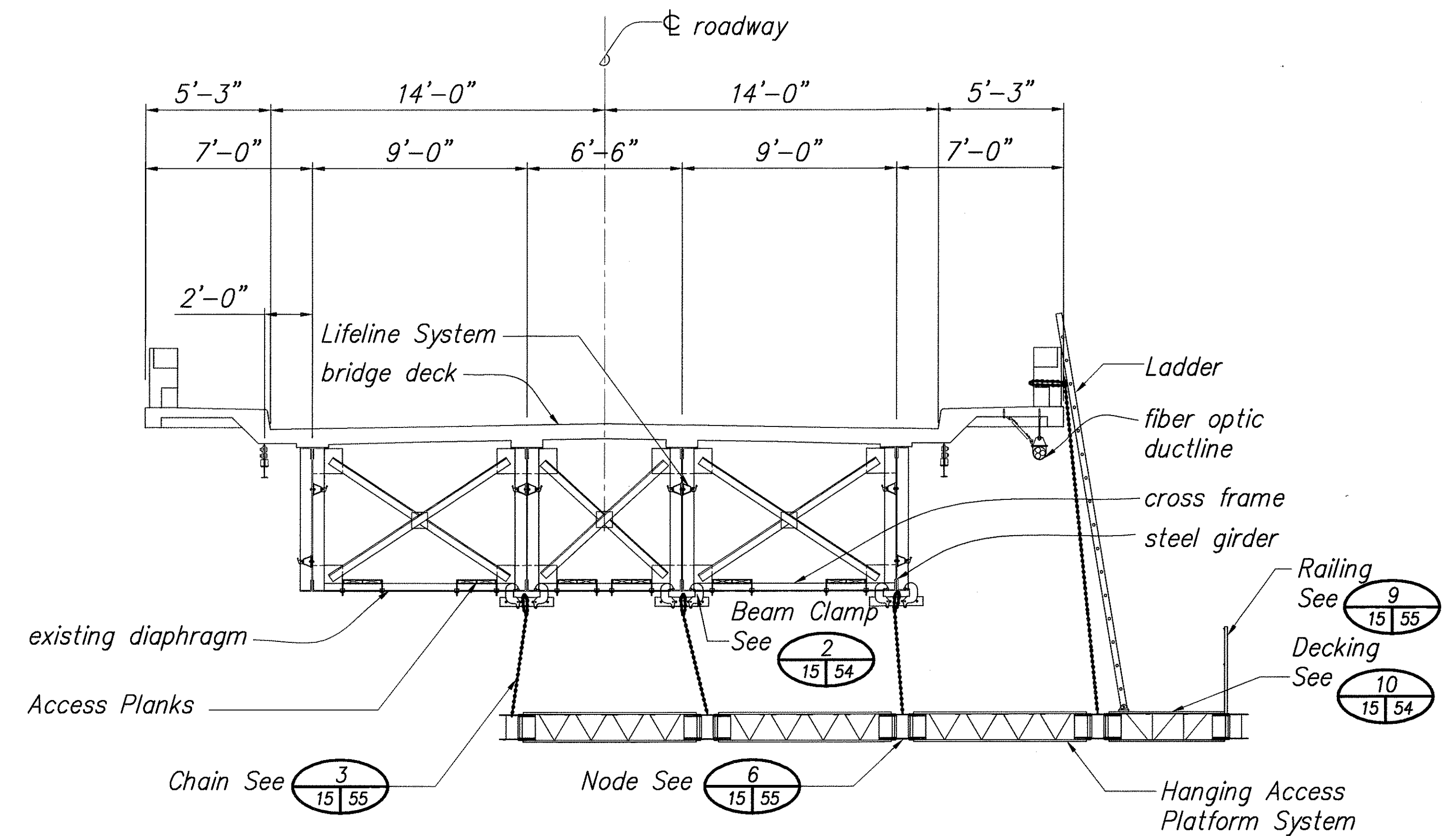
SECTION WITH HANGING ACCESS PLATFORM CONFIGURATION No. 1 B 13 19 15 Scale: 1/4" = 1'-0"
