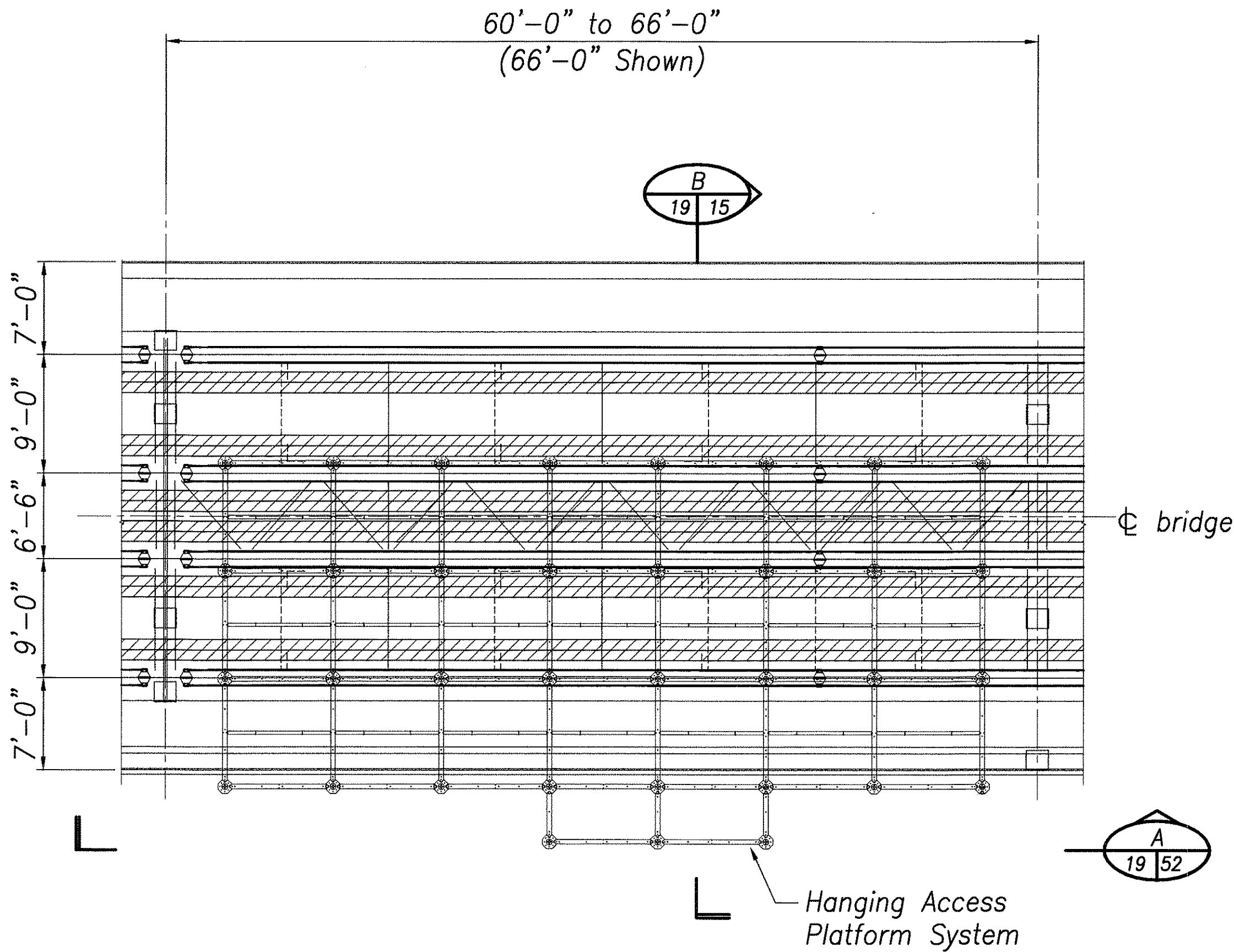
HANGING ACCESS PLATFORM PLANS CONFIGURATION No. 1 Scale: 1/8" = 1'-0"
