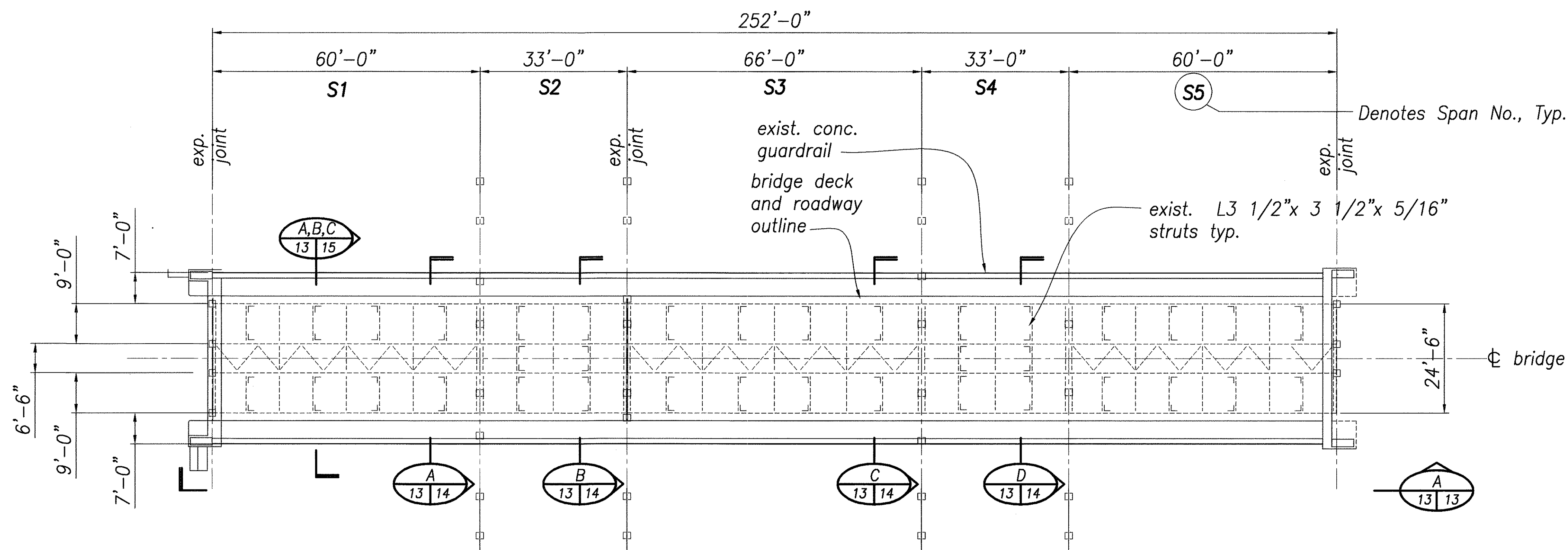
PLAN - PAHEEHĒ BRIDGE Scale: 1/16" = 1'-0" 1 13 13
