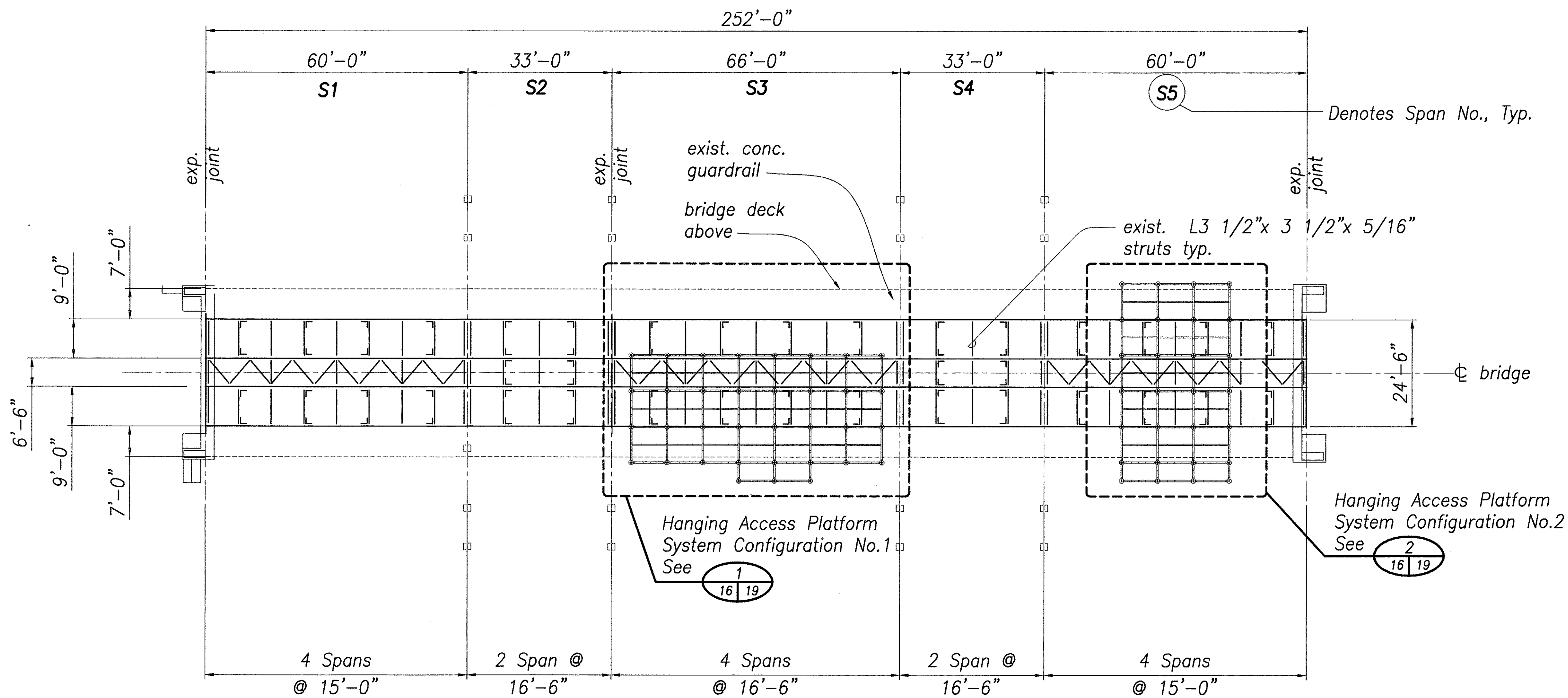
PAHEEHEE BRIDGE GIRDER PLAN 1/16 16 Scale: 1/16" = 1'-0"
