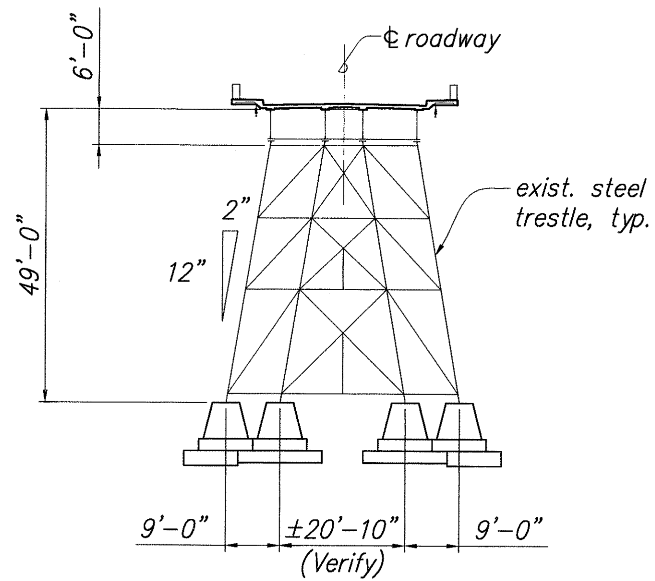
SECTION AT BENT No. 4 D 13 14 Scale: 1/16" = 1'-0"
