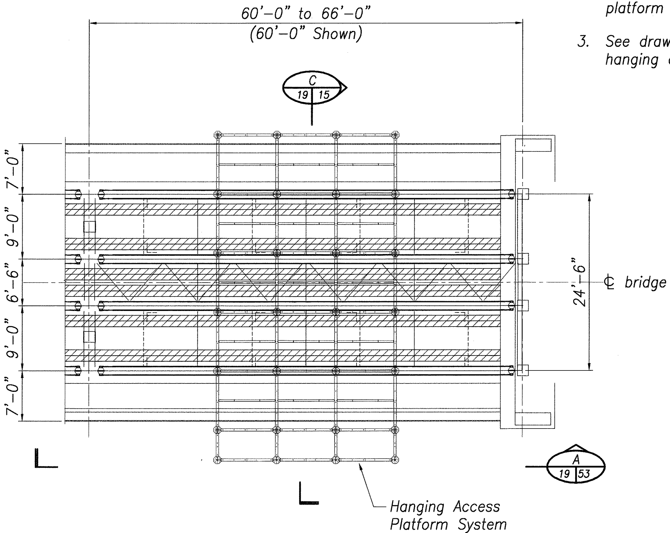
HANGING ACCESS PLATFORM PLANS CONFIGURATION No. 2 Scale: 1/8" = 1'-0"
