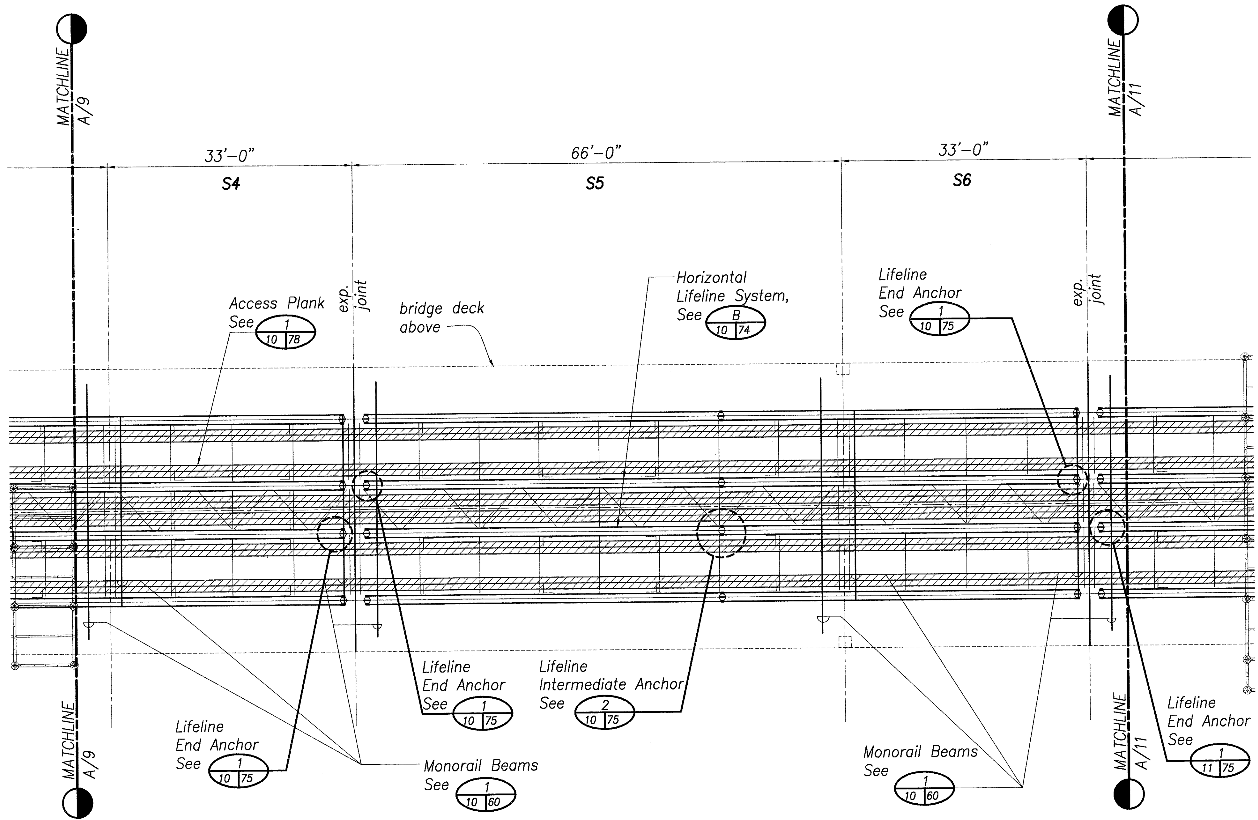
KAPUE BRIDGE ENLARGED LIFELINE SYSTEM, PLANKING & ACCESS PLATFORM PLAN Scale: 1/8" = 1'-0"
