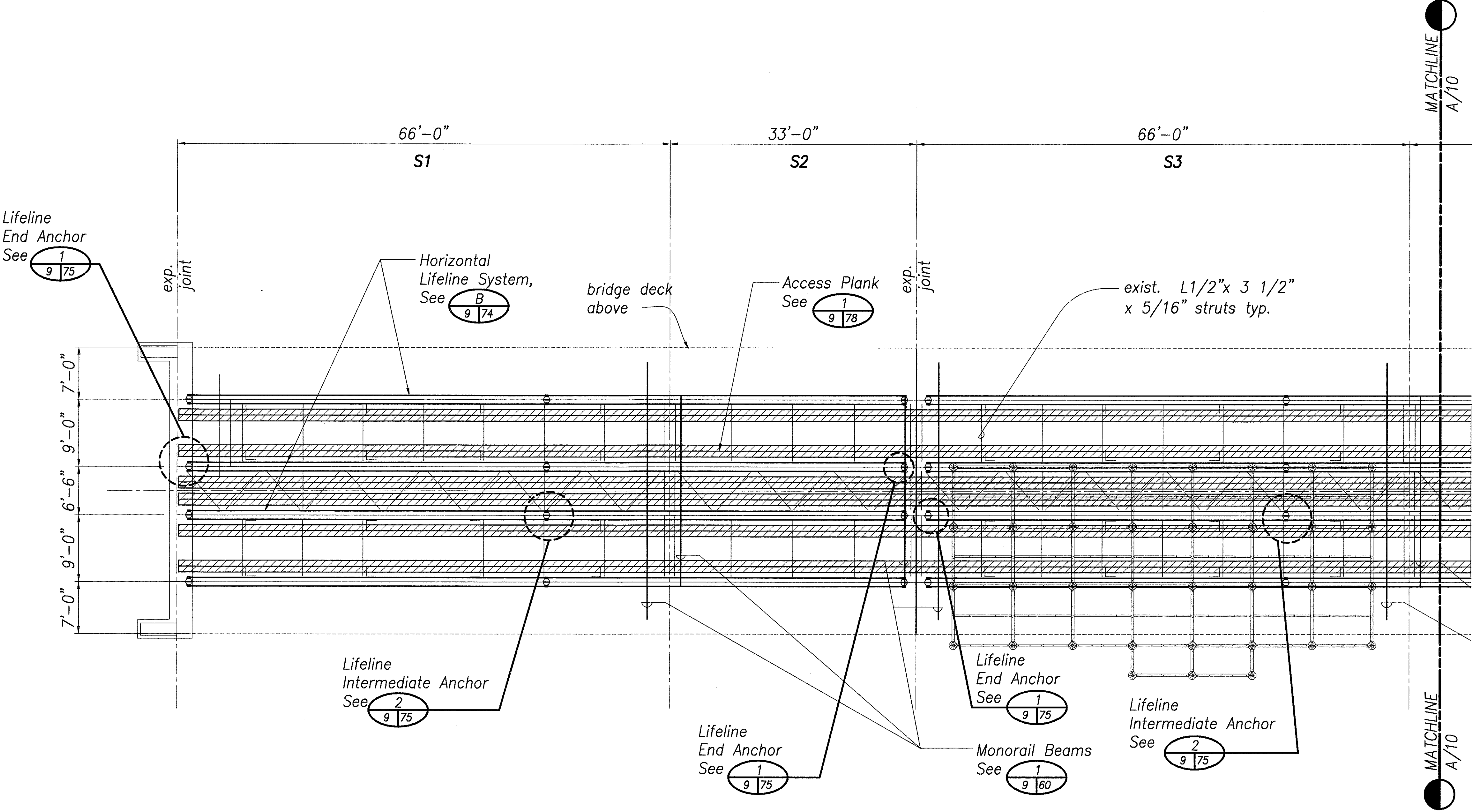
KAPUE BRIDGE ENLARGED LIFELINE SYSTEM, PLANKING & ACCESS PLATFORM PLAN Scale: 1/8" = 1'-0" 1 9 | 9
