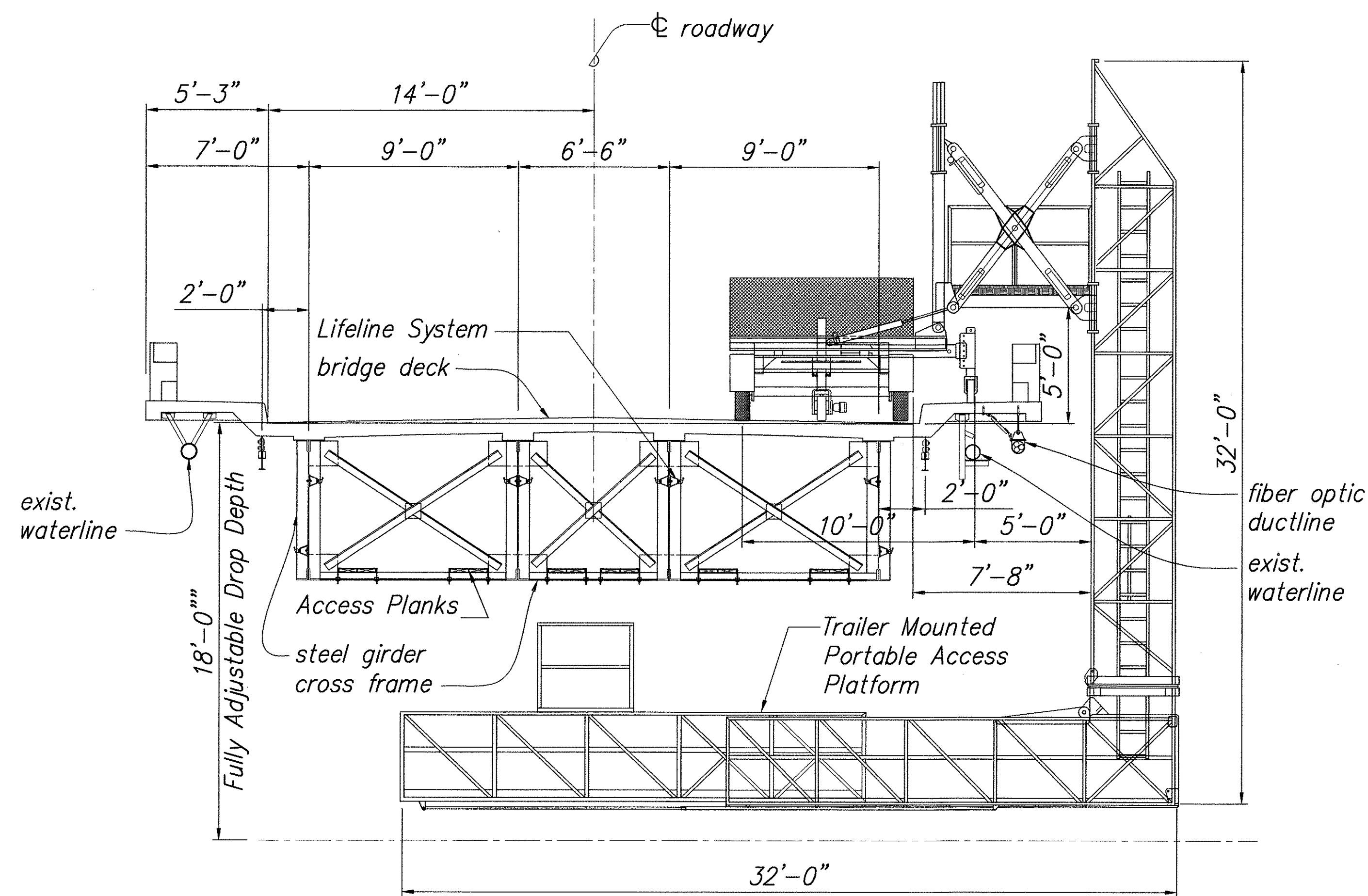
SECTION WITH PORTABLE ACCESS PLATFORM Scale: 1/4" = 1'-0" A 5 7
