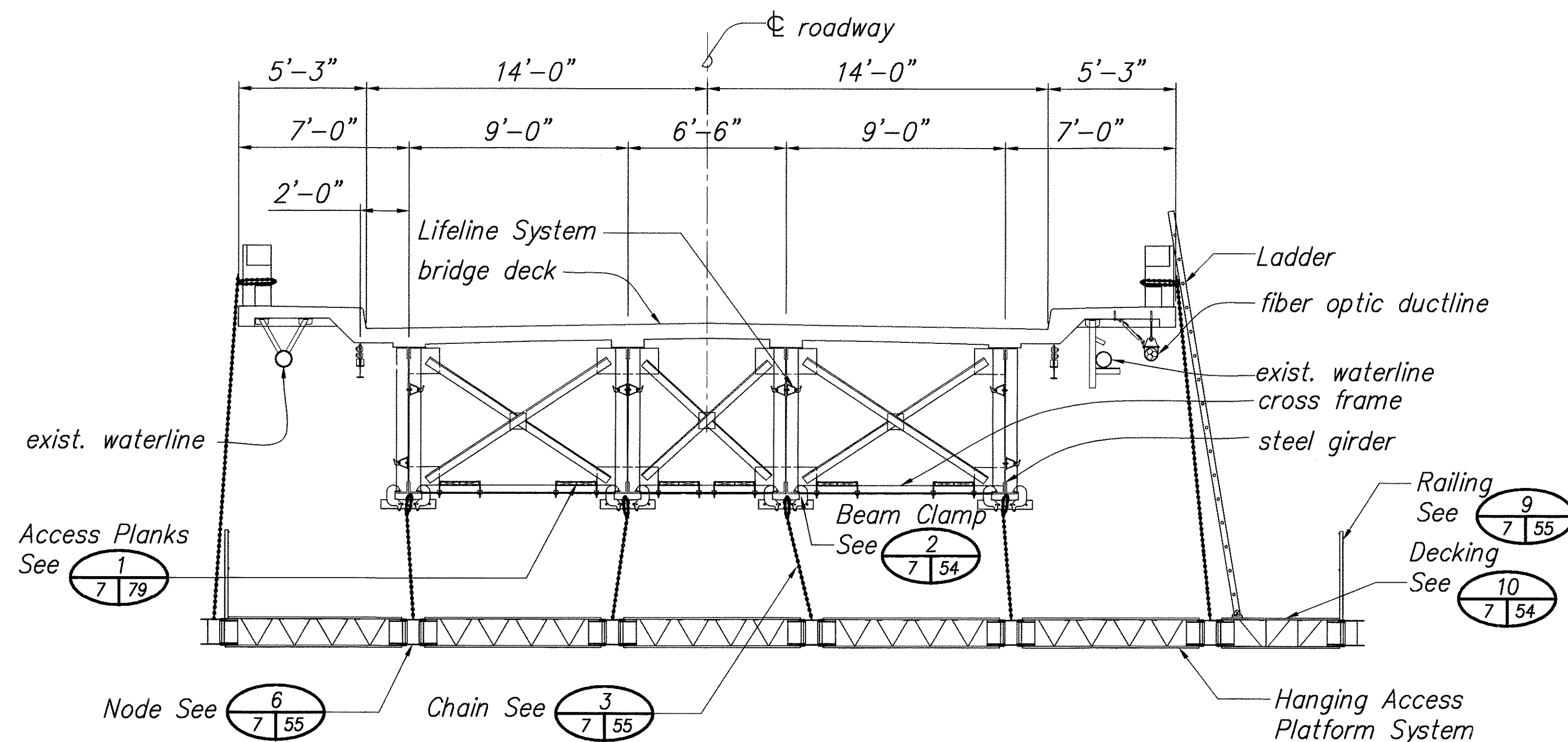
SECTION WITH PORTABLE ACCESS PLATFORM Scale: 1/4" = 1'-0" A 5 7
