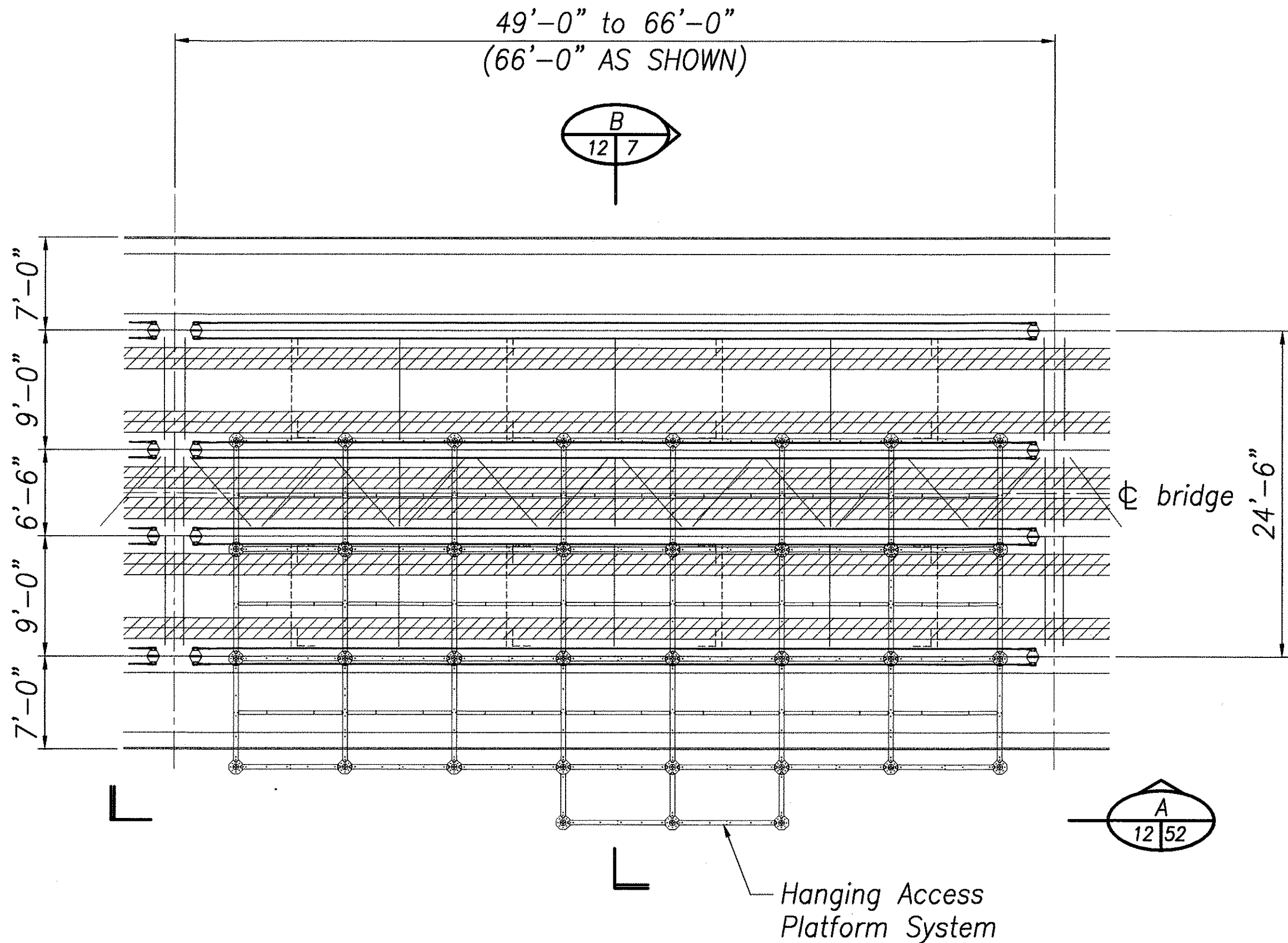
HANGING ACCESS PLATFORM PLAN CONFIGURATION No. 1 Scale: 1/8" = 1'-0"
