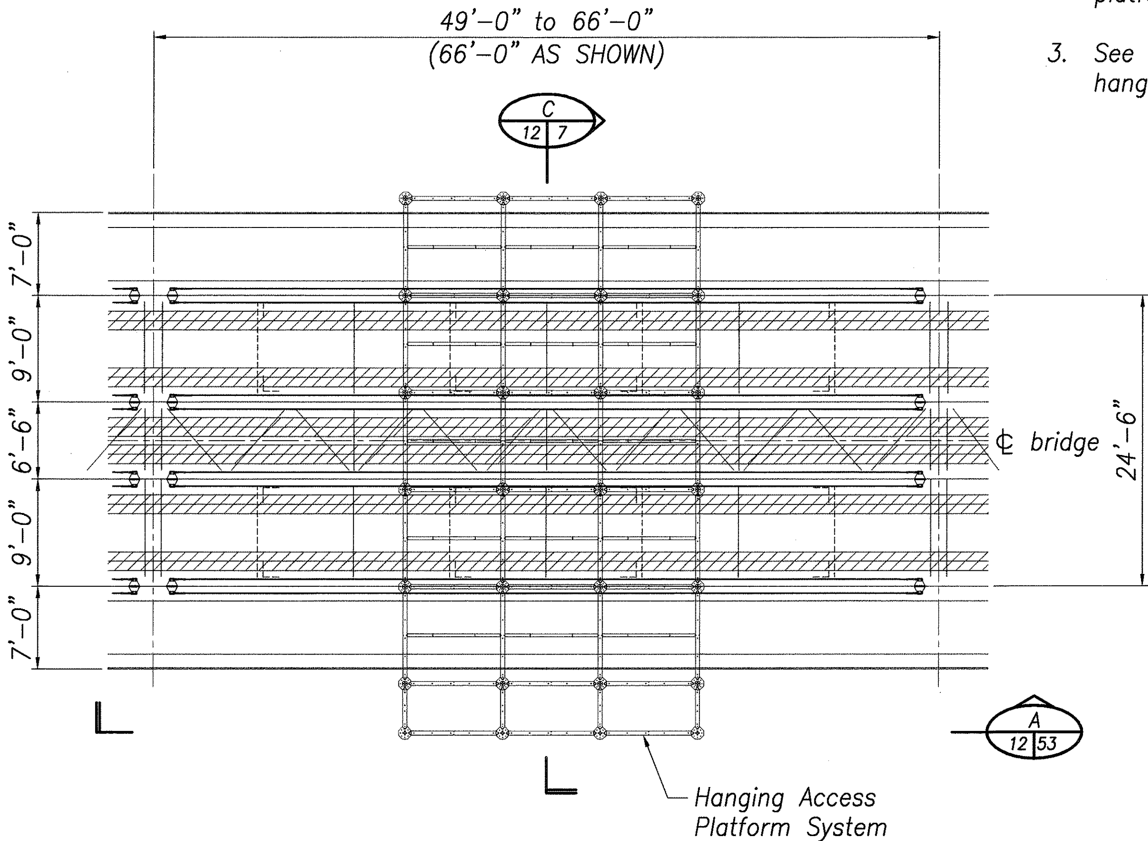
HANGING ACCESS PLATFORM PLAN CONFIGURATION No. 2 Scale: 1/8" = 1'-0"
