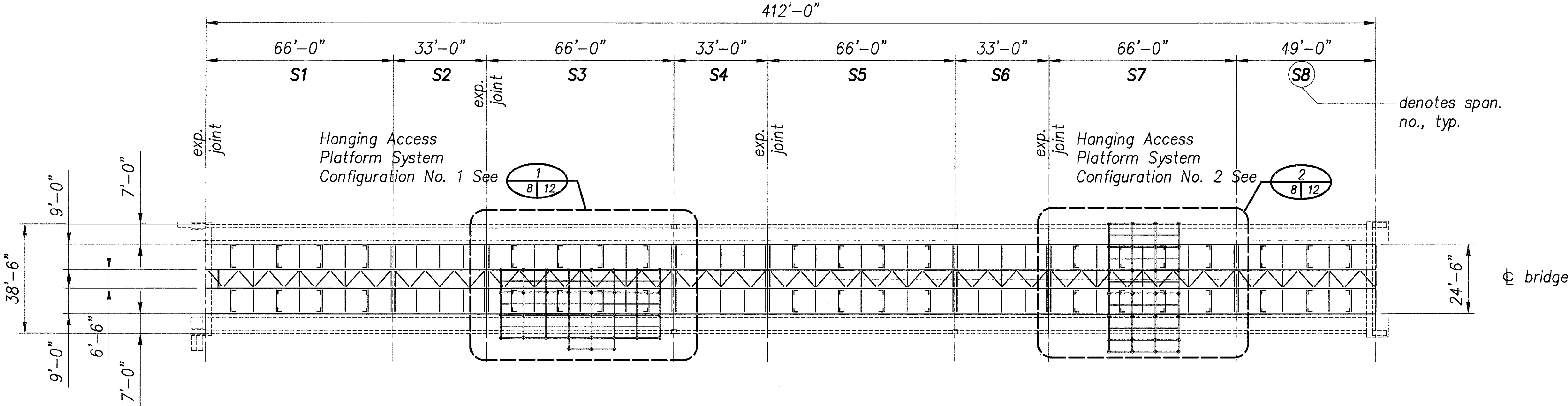
KAPUE BRIDGE GIRDER PLAN Scale: 3/64" = 1'-0" 1/8 8
