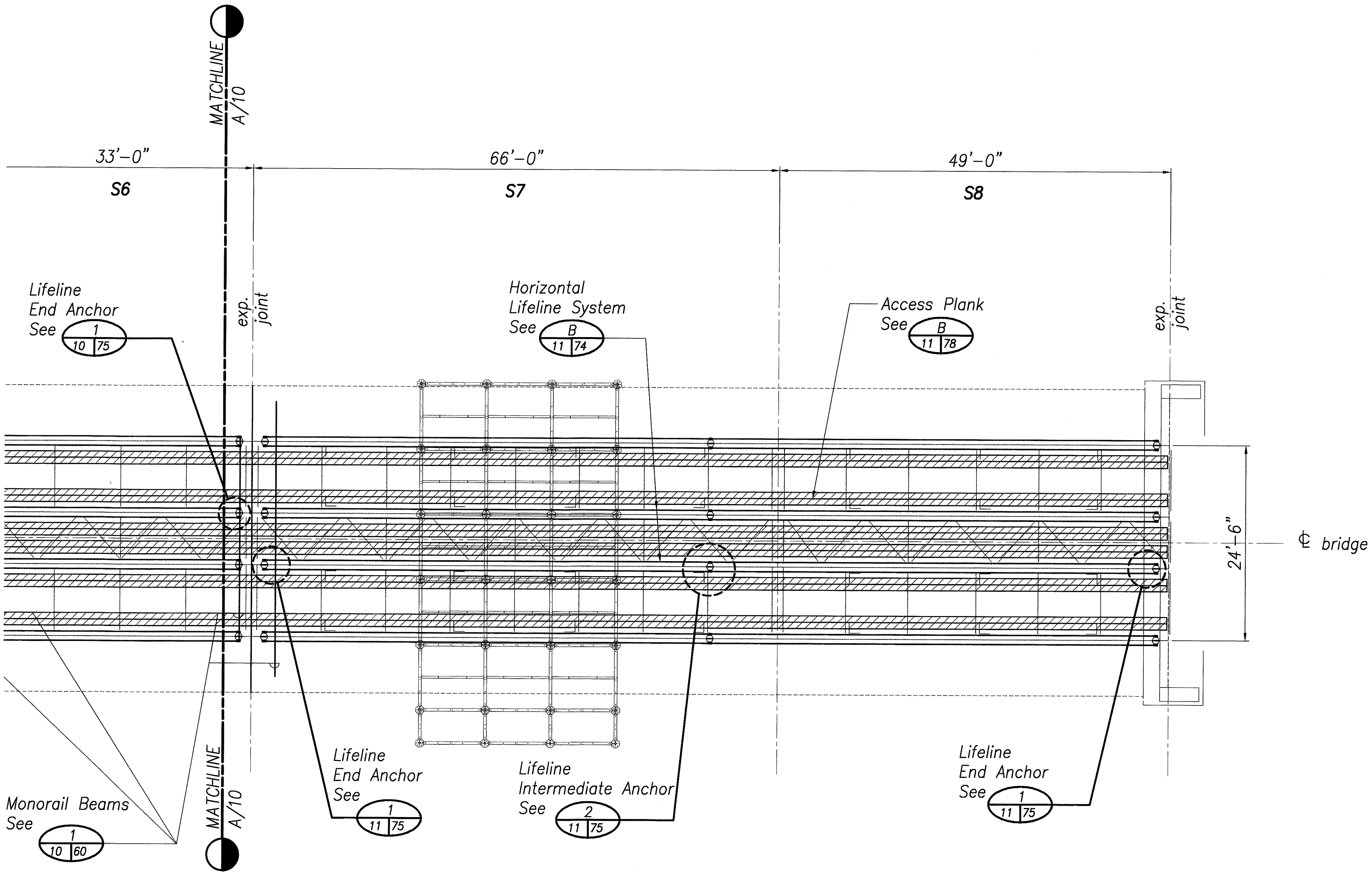
KAPUE BRIDGE ENLARGED LIFELINE SYSTEM, PLANKING & ACCESS PLATFORM PLAN Scale: 1/8" = 1'-0" 1 11 11
