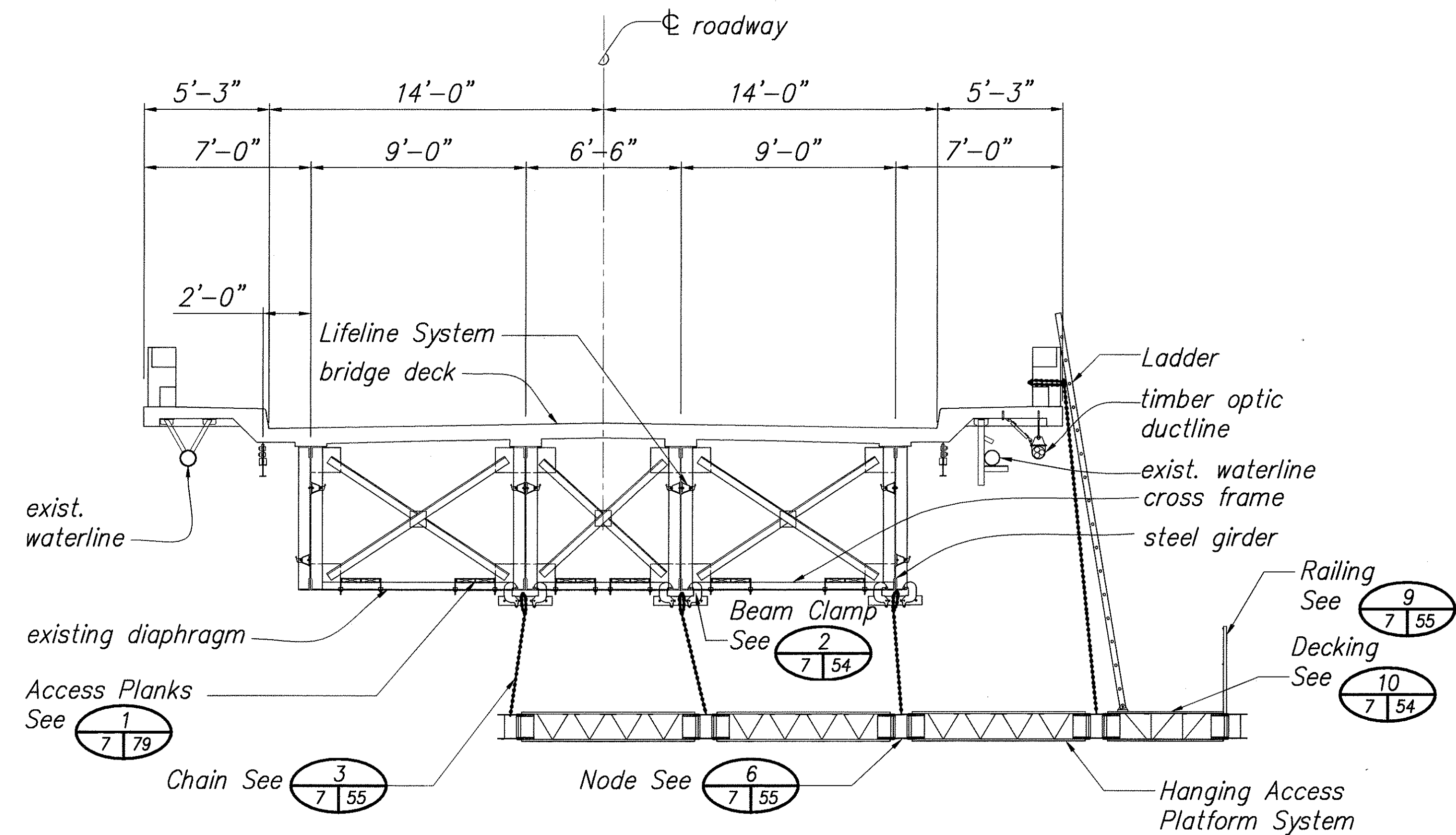
SECTION WITH HANGING ACCESS PLATFORM CONFIGURATION No. 1 Scale: 1/4" = 1'-0" B 5 7
