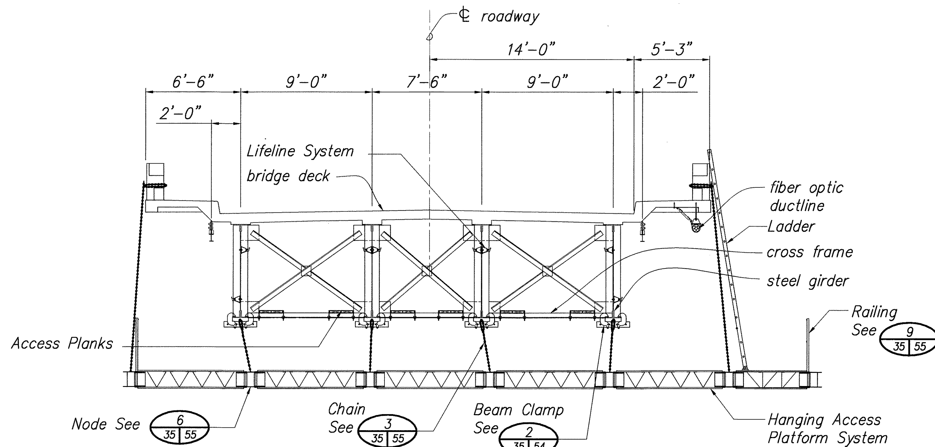
SECTION WITH HANGING ACCESS PLATFORM CONFIGURATION No. 2 Scale: 1/4" = 1'-0"
