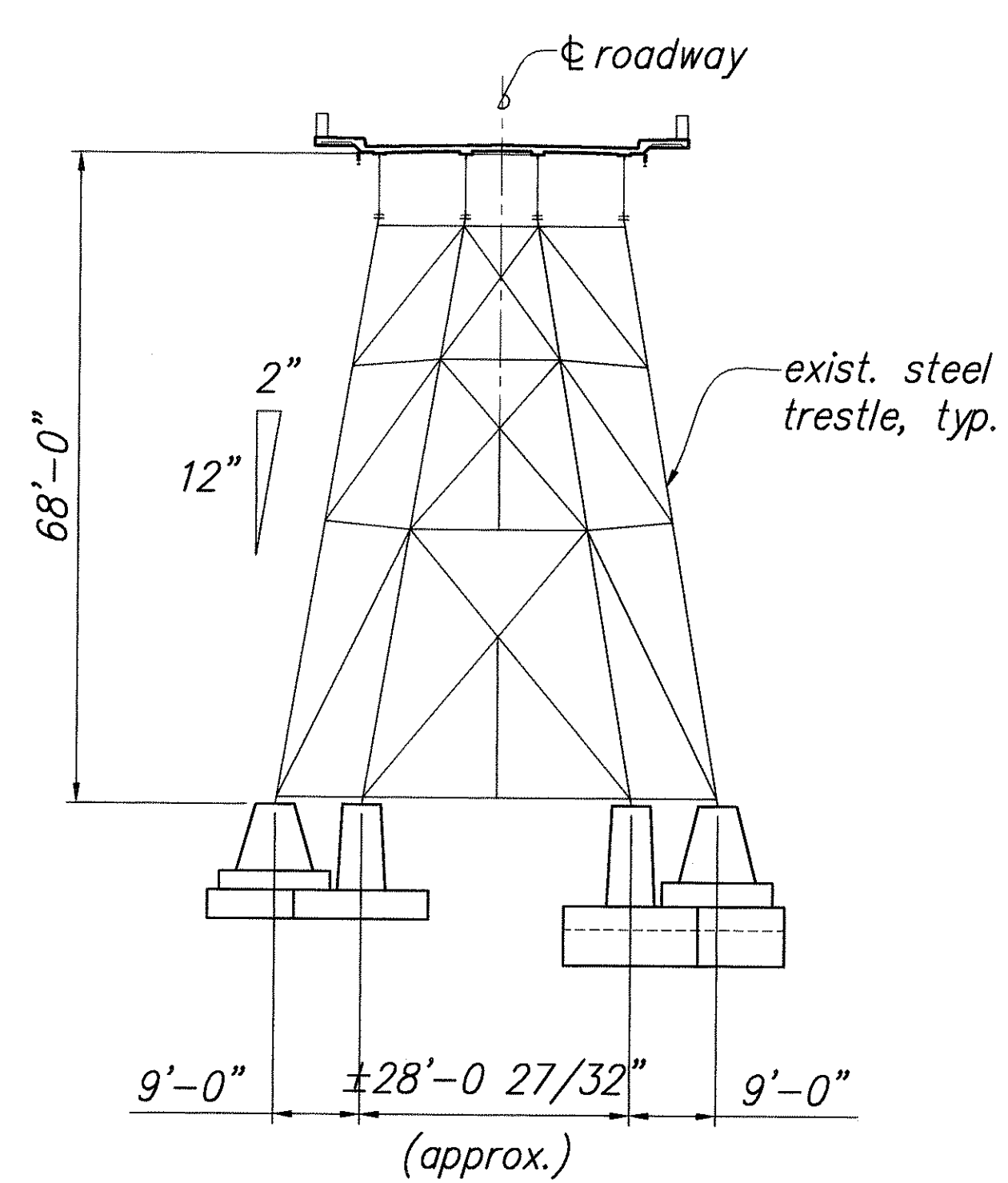
SECTION AT BENT No. 12 C 32 | 34 Scale: 1/16" = 1'-0"
