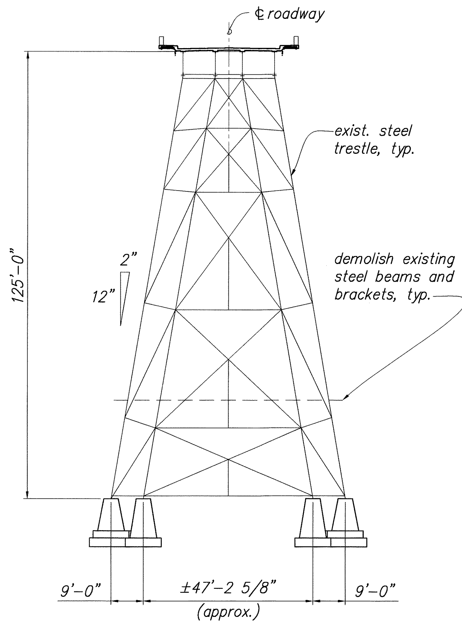
SECTION AT BENT No. 2 B 32 | 33 Scale: 1/16" = 1'-0"
