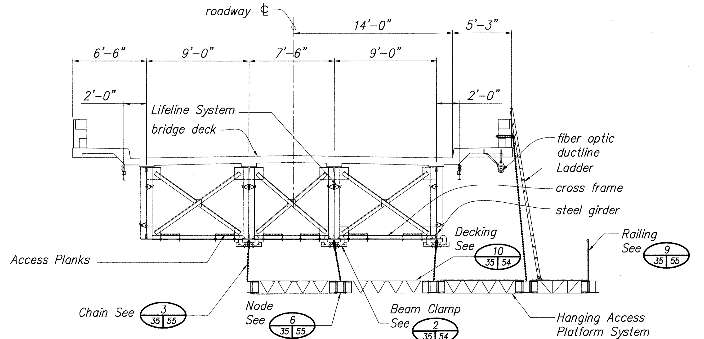
SECTION WITH HANGING ACCESS PLATFORM CONFIGURATION No. 1 Scale: 1/4" = 1'-0"
