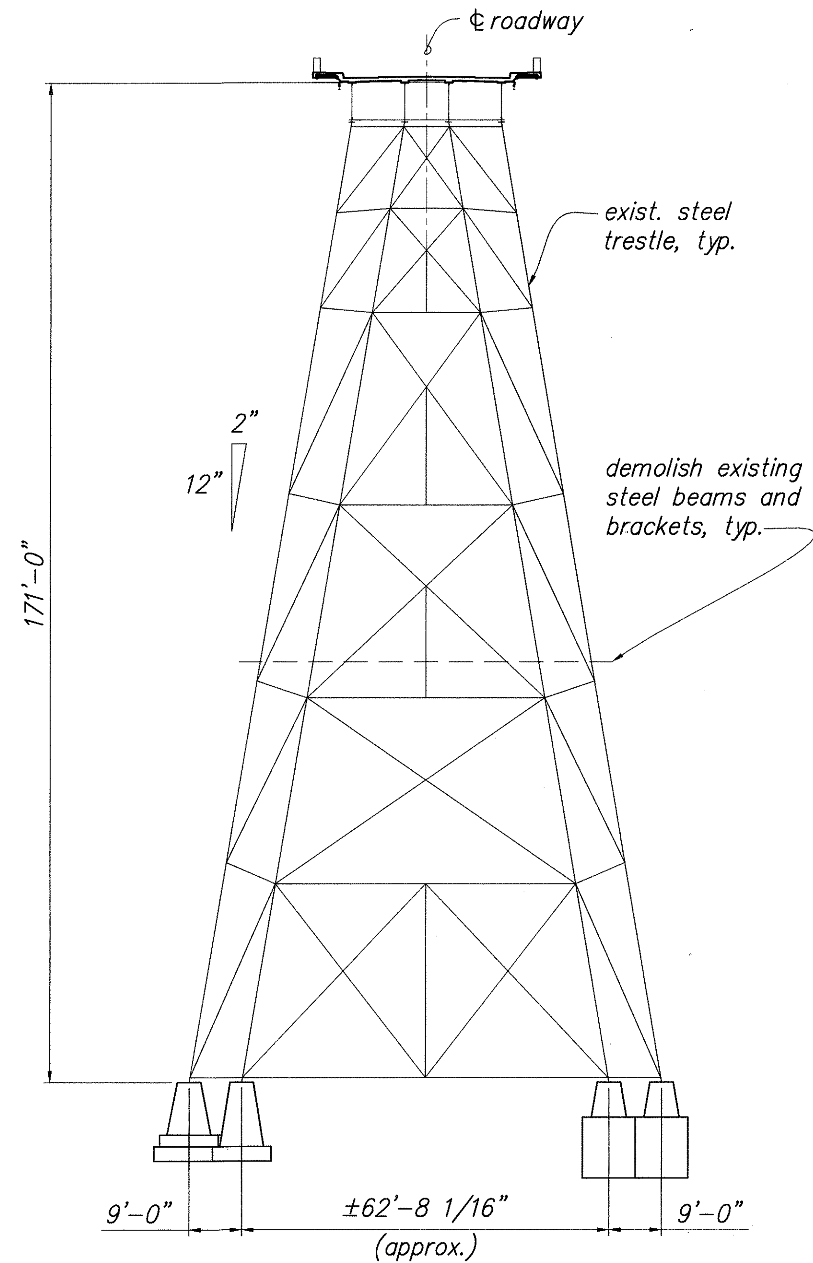
SECTION AT BENT No. 4 To 9 D 32 | 33 Scale: 1/16" = 1'-0"
