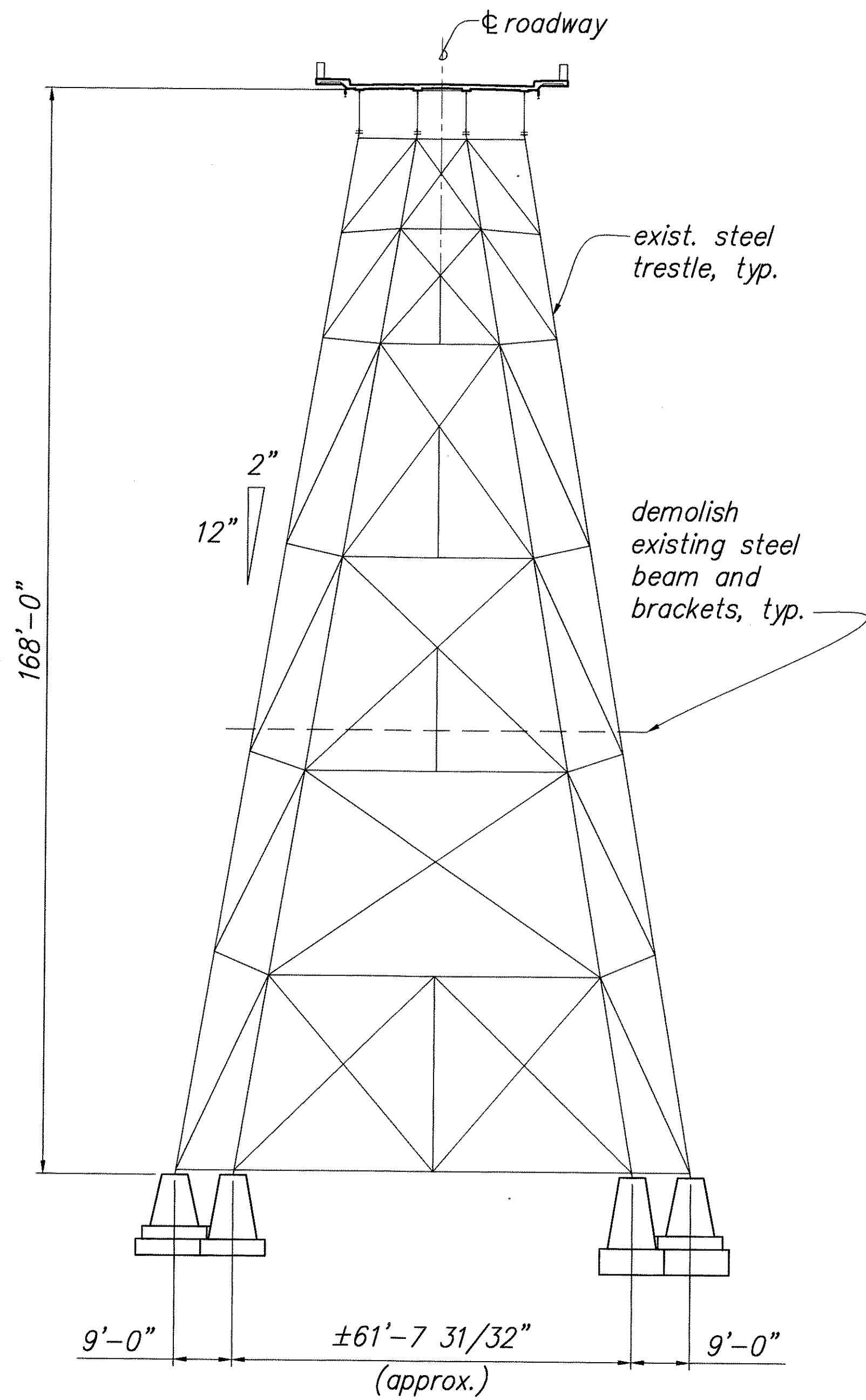
SECTION AT BENT No. 10 A 32 | 34 Scale: 1/16" = 1'-0"
