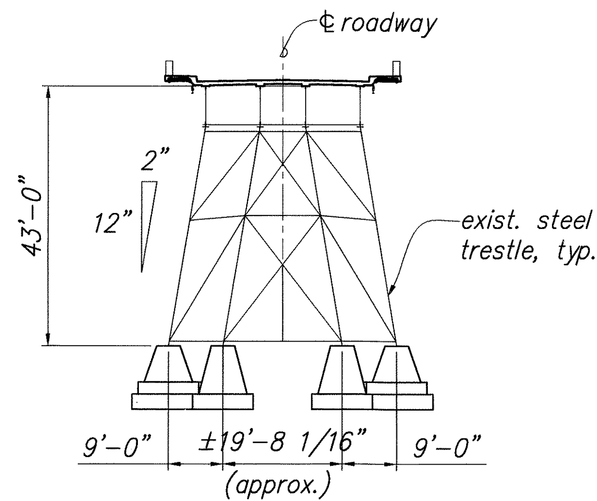
SECTION AT BENT No. 1 A 32 | 33 Scale: 1/16" = 1'-0"
