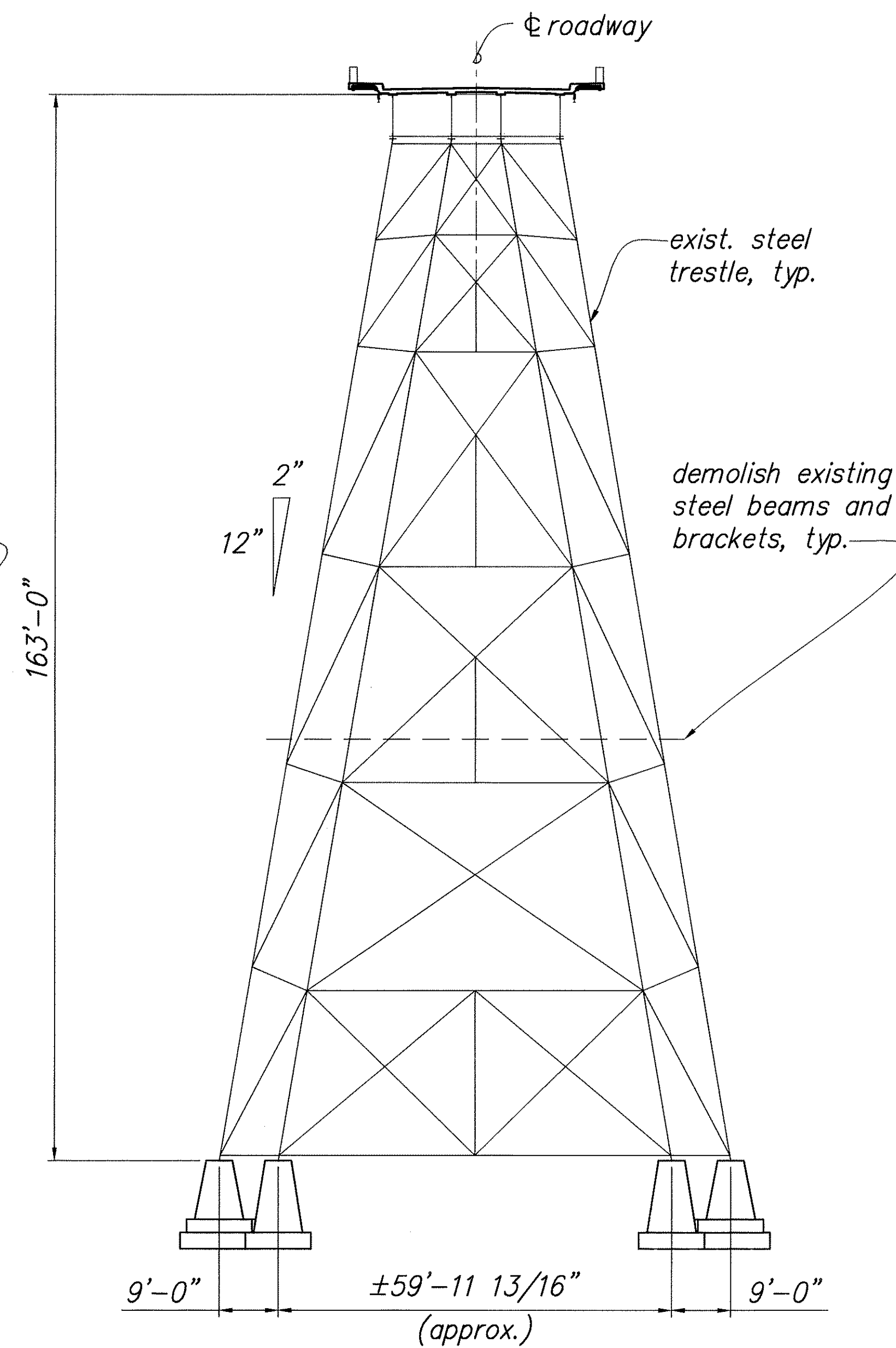
SECTION AT BENT No. 3 C 32 | 33 Scale: 1/16" = 1'-0"
