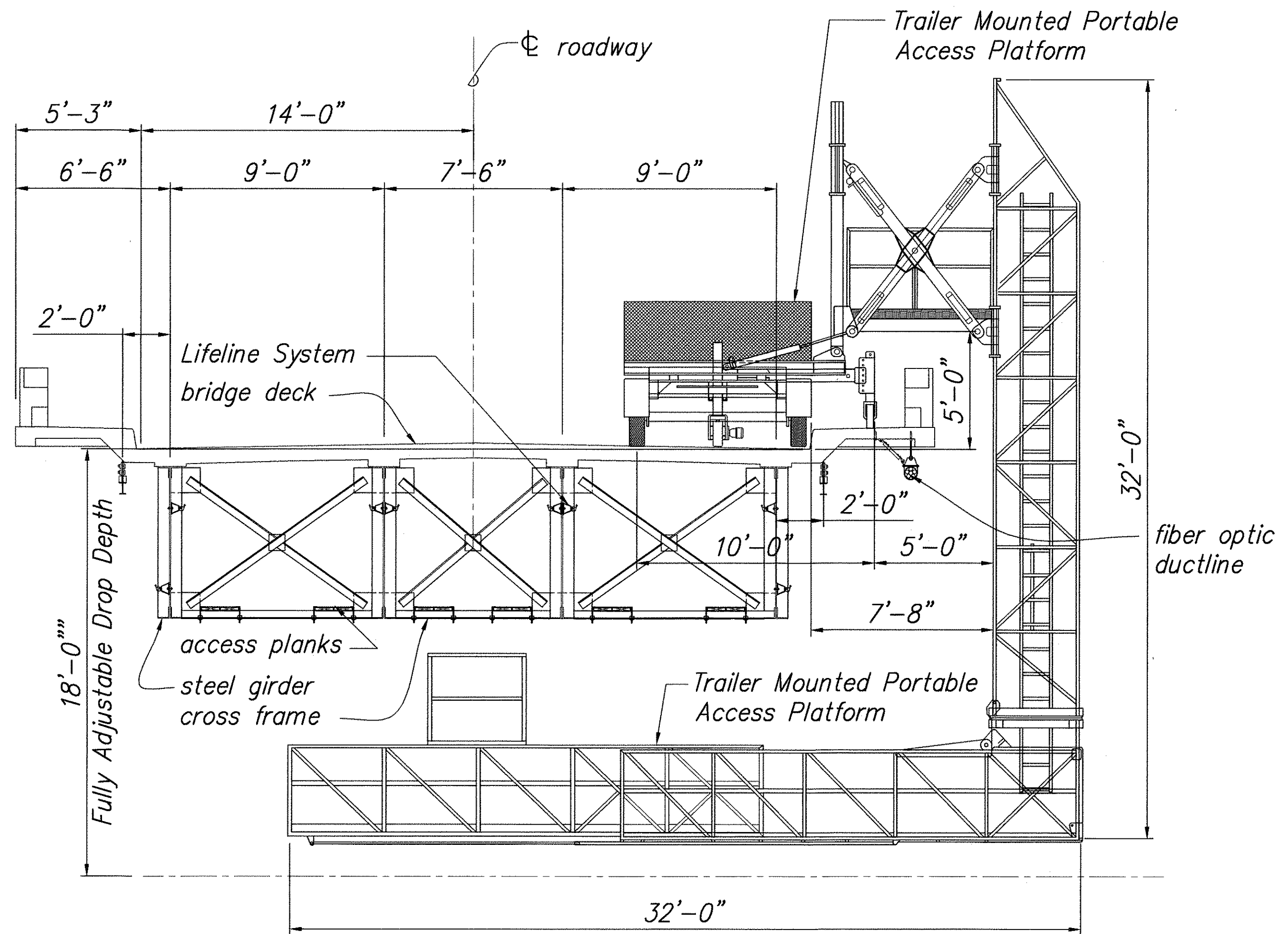
SECTION WITH PORTABLE ACCESS PLATFORM Scale: 1/4" = 1'-0"
