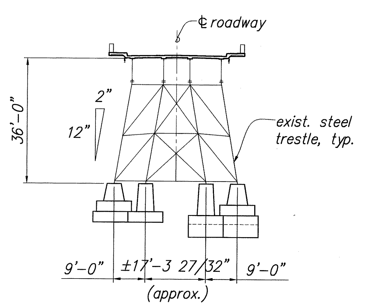
SECTION AT BENT No. 13 D 32 | 34 Scale: 1/16" = 1'-0"
